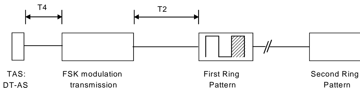
Figure 5: Data transmission prior to ringing - case a) DT-AS
