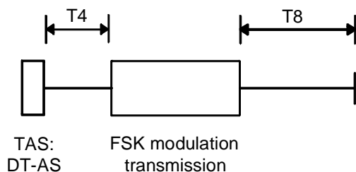
Figure 8: Data transmission not associated with ringing - case a) DT-AS
