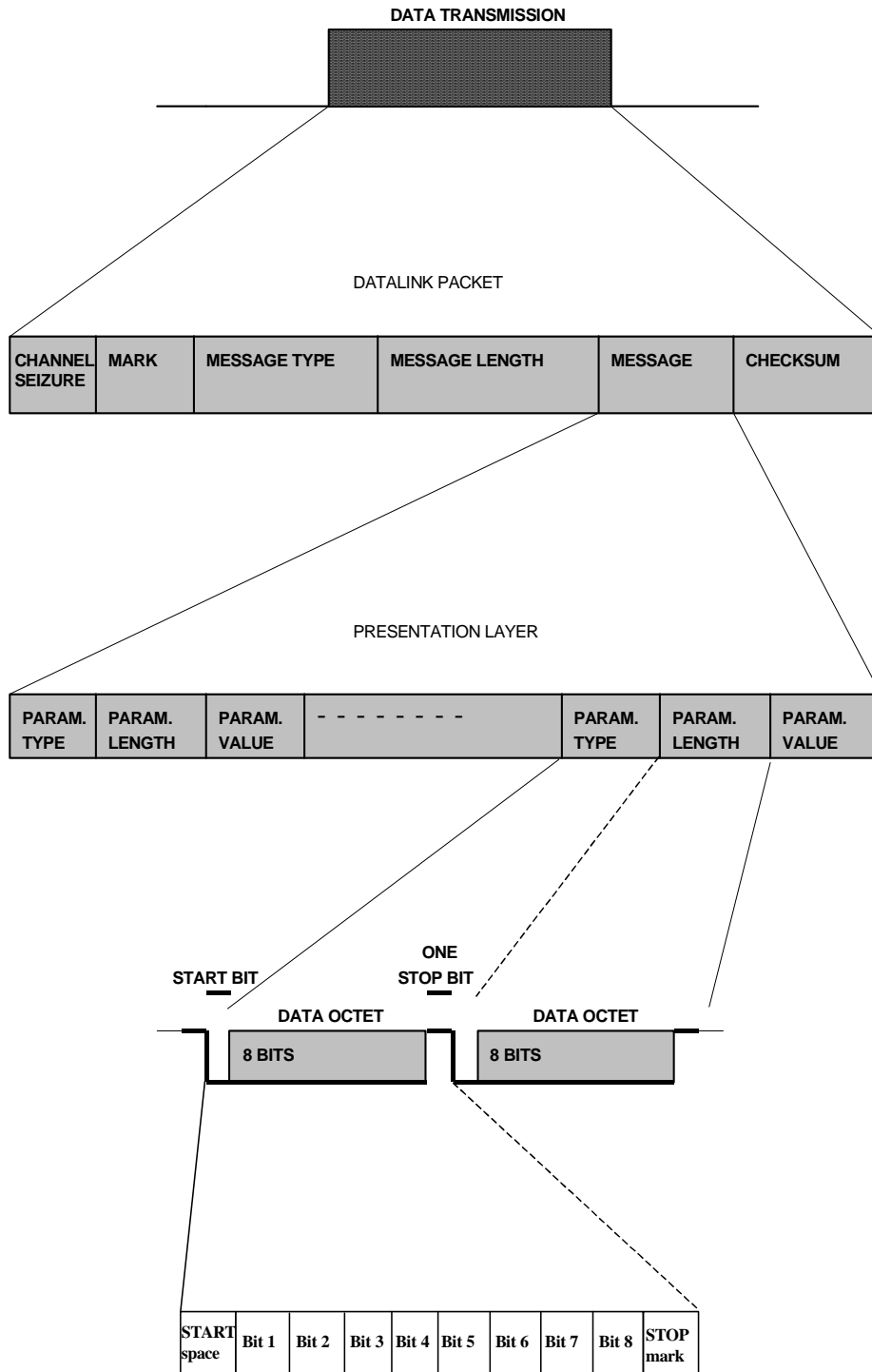
Figure D.1: Format of the data transmission
