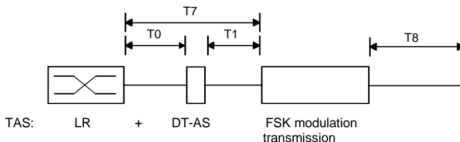
Figure 10: Data transmission not related with ringing - case c) line reversal + DT-AS
