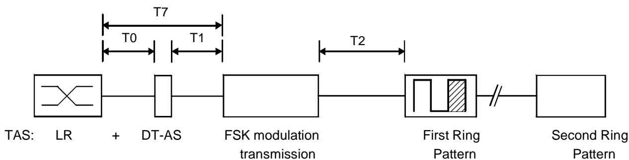
Figure 7: Data transmission prior to ringing - case c) LR+DT-AS
