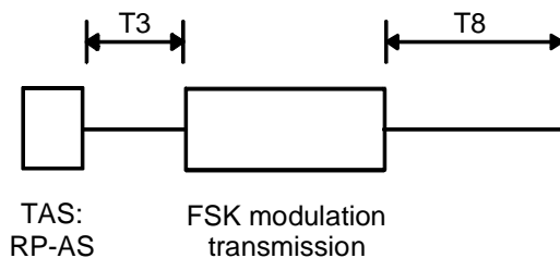
Figure 9: Data transmission not associated with ringing - case b) RP-AS
