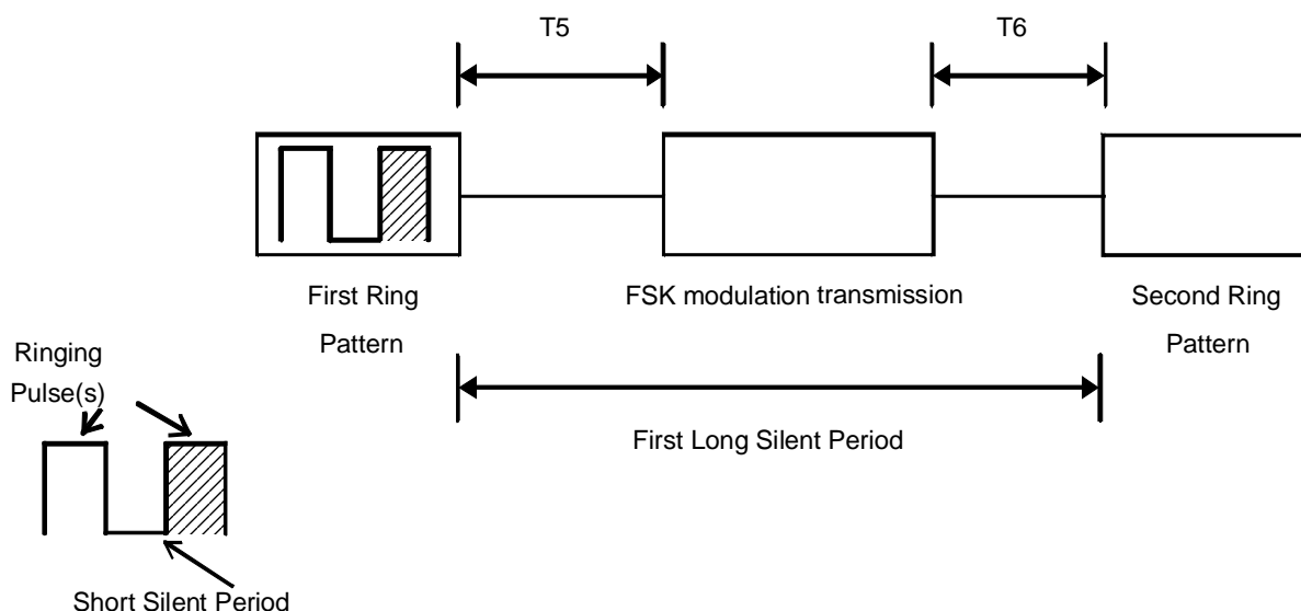
Figure 4: Data transmission during ringing
