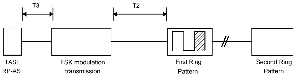
Figure 6: Data transmission prior to ringing - case b) RP-AS
