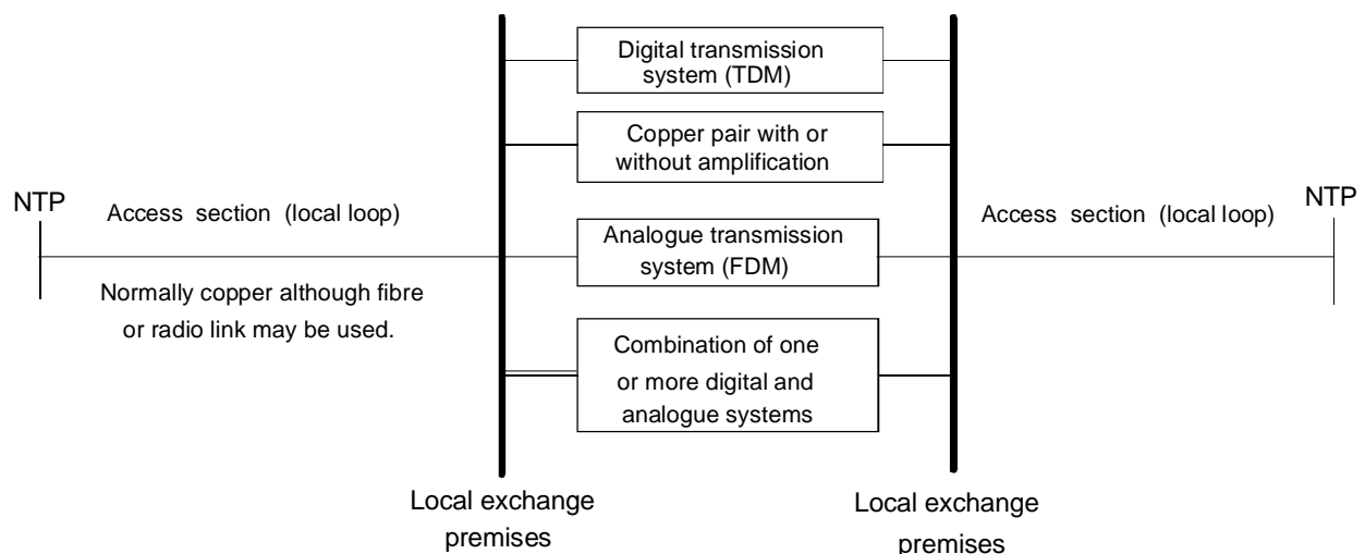
Figure C.1: Means of providing analogue leased lines
