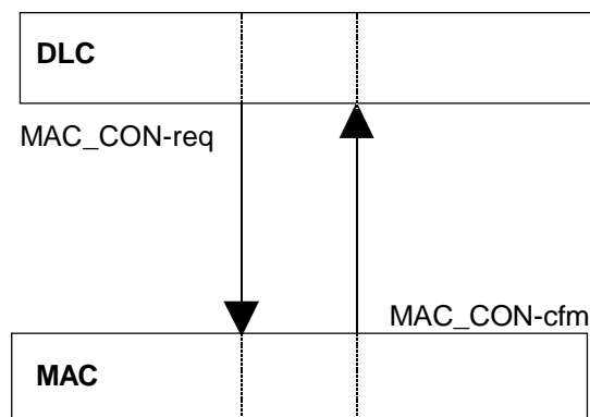
Figure 80: Establishment of a MAC connection initiating side
