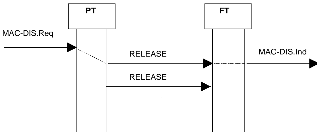
Figure 90: Bearer release
