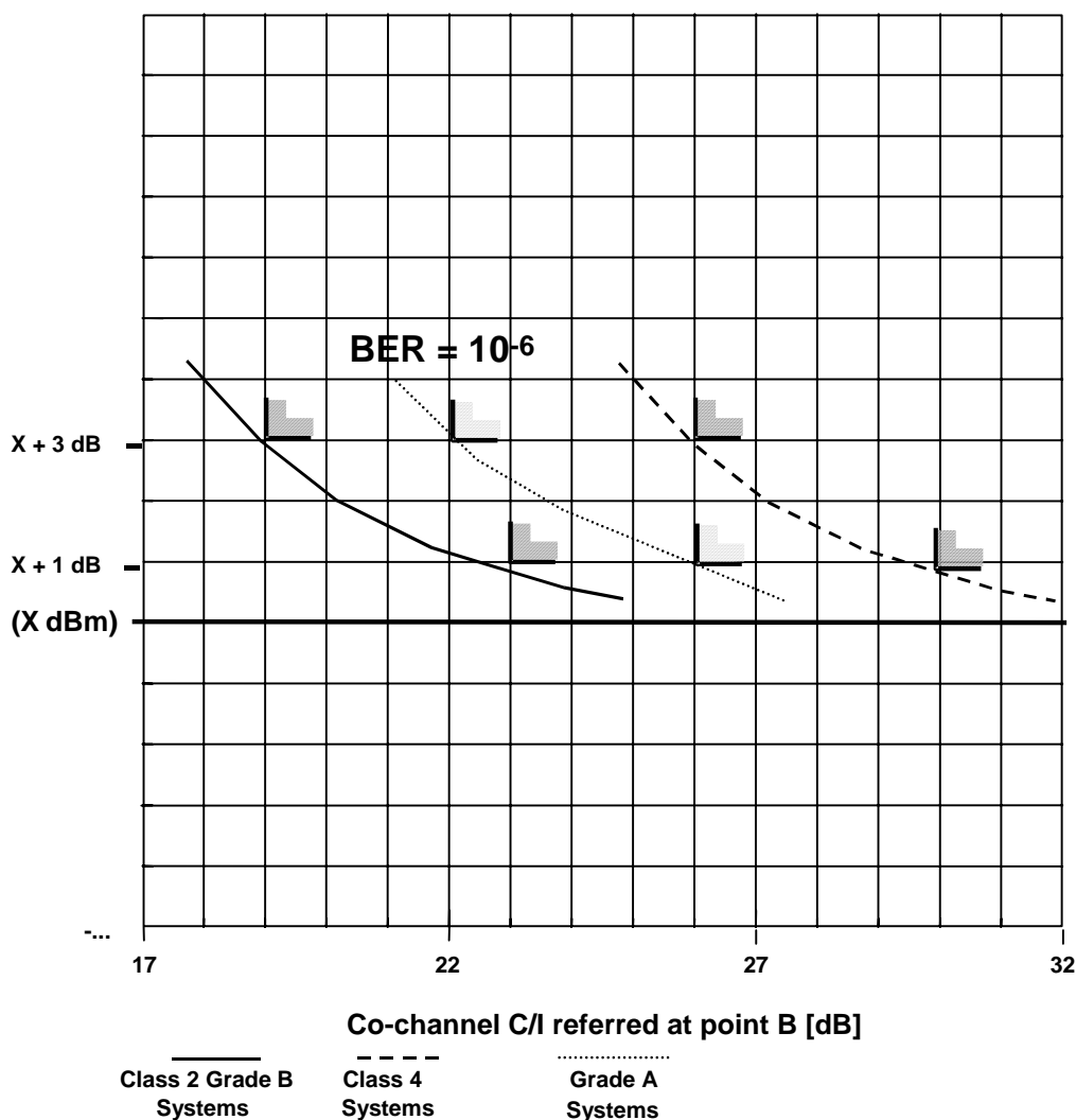
Figure A.2a: Co-channel interference threshold degradation
