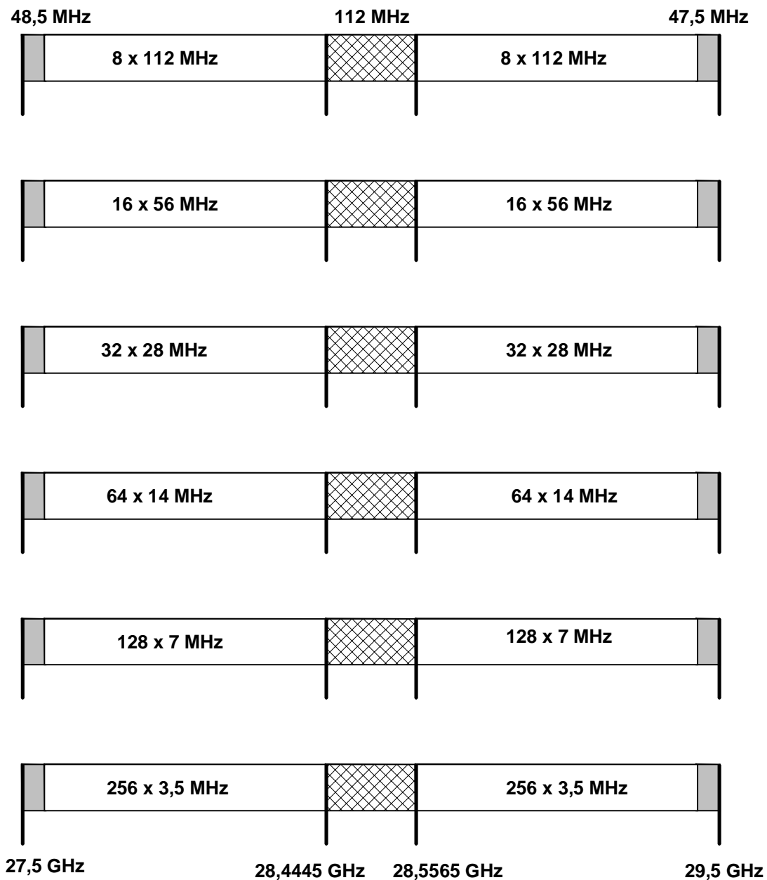
Figure A.1: Radio frequency channel arrangement
