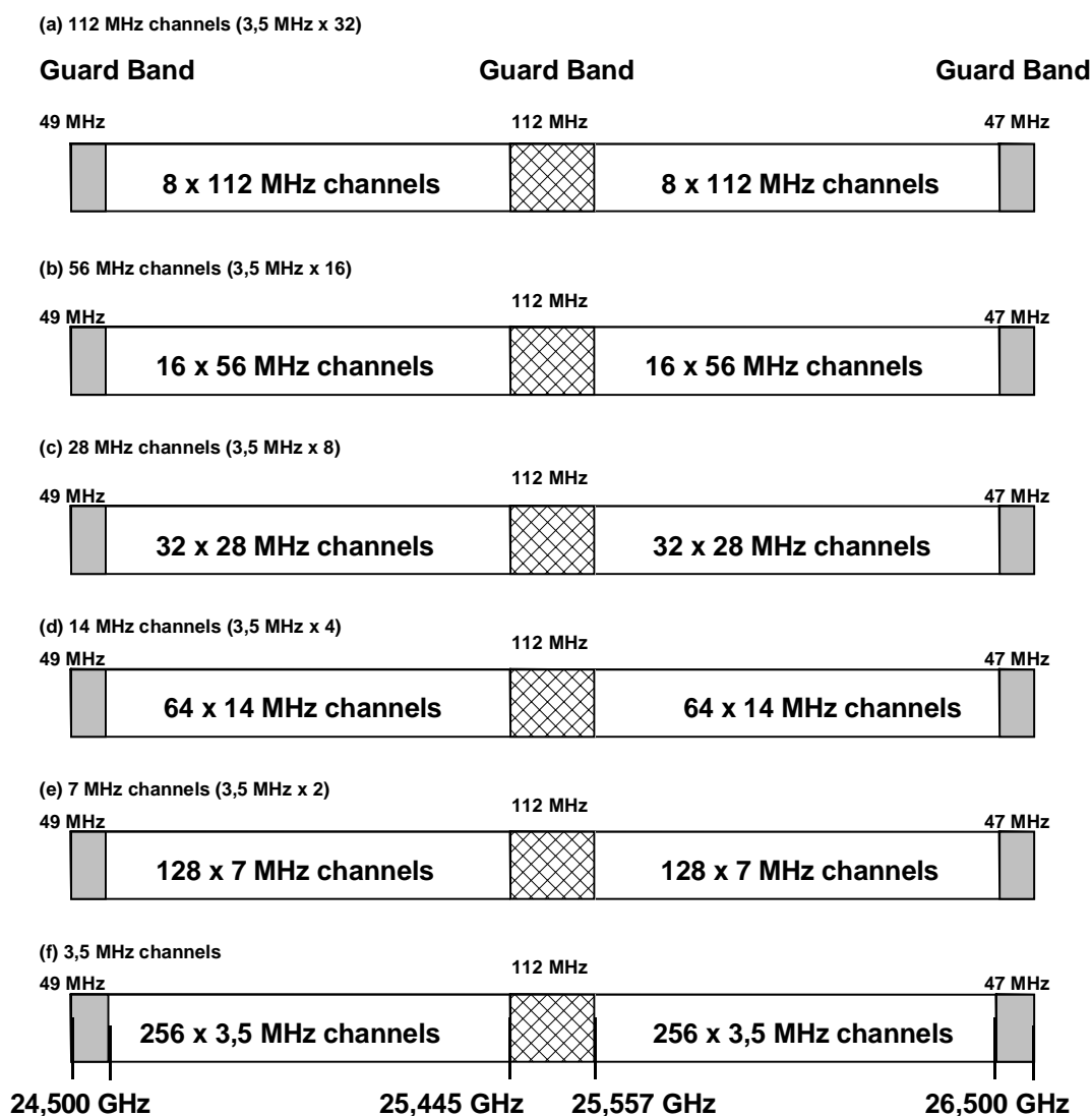
Figure A.1: Radio frequency channel arrangement
