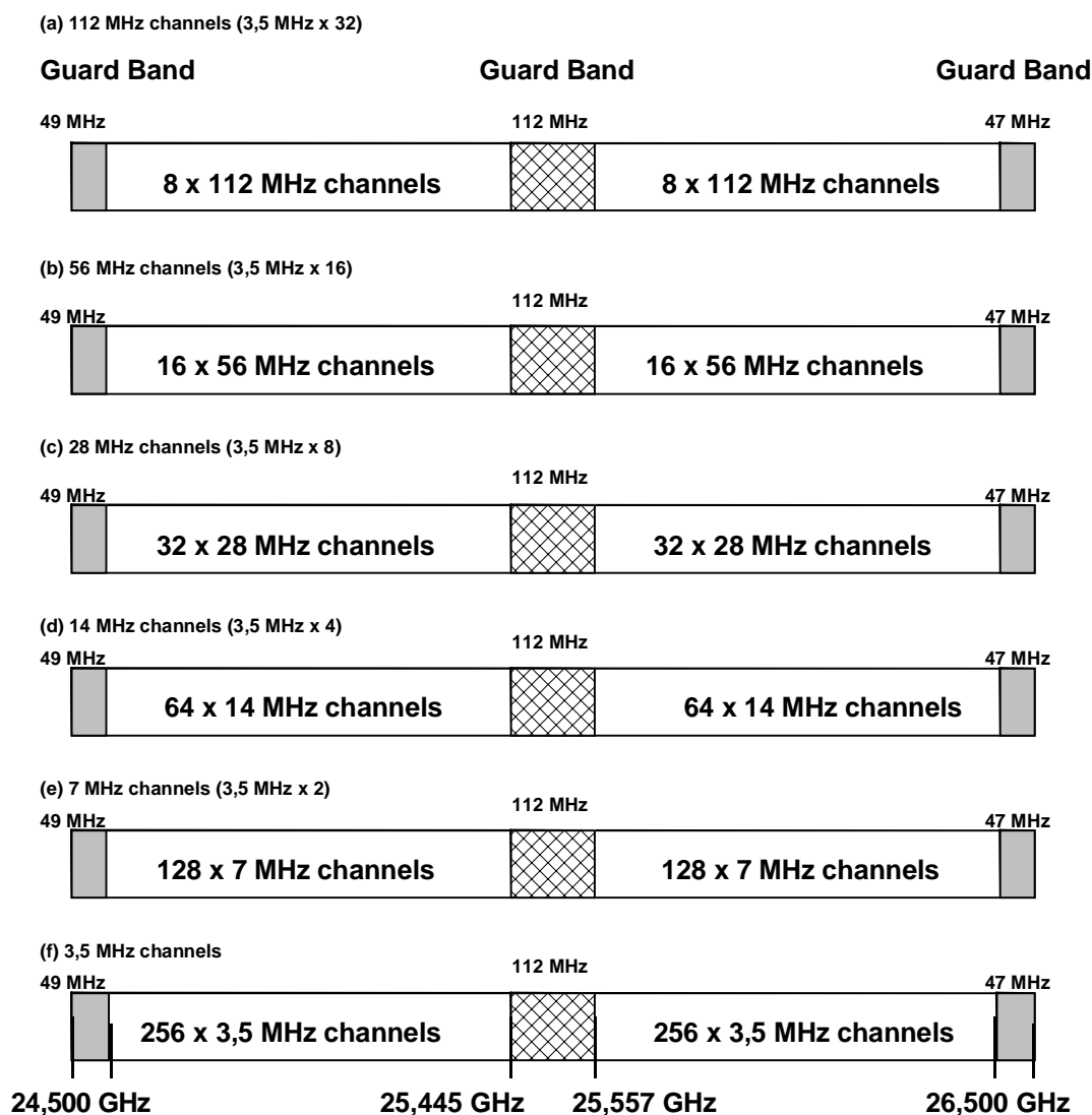
Figure A.1a: Radio frequency channel arrangement
