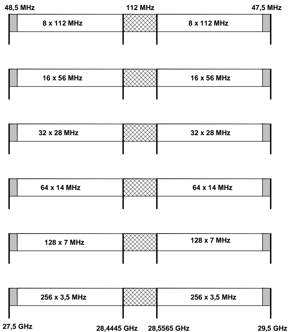
Figure A.1b: Radio frequency channel arrangement
