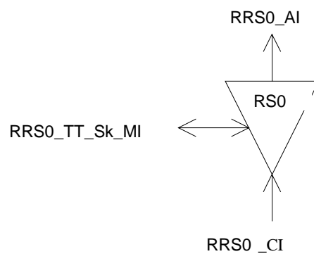
Figure 35: RRS0_TT_Sk symbol
