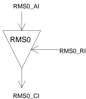
Figure 48: RMS0_TT_So symbol
