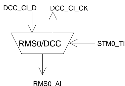
Figure 50: RMS0/DCC_A_So symbol
