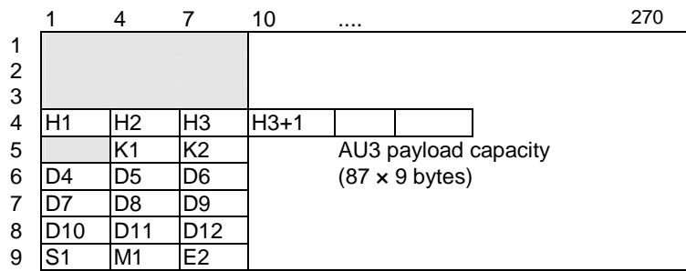
Figure 47: RMS0_AI_D
