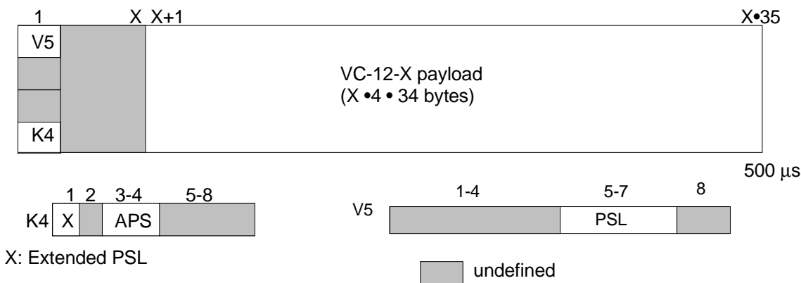
Figure 28: S12-X_AI_D
