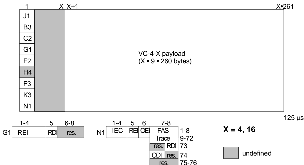
Figure 4: S4-Xc_CI_D
