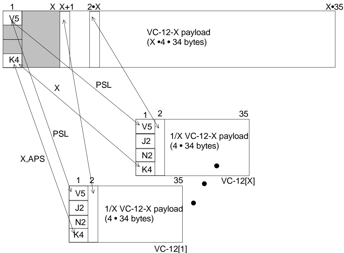
Figure 30: S12-X_AI_D to S12-Xv_CI_D mapping
