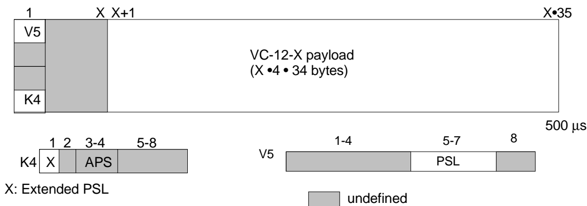
Figure 32: S12-XP_CI_D
