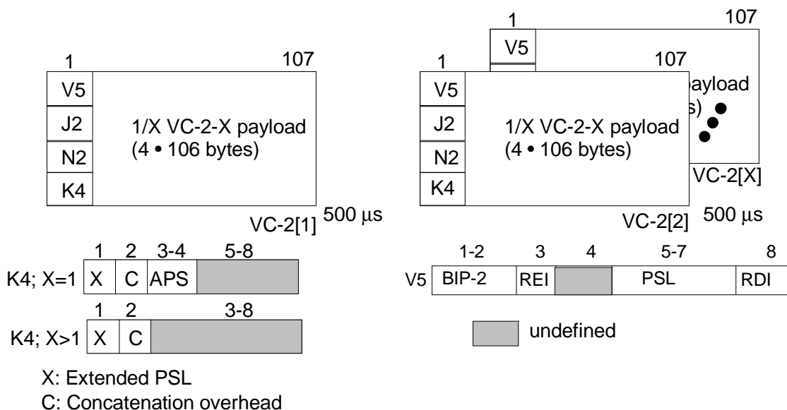
Figure 21: S2-Xv_CI_D
