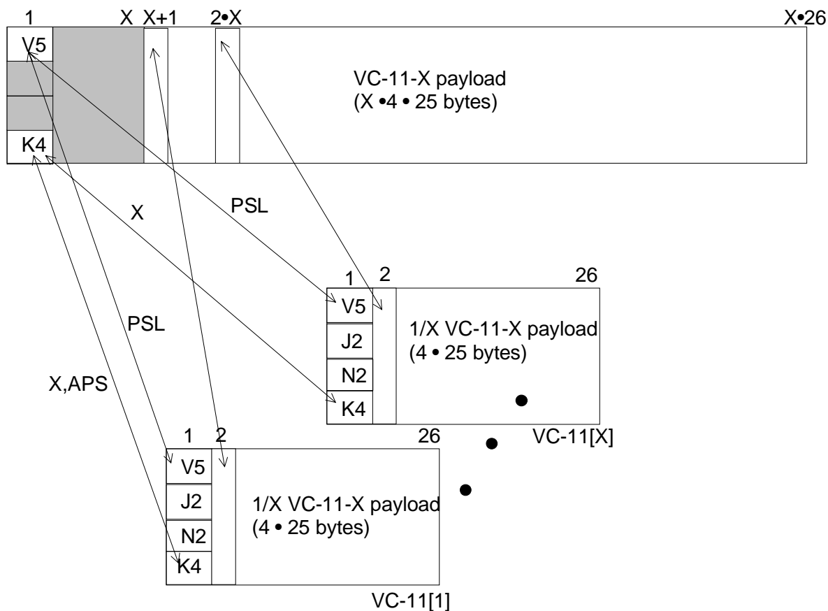
Figure A.5: S11-X_AI_D to S11-Xv_CI_D mapping
