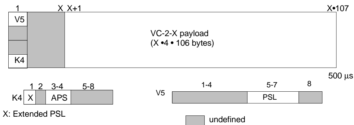
Figure 20: S2-X_AI_D
