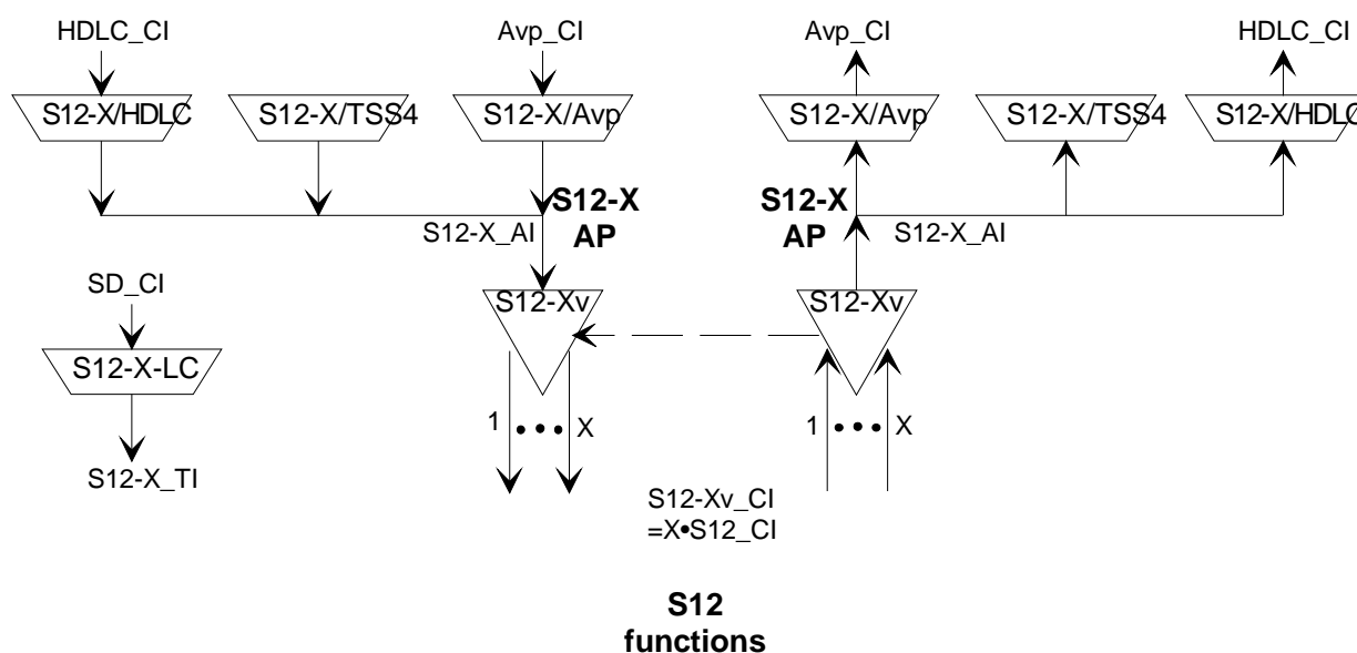
Figure 26: Concatenated VC-12 path layer atomic functions
