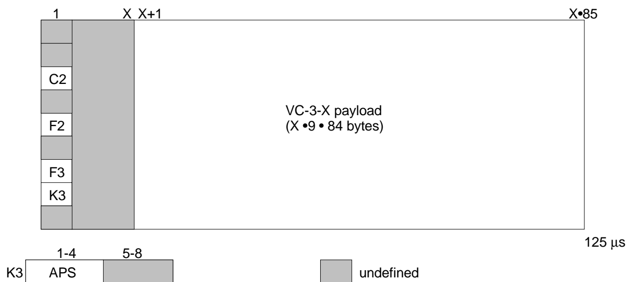
Figure 12: S3-X_AI_D
