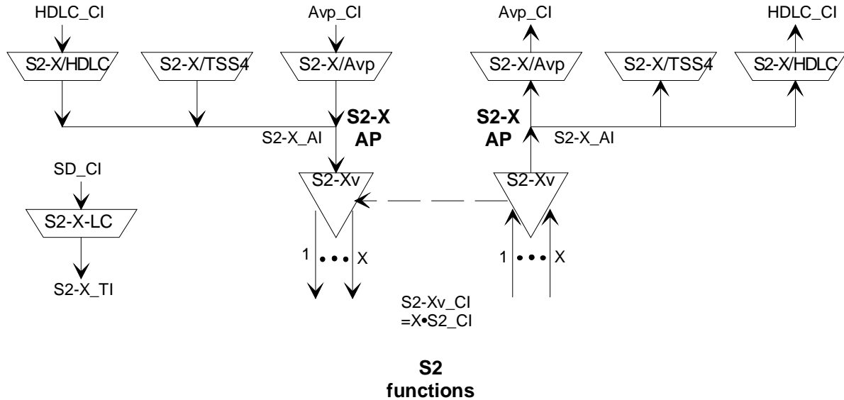
Figure 18: Concatenated VC-2 path layer atomic functions
