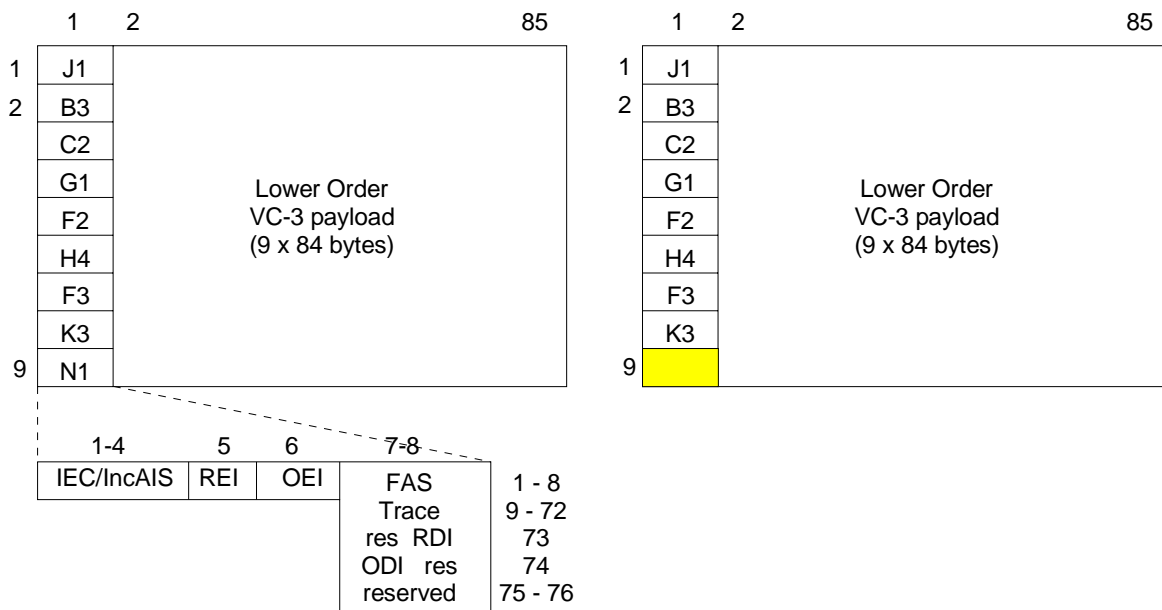
Figure 71: S3_CI_D (left) with defined N1 and S3D_AI_D (right)
