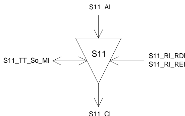
Figure F.8: S11_TT_So symbol
