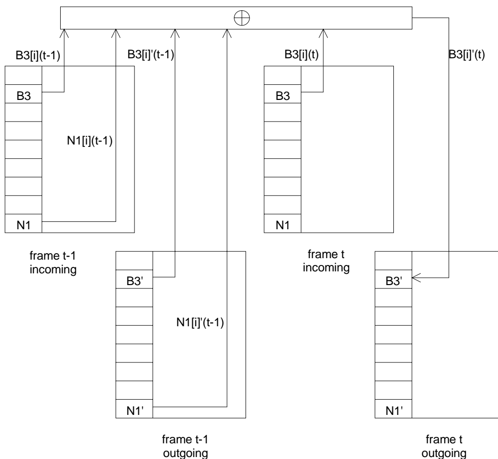
Figure 63: B3[i] , i=1..8 compensating process
