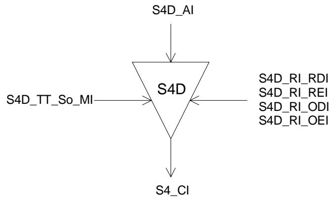
Figure 61: S4D_TT_So symbol
