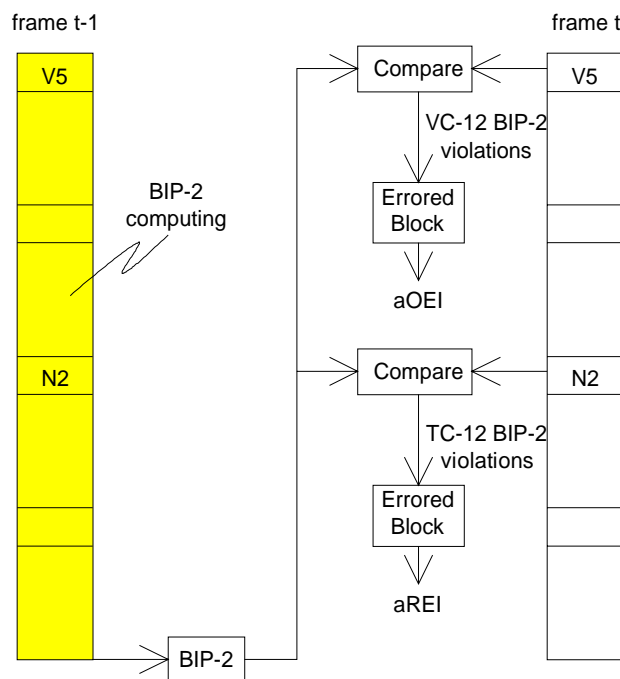
Figure 179: TC-12 and VC-12 BIP-2 computing and comparison
