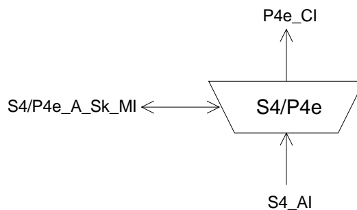
Figure 16: S4/P4e_A_Sk symbol
