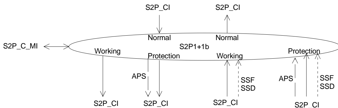
Figure 125: S2P1+1b_C symbol
