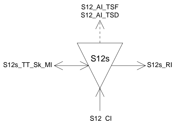
Figure 167: S12s_TT_Sk symbol
