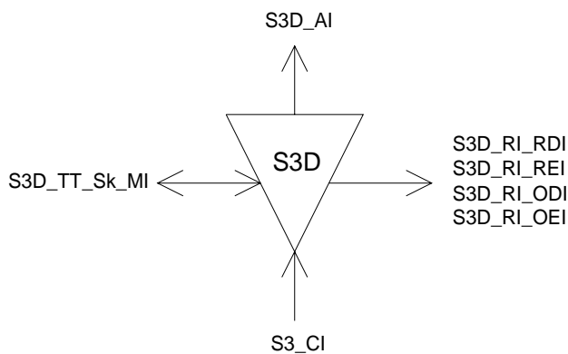
Figure 104: S3D_TT_Sk symbol
