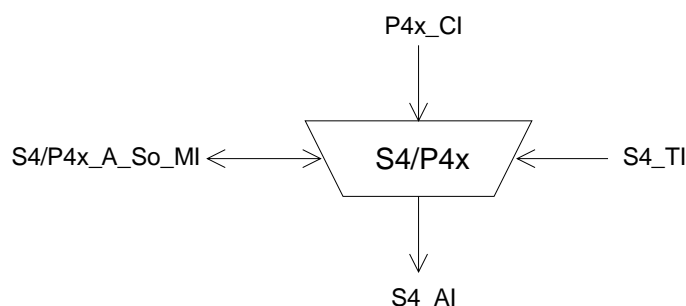
Figure 10: S4/P4x_A_So symbol
