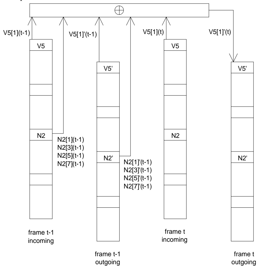
Figure 177: V5[1] compensating process
