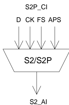
Figure 128: S2/S2P_A_Sk symbol
