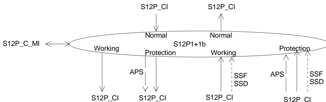
Figure 170: S12P1+1b_C symbol
