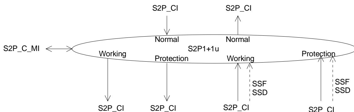
Figure 124: S2P1+1u_C symbol
