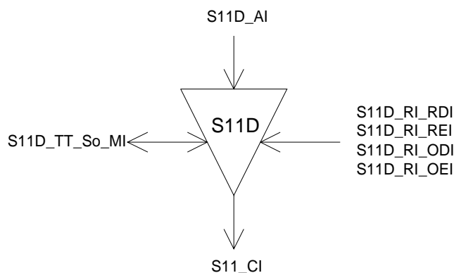
Figure F.26: S11D_TT_So symbol
