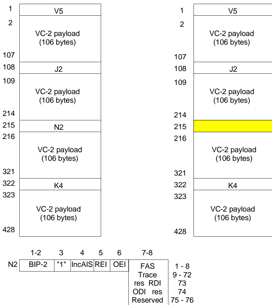
Figure 111: S2_CI_D (left) with defined N2 and S2D_AI_D (right)
