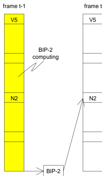
Figure 131: TC BIP-2 computing and insertion
