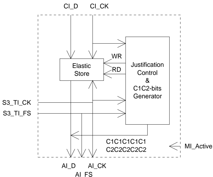
Figure 79: main processes within S3/P31x_A_So
