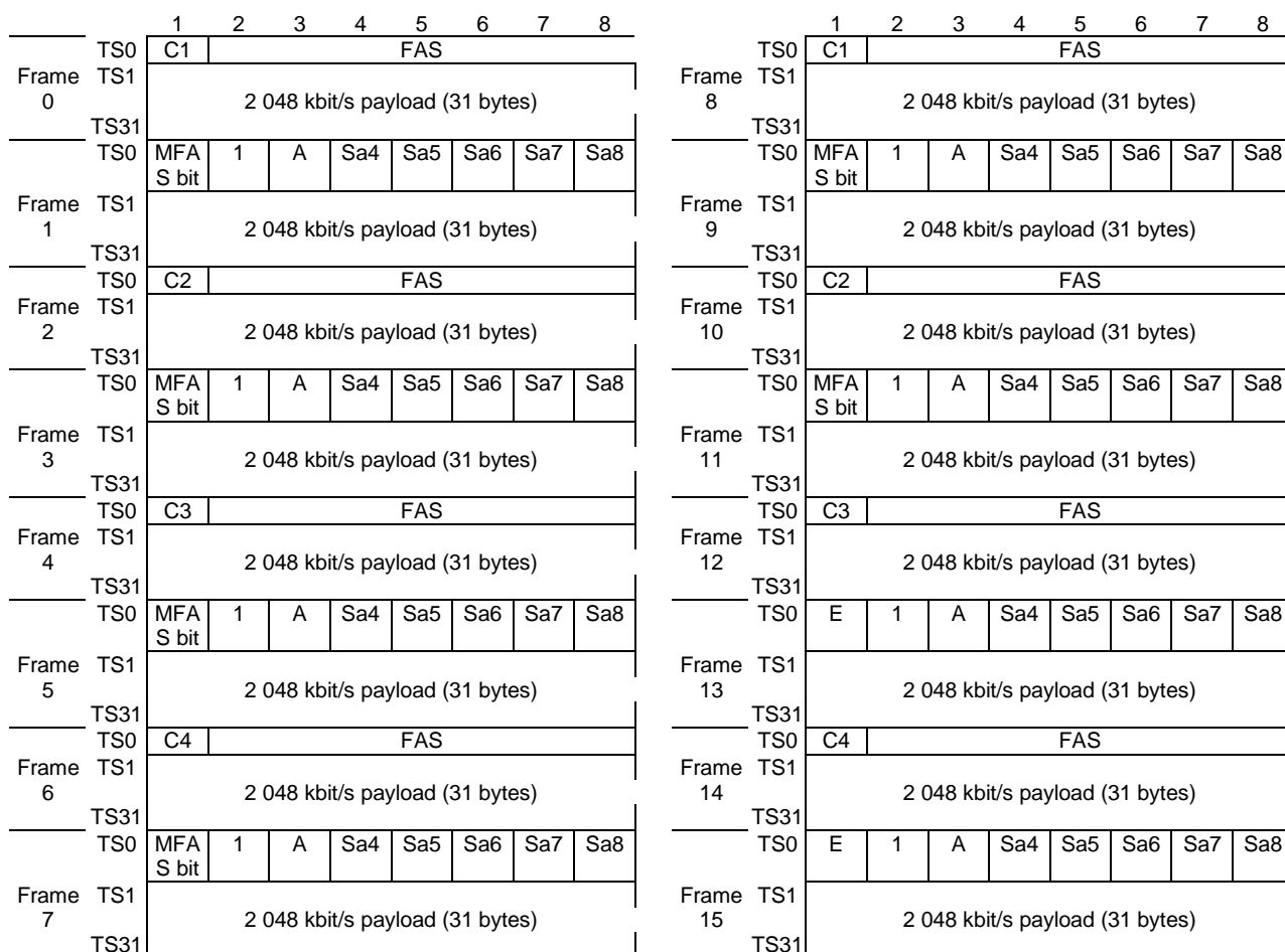
Figure 158: P12s_CI_D (with CRC-4 multiframe)
