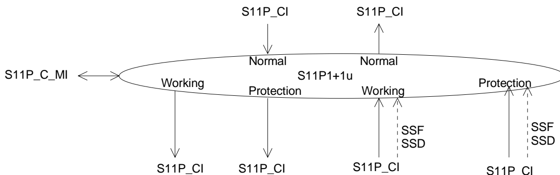
Figure F.20: S11P1+1u_C symbol
