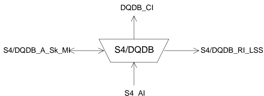
Figure 47: S4/DQDB_A_Sk symbol
