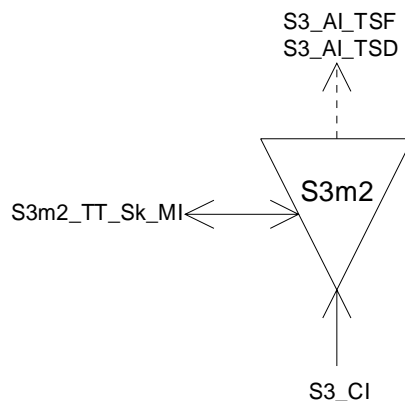
Figure 94: S3m2_TT_Sk symbol
