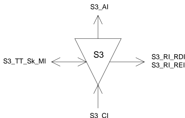
Figure 77: S3_TT_Sk symbol
