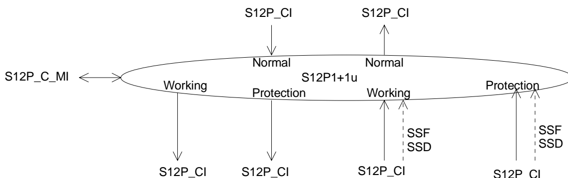
Figure 169: S12P1+1u_C symbol
