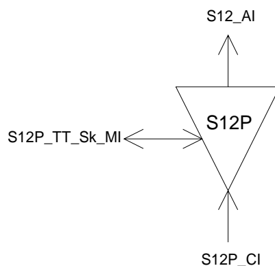
Figure 172: S12P_TT_Sk symbol
