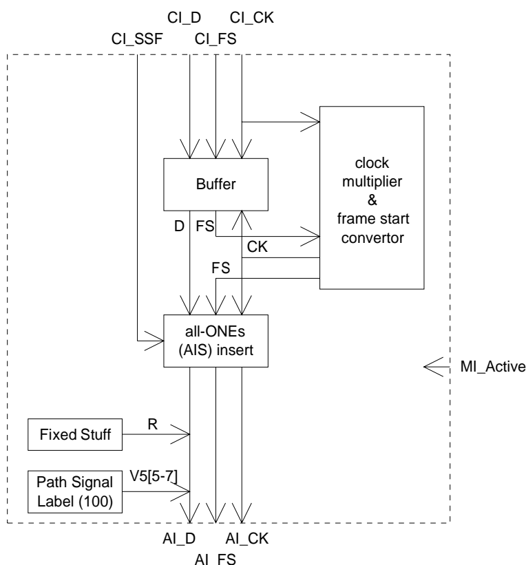
Figure 153: Main processes within S12/P12s_A_So
