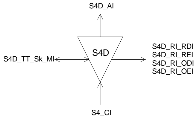
Figure 64: S4D_TT_Sk symbol
