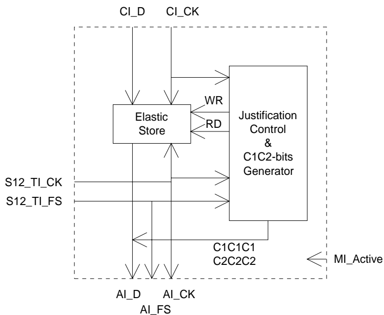
Figure 149: Main processes within S12/P12x_A_So
