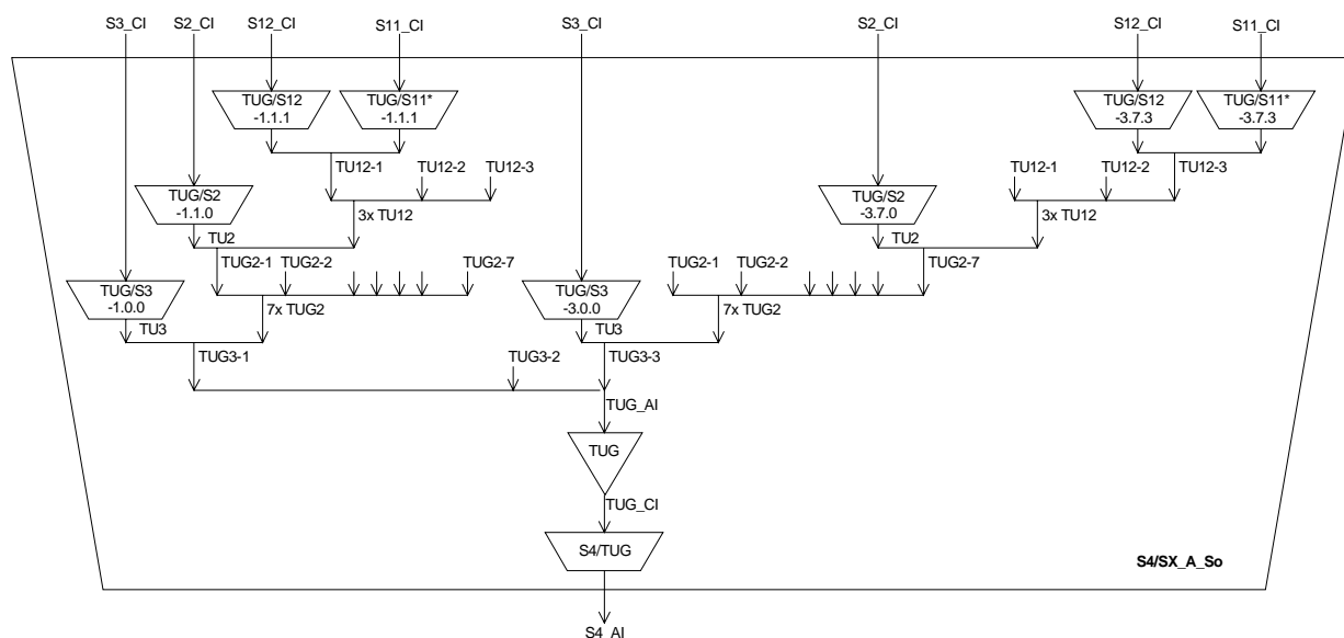
Figure 18: S4/SX_A_So compound function with set of S4/Sm_A_So atomic functions
