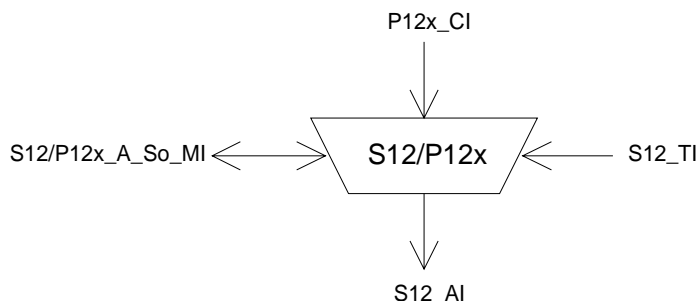
Figure 147: S12/P12x_A_So symbol
