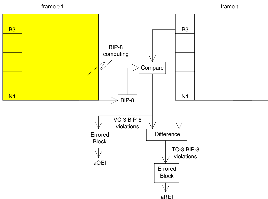
Figure 105: TC-3 and VC-3 BIP-8 computing and comparison
