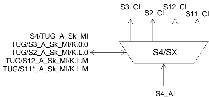
Figure 31: S4/TUG_A_Sk symbol
