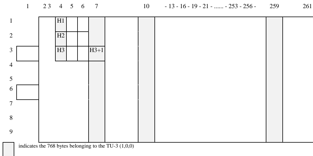
Figure 24: TUG_AI_D/1.0.0 signal
