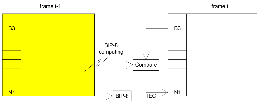
Figure 102: TC IEC computing and insertion
