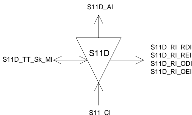
Figure F.29: S11D_TT_Sk symbol
