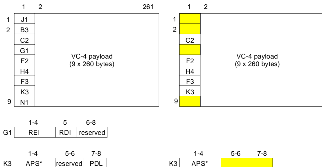
Figure 2: S4_CI_D (left) and S4_AI_D (right)
