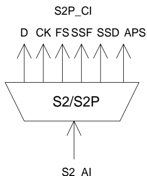
Figure 129: S2/S2P_A_Sk symbol
