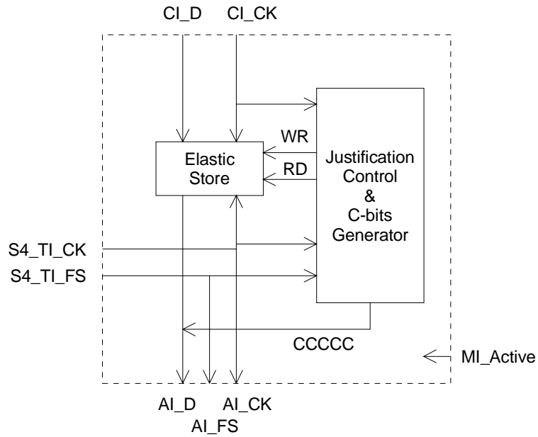
Figure 11: Main processes within S4/P4x_A_So
