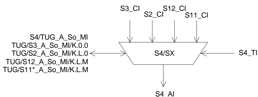
Figure 17: S4/SX_A_So symbol
