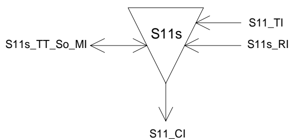
Figure F.17: S11s_TT_So symbol
