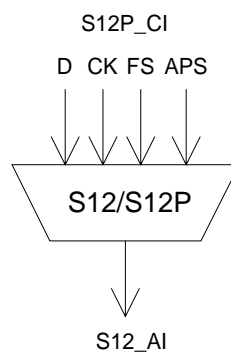
Figure 173: S12/S12P_A_Sk symbol
