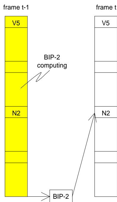
Figure F.27: TC BIP-2 computing and insertion
