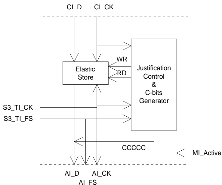
Figure E.2: main processes within S3/P32x_A_So
