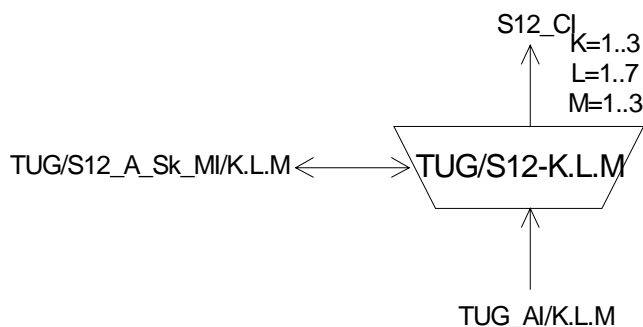
Figure 37: TUG/S12_A_Sk/K.L.M symbol
