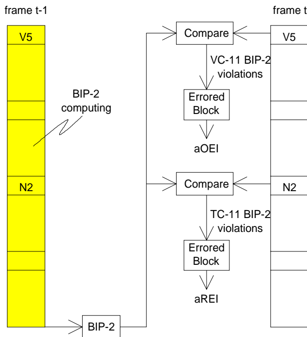
Figure F.30: TC-11 and VC-11 BIP-2 computing and comparison
