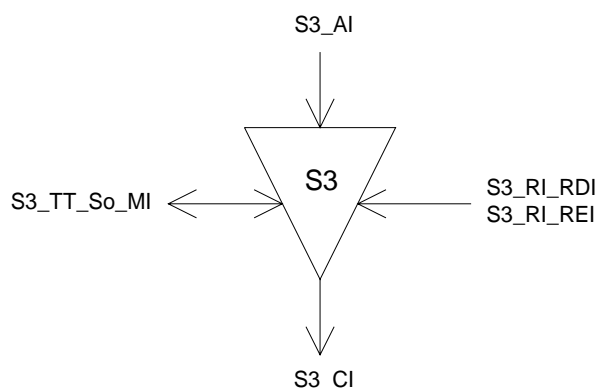
Figure 76: S3_TT_So symbol
