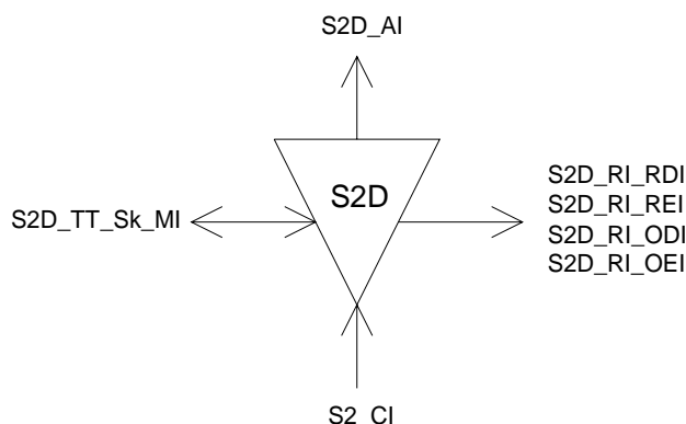
Figure 133: S2D_TT_Sk symbol
