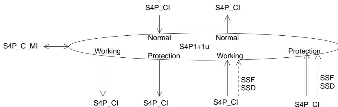
Figure 55: S4P1+1u_C symbol
