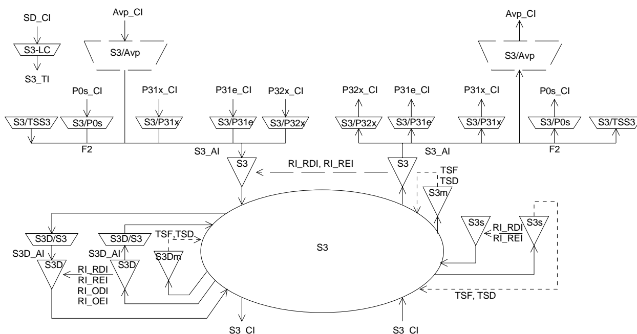
Figure 69: VC-3 path layer atomic functions
