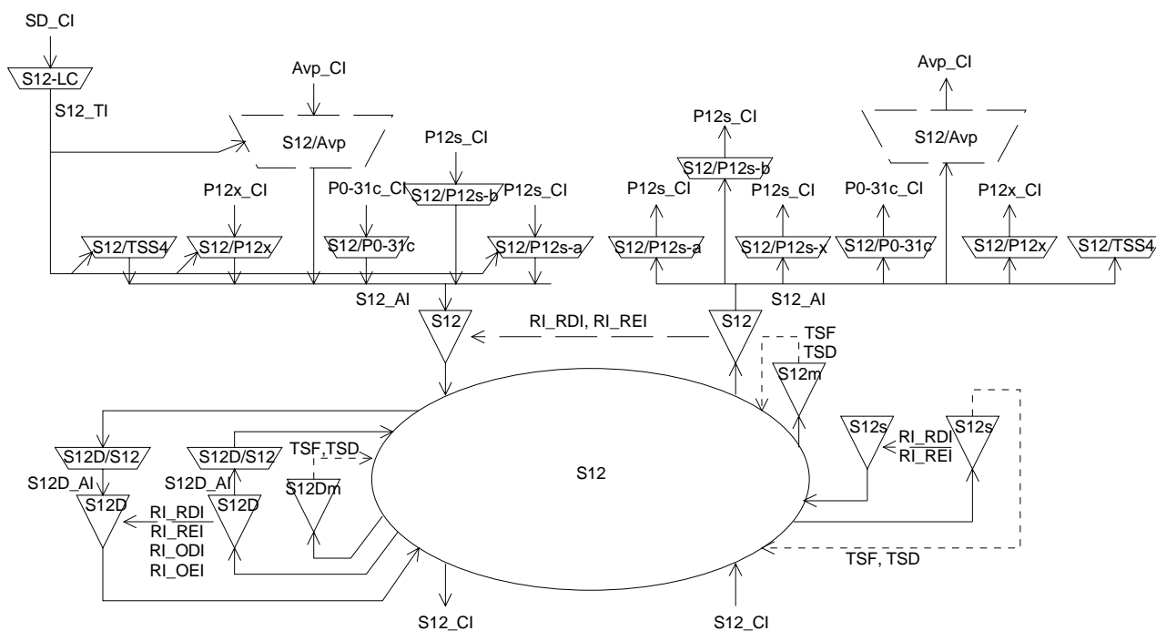
Figure 138: VC-12 Path layer atomic functions
