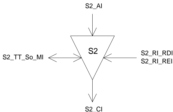
Figure 116: S2_TT_So symbol
