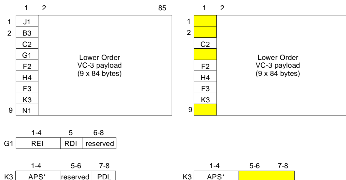
Figure 70: S3_CI_D (left) and S3_AI_D (right)
