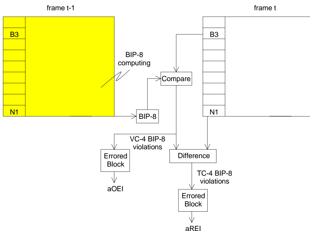
Figure 65: TC-4 and VC-4 BIP-8 computing and comparison
