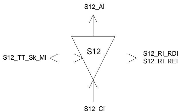
Figure 146: S12_TT_Sk symbol
