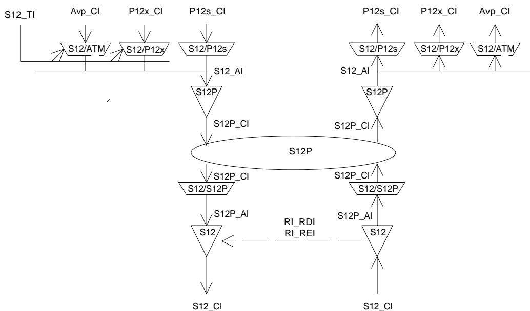
Figure 141: VC-12 Layer Trail Protection atomic functions
