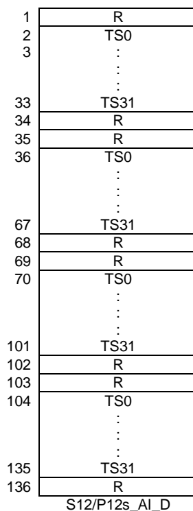
Figure 152: 2 048 kbit/s byte synchronous mapping into Container 12
