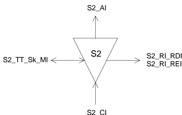
Figure 117: S2_TT_Sk symbol
