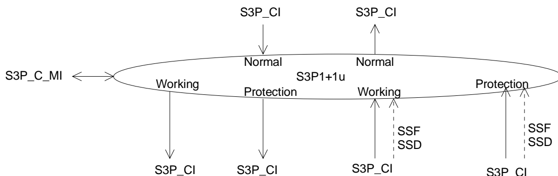
Figure 95: S3P1+1u_C symbol
