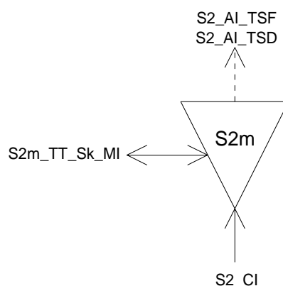
Figure 120: S2m_TT_Sk symbol
