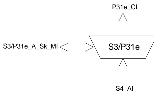
Figure 84: S3/P31e_A_Sk symbol
