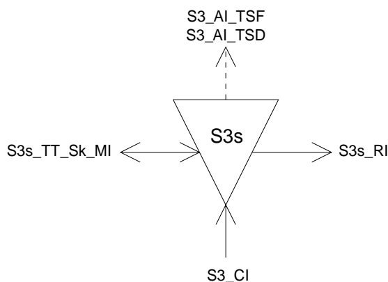
Figure 93: S3s_TT_Sk symbol
