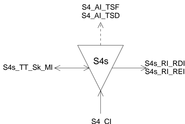
Figure 53: S4s_TT_Sk symbol
