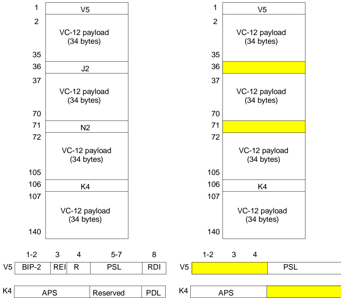
Figure 139: S12_CI_D (left) and S12_AI_D (right)
