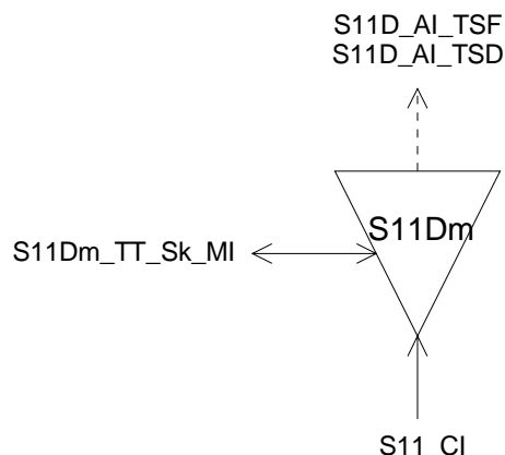
Figure F.33: S11Dm_TT_Sk symbol
