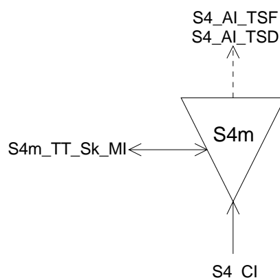
Figure 51: S4m_TT_Sk symbol
