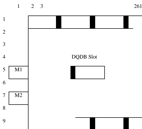
Figure 43: Mapping of DQDB_CI (Slots and Management octet) in the VC-4 structure
