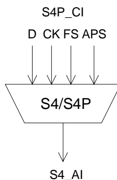
Figure 59: S4/S4P_A_So symbol
