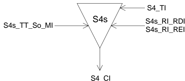
Figure 52: S4s_TT_So symbol
