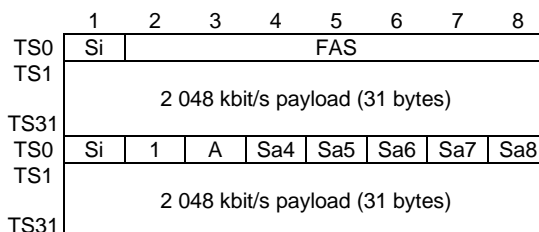
Figure 157: P12s_CI_D (without CRC-4 multiframe)
