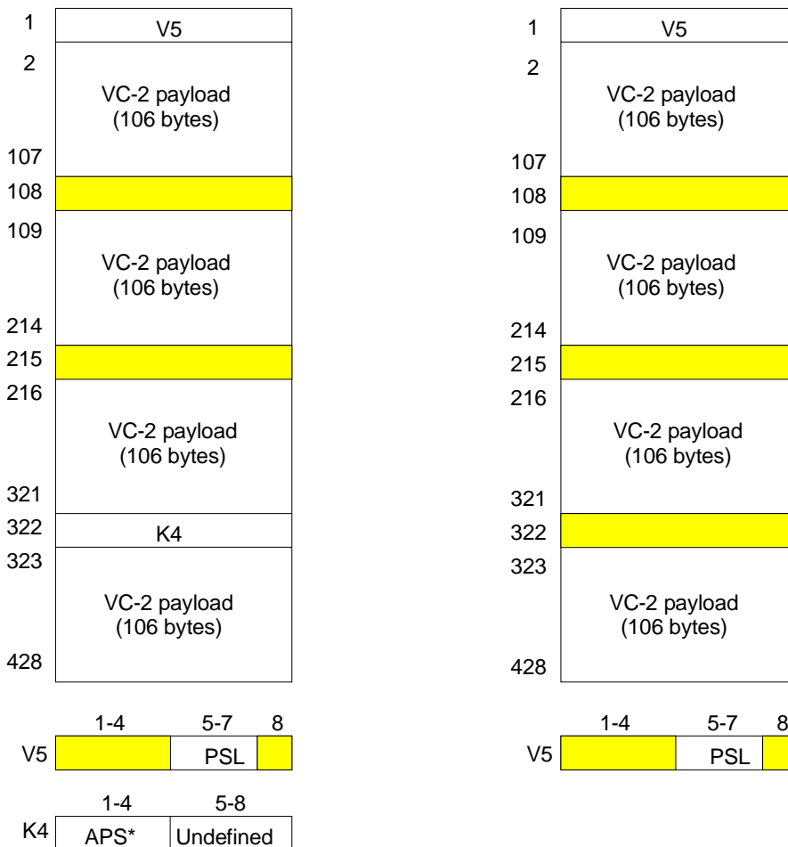
Figure 113: S2P_AI_D (left) and S2P_CI_D (right)
