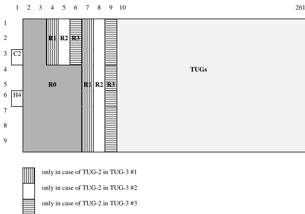
Figure 21: VC-4 payload (TUGs and fixed stuff "R" bytes)
