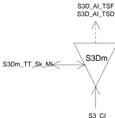
Figure 108: S3Dm_TT_Sk symbol
