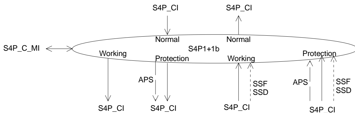
Figure 56: S4P1+1b_C symbol
