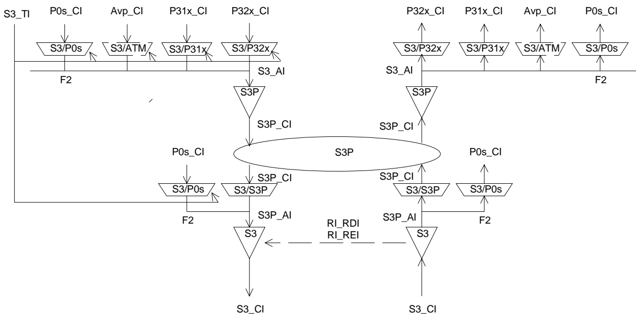
Figure 72: VC-3 Layer Trail Protection atomic functions
