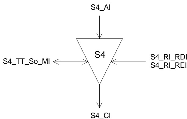
Figure 8: S4_TT_So symbol
