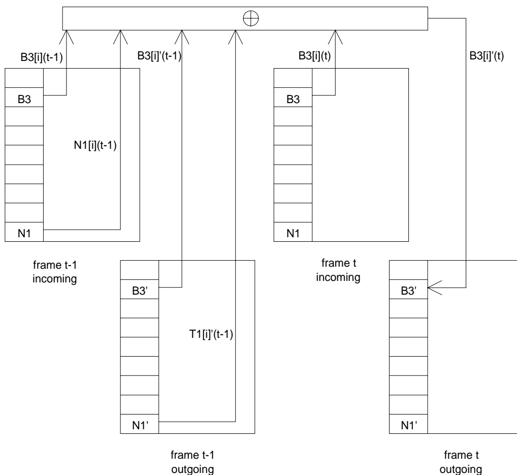
Figure 103: B3[i], i=1..8 compensating process
