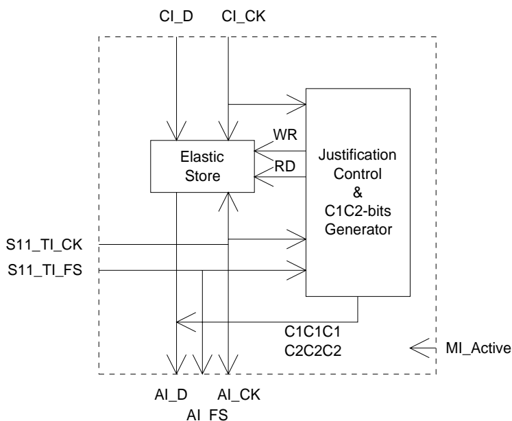
Figure F.12: main processes within S11/P11x_A_So
