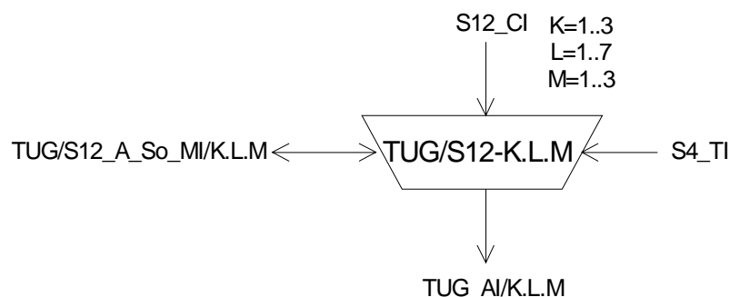
Figure 27: TUG/S12_A_So/K.L.M symbol
