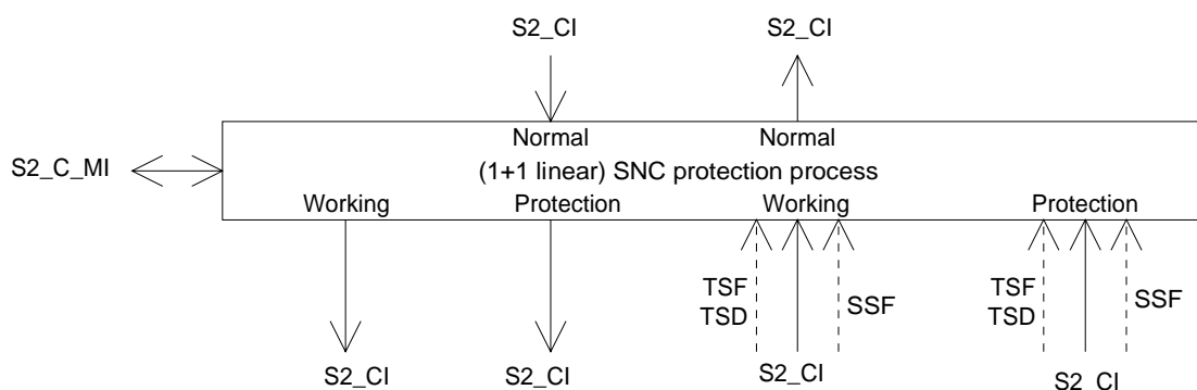
Figure 115: VC-2 1+1 SNC protection process (SNC/I, SNC/N, SNC/S)
