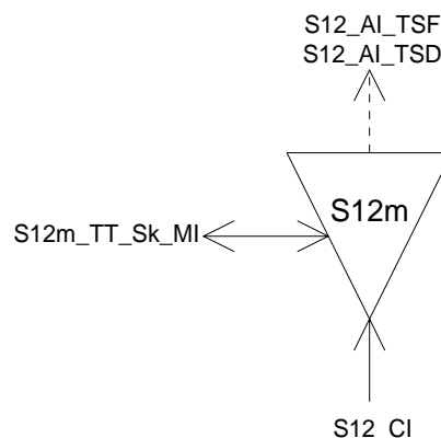
Figure 165: S12m_TT_Sk symbol
