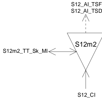
Figure 168: S12m2_TT_Sk symbol
