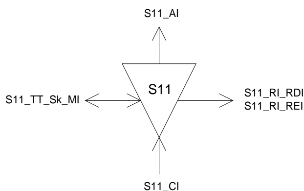
Figure F.9: S11_TT_Sk symbol
