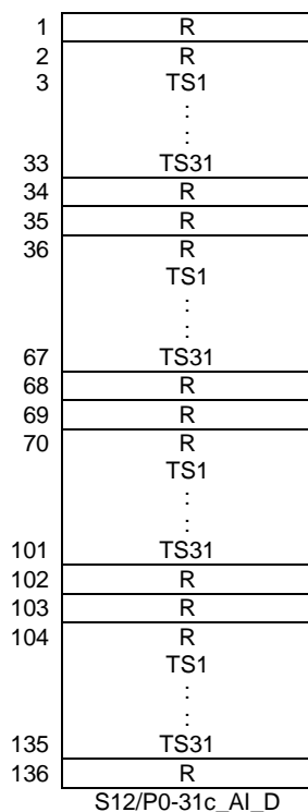
Figure 161: 1 984 kbit/s byte synchronous mapping into Container 12
