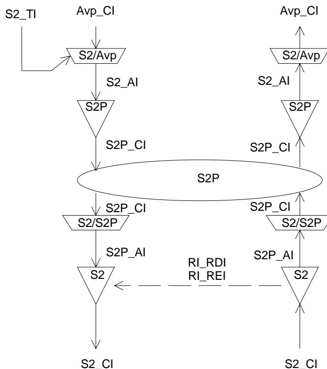
Figure 112: VC-2 Layer Trail Protection atomic functions
