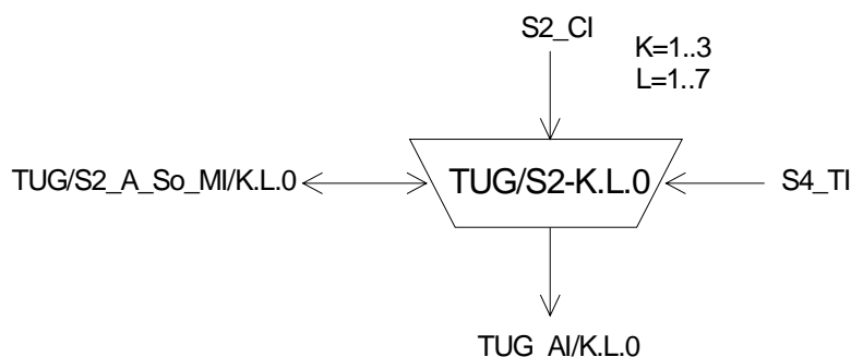
Figure 25: TUG/S2_A_So/K.L.0 symbol
