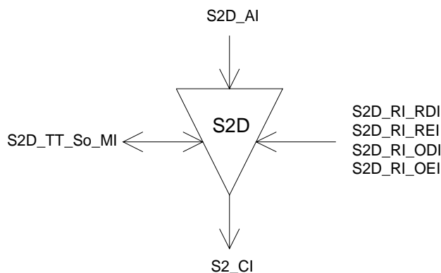
Figure 130: S2D_TT_So symbol
