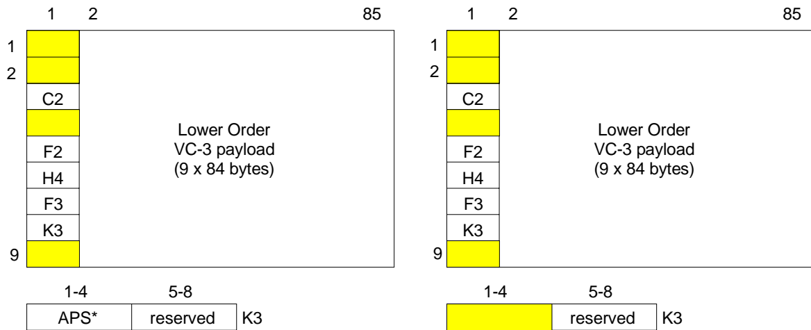
Figure 73: S3P_AI_D (left) and S3P_CI_D (right) signals
