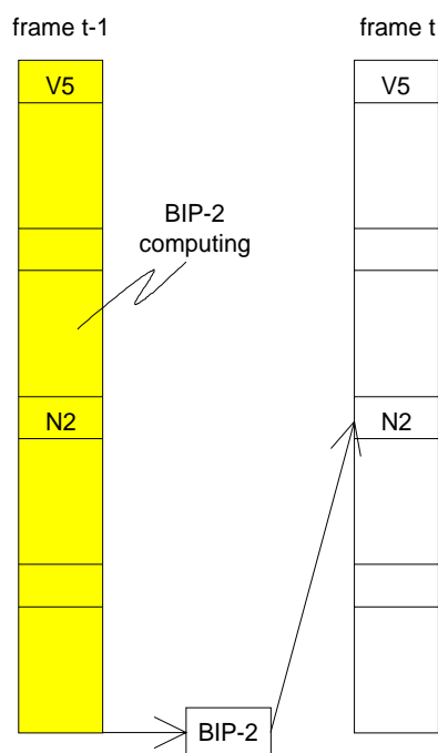
Figure 176: TC BIP-2 computing and insertion
