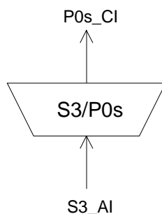
Figure 87: S3/P0s_A_Sk symbol
