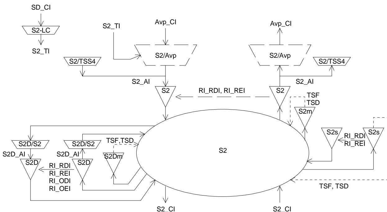
Figure 109: VC-2 Path layer atomic functions
