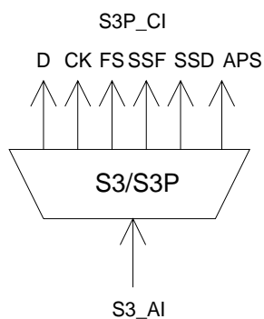
Figure 100: S3/S3P_A_Sk symbol
