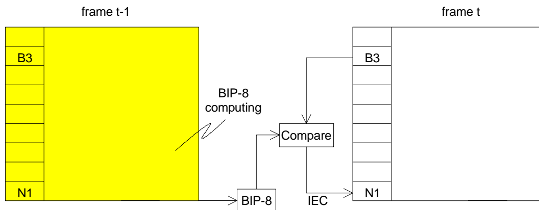
Figure 62: TC IEC computing and insertion
