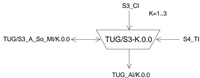
Figure 23: TUG/S3_A_So/K.0.0 symbol
