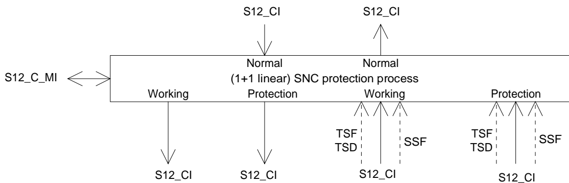
Figure 144: VC-12 1+1 SNC protection process (SNC/I, SNC/N, SNC/S)
