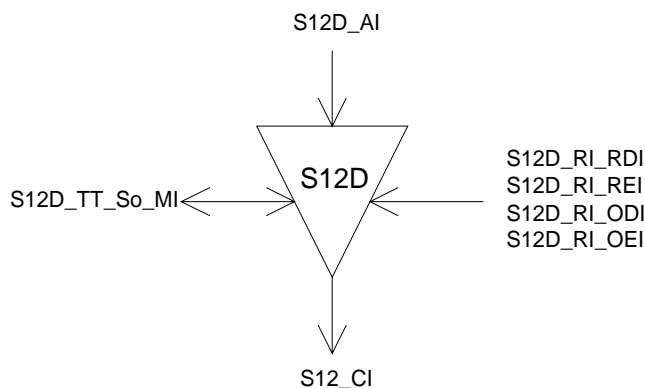
Figure 175: S12D_TT_So symbol
