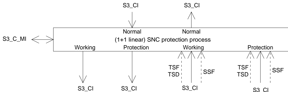
Figure 75: VC-3 1+1 SNC protection process (SNC/I, SNC/N, SNC/S)
