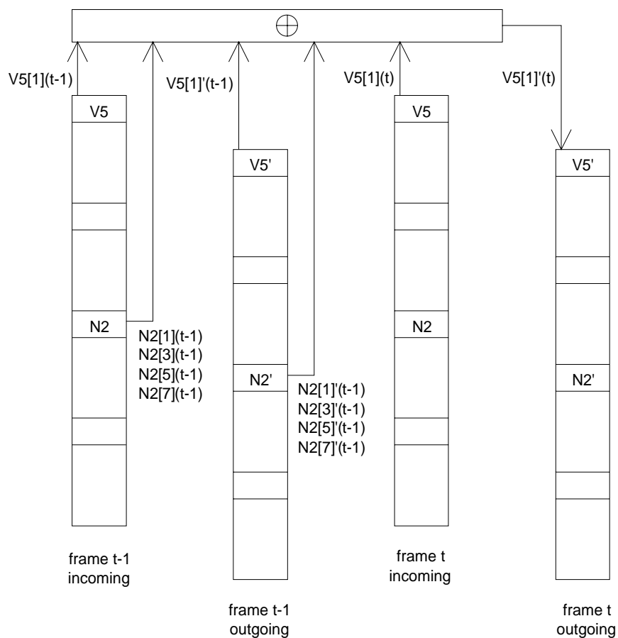
Figure 132: V5[1] compensating process
