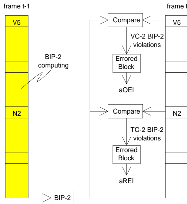
Figure 134: TC-2 and VC-2 BIP-2 computing and comparison
