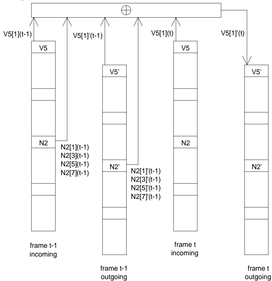
Figure F.28: V5[1] compensating process
