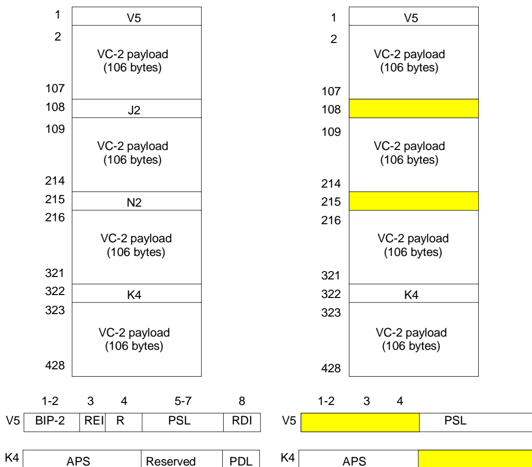
Figure 110: S2_CI_D (left) and S2_AI_D (right)
