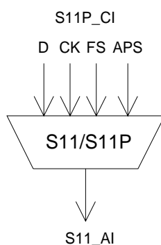
Figure F.24: S11/S11P_A_Sk symbol
