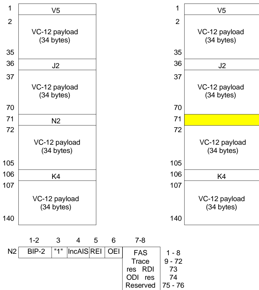
Figure 140: S12_CI_D (left) with defined N2 and S12D_AI_D (right)
