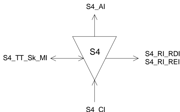
Figure 9: S4_TT_Sk symbol
