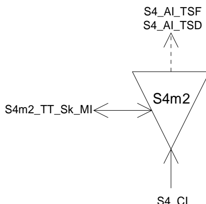
Figure 54: S4m2_TT_Sk symbol
