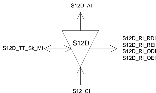
Figure 178: S12D_TT_Sk symbol
