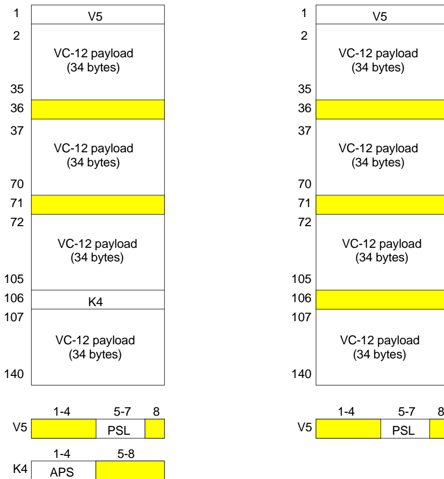
Figure 142: S12P_AI_D (left) and S12P_CI_D (right)
