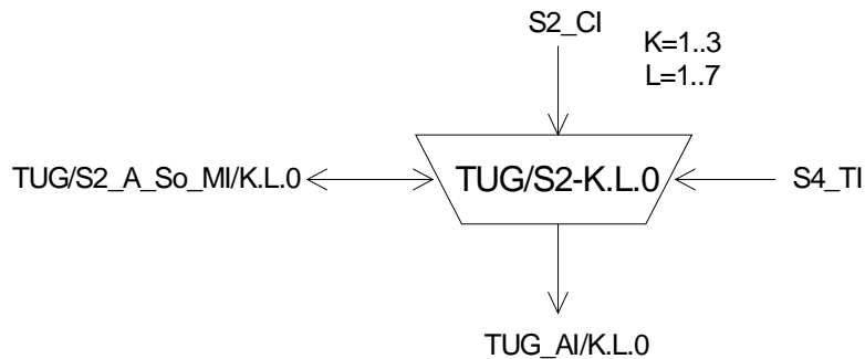
Figure 25: TUG/S2_A_So/K.L.0 symbol
