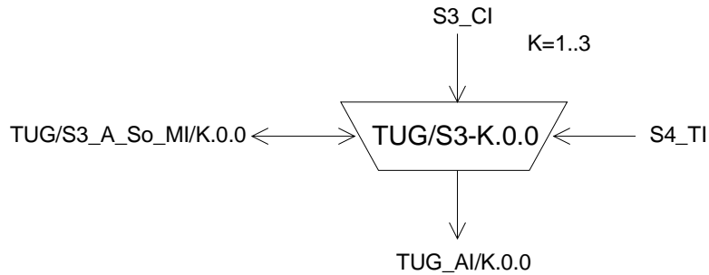
Figure 23: TUG/S3_A_So/K.0.0 symbol
