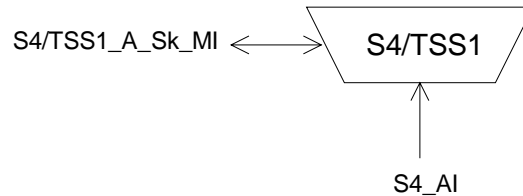
Figure 50: S4/TSS1_A_Sk symbol
