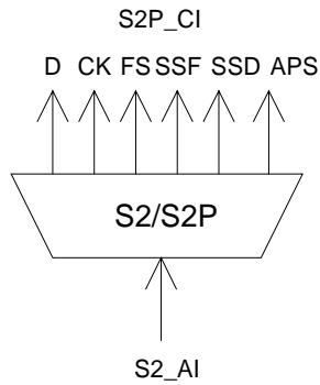
Figure 129: S2/S2P_A_Sk symbol
