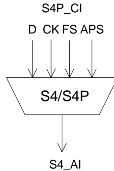
Figure 59: S4/S4P_A_So symbol
