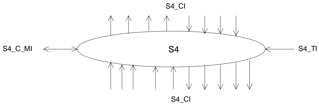
Figure 6: S4_C symbol
