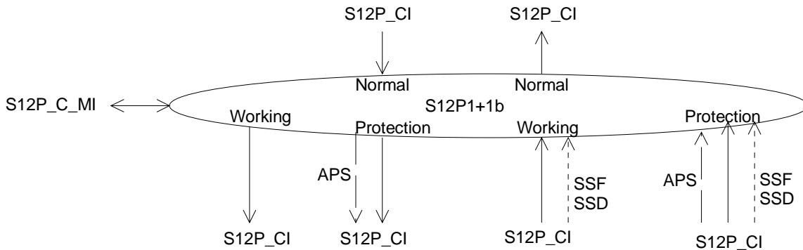
Figure 170: S12P1+1b_C symbol
