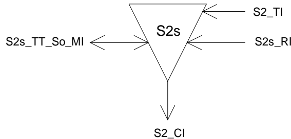
Figure 121: S2s_TT_So symbol
