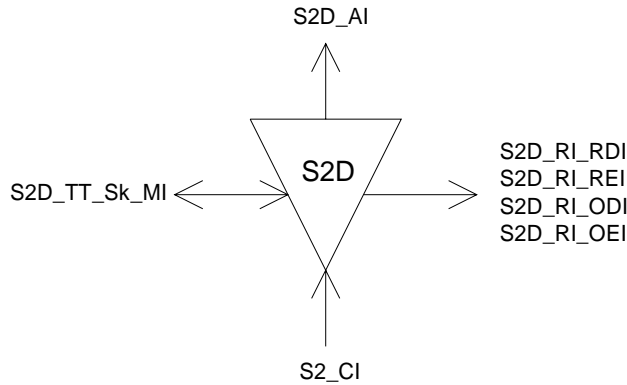
Figure 133: S2D_TT_Sk symbol
