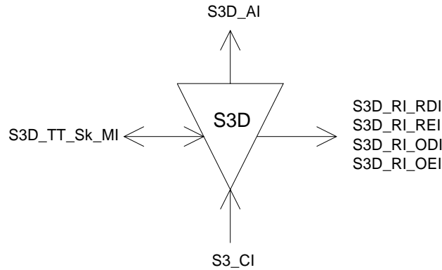
Figure 104: S3D_TT_Sk symbol
