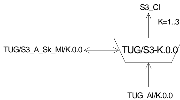
Figure 35: TUG/S3_A_Sk/K.0.0 symbol
