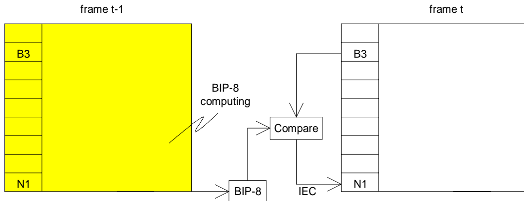
Figure 102: TC IEC computing and insertion
