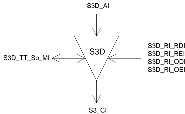
Figure 101: S3D_TT_So symbol
