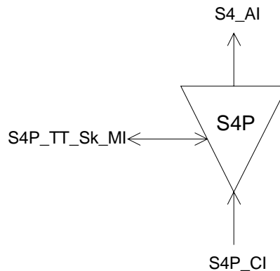
Figure 58: S4P_TT_Sk symbol
