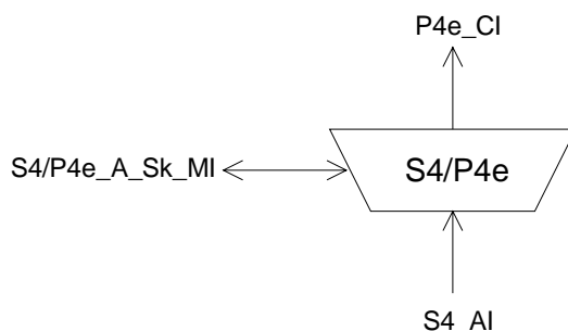
Figure 16: S4/P4e_A_Sk symbol
