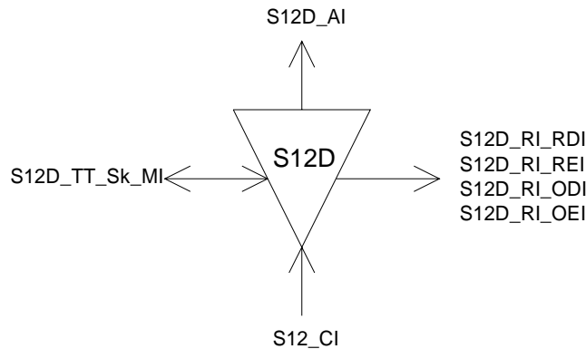
Figure 178: S12D_TT_Sk symbol
