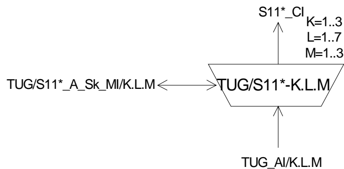
Figure 38: TUG/S11*_A_Sk symbol
