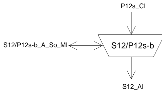
Figure 151: S12/P12s-b_A_So symbol
