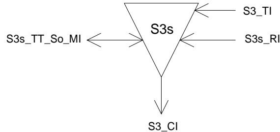
Figure 92: S3s_TT_So symbol
