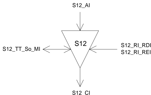
Figure 145: S12_TT_So symbol
