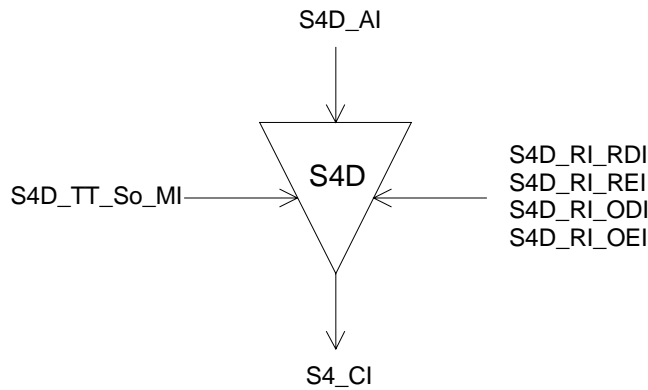
Figure 61: S4D_TT_So symbol
