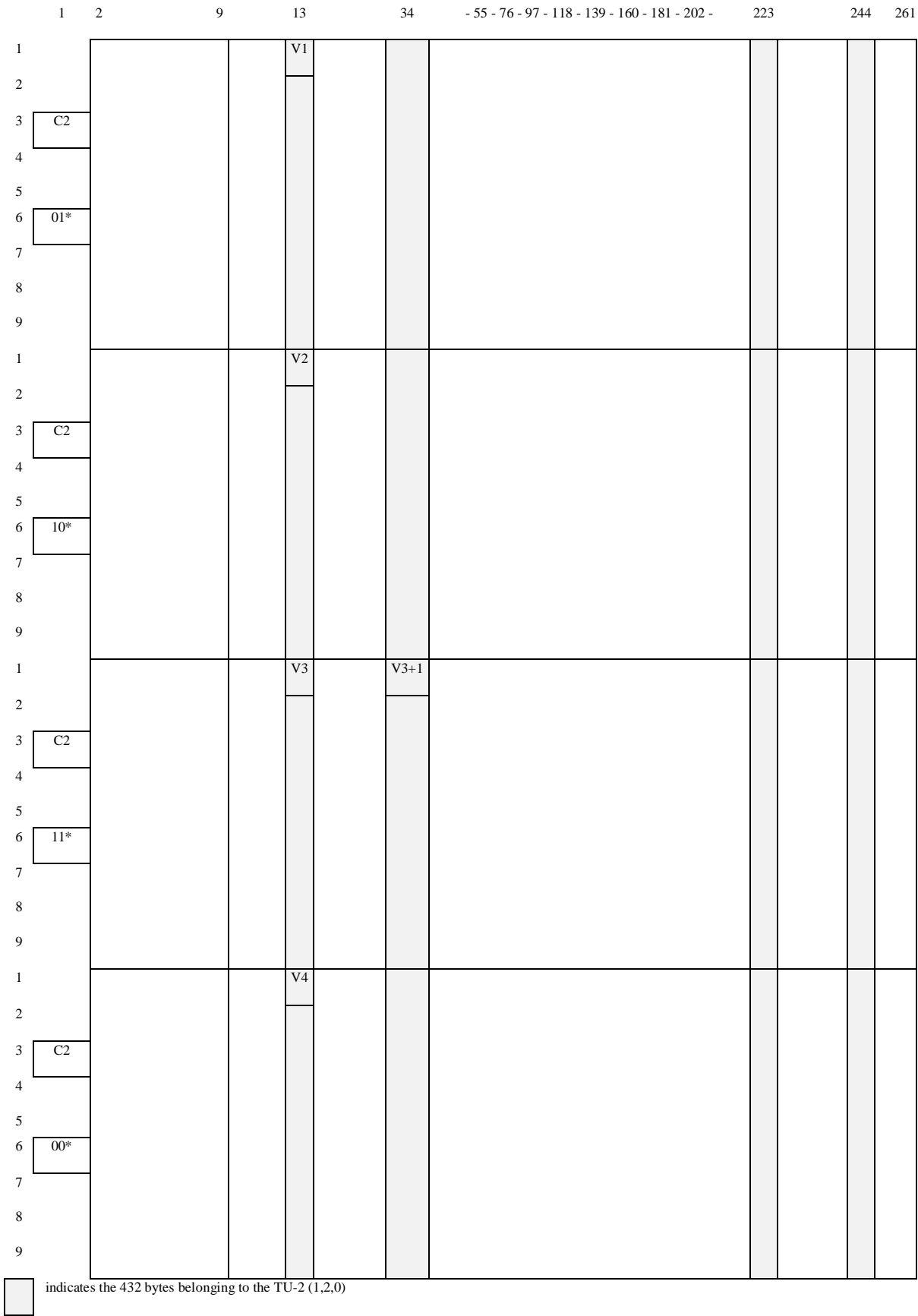
Figure 26: TUG_AI_D/1.2.0 signal
