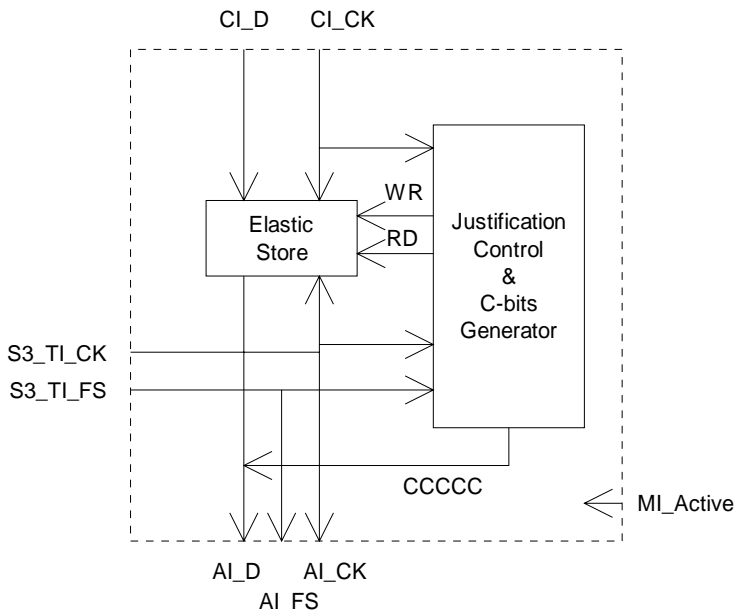
Figure E.2: main processes within S3/P32x_A_So
