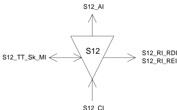
Figure 146: S12_TT_Sk symbol
