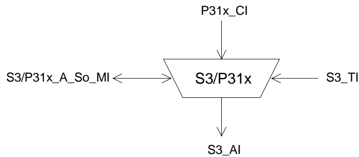
Figure 78: S3/P31x_A_So symbol
