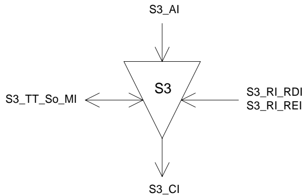
Figure 76: S3_TT_So symbol
