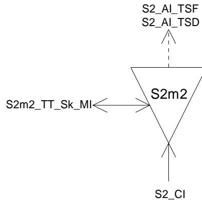
Figure 123: S2m2_TT_Sk symbol
