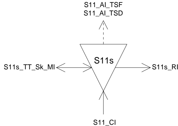
Figure F.18: S11s_TT_Sk symbol
