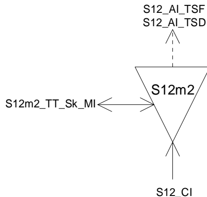
Figure 168: S12m2_TT_Sk symbol
