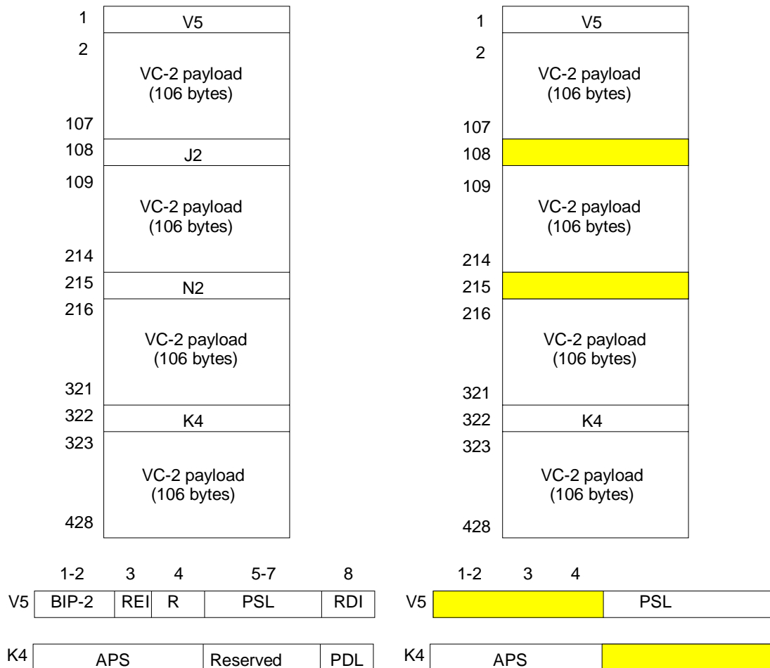
Figure 110: S2_CI_D (left) and S2_AI_D (right)
