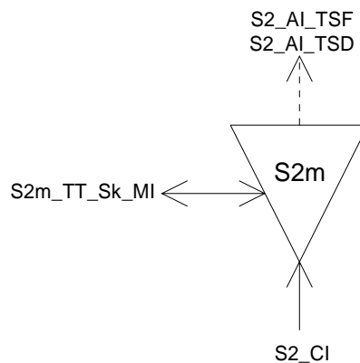
Figure 120: S2m_TT_Sk symbol
