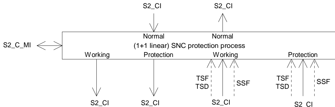
Figure 115: VC-2 1+1 SNC protection process (SNC/I, SNC/N, SNC/S)
