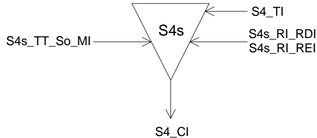
Figure 52: S4s_TT_So symbol
