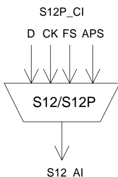
Figure 173: S12/S12P_A_Sk symbol
