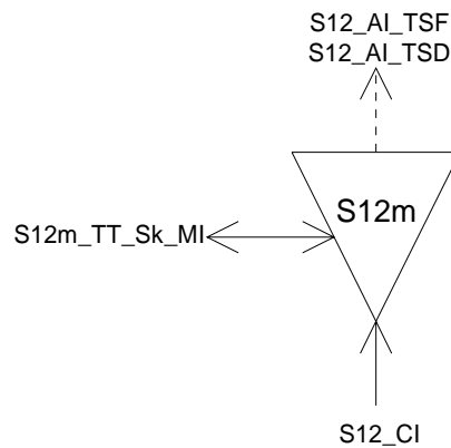
Figure 165: S12m_TT_Sk symbol
