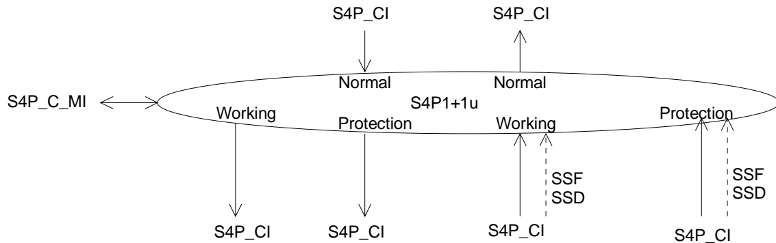
Figure 55: S4P1+1u_C symbol
