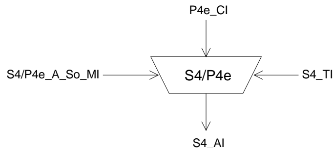
Figure 15: S4/P4e_A_So symbol
