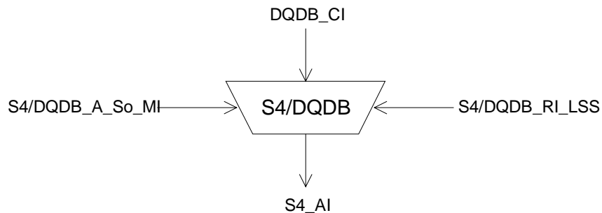
Figure 42: S4/DQDB_A_So symbol
