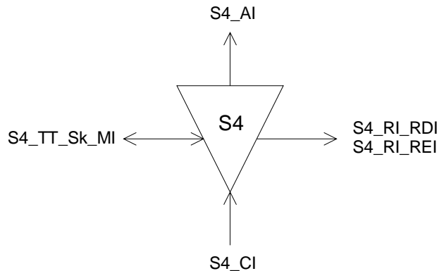
Figure 9: S4_TT_Sk symbol
