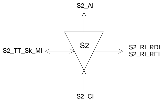
Figure 117: S2_TT_Sk symbol
