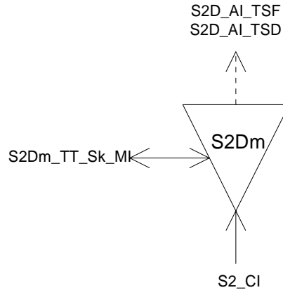
Figure 137: S2Dm_TT_Sk symbol
