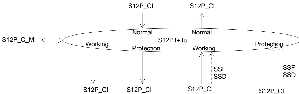
Figure 169: S12P1+1u_C symbol
