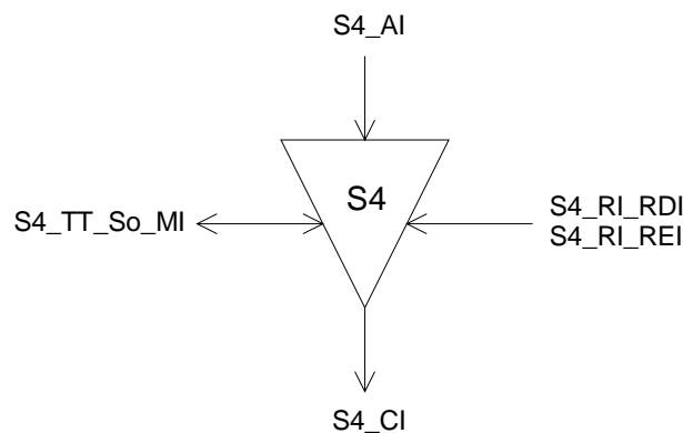
Figure 8: S4_TT_So symbol
