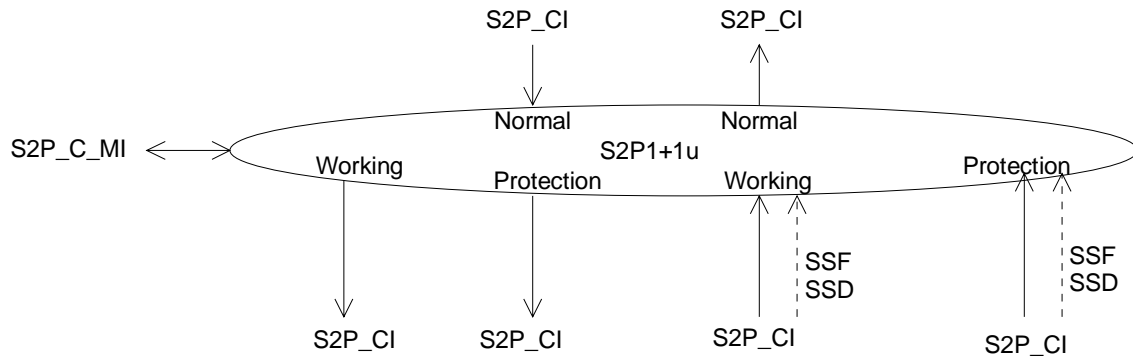
Figure 124: S2P1+1u_C symbol
