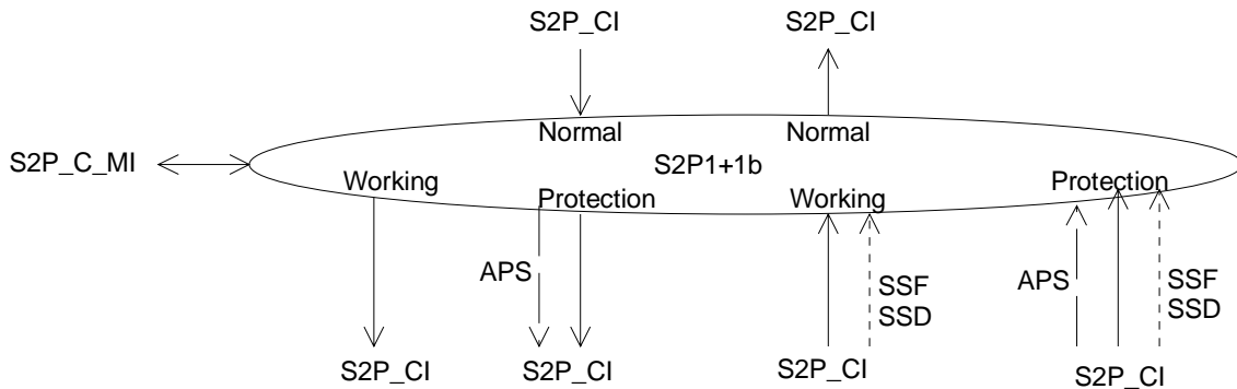
Figure 125: S2P1+1b_C symbol
