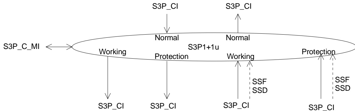
Figure 95: S3P1+1u_C symbol
