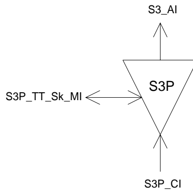
Figure 98: S3P_TT_Sk symbol
