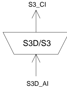
Figure 107: S3D/S3_A_Sk symbol
