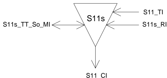
Figure F.17: S11s_TT_So symbol
