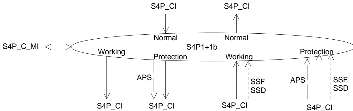
Figure 56: S4P1+1b_C symbol
