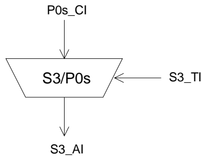
Figure 85: S3/P0s_A_So symbol
