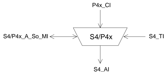
Figure 10: S4/P4x_A_So symbol
