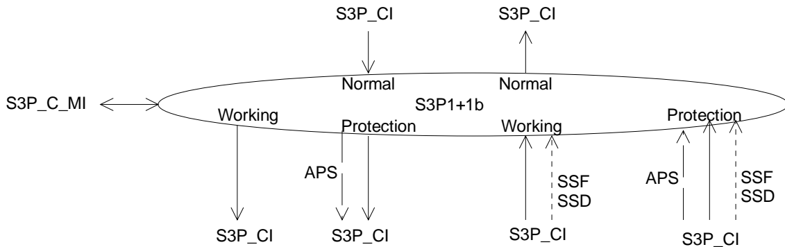
Figure 96: S3P1+1b_C symbol
