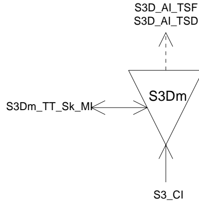
Figure 108: S3Dm_TT_Sk symbol
