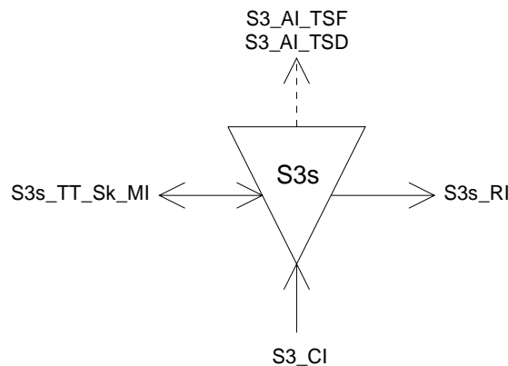
Figure 93: S3s_TT_Sk symbol
