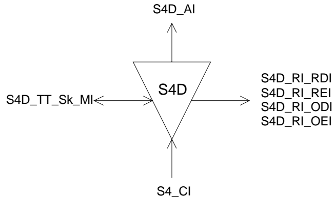
Figure 64: S4D_TT_Sk symbol
