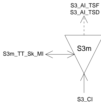
Figure 91: S3m_TT_Sk symbol
