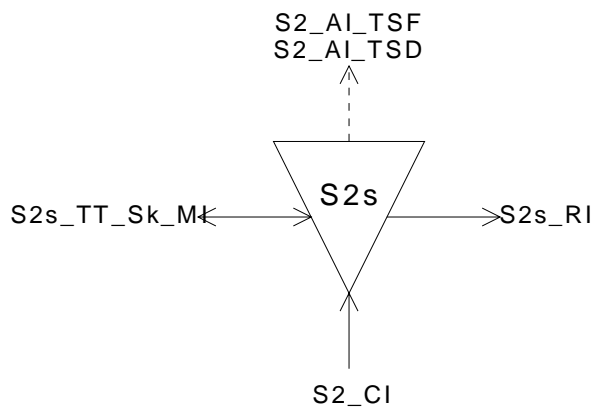
Figure 122: S2s_TT_Sk symbol
