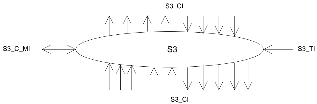
Figure 74: S3_C symbol
