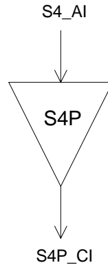
Figure 57: S4P_TT_So symbol
