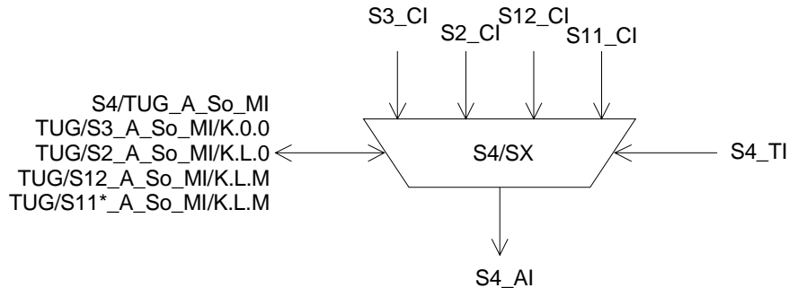
Figure 17: S4/SX_A_So symbol
