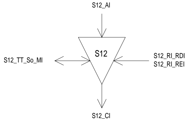
Figure 142: S12_TT_So symbol
