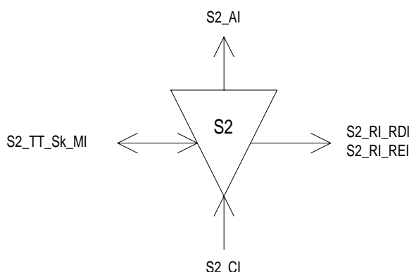
Figure 115: S2_TT_Sk symbol
