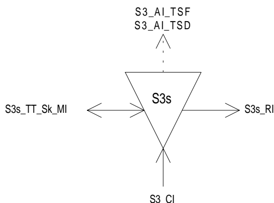
Figure 92: S3s_TT_Sk symbol
