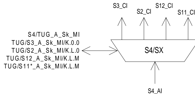
Figure 31: S4/TUG_A_Sk symbol
