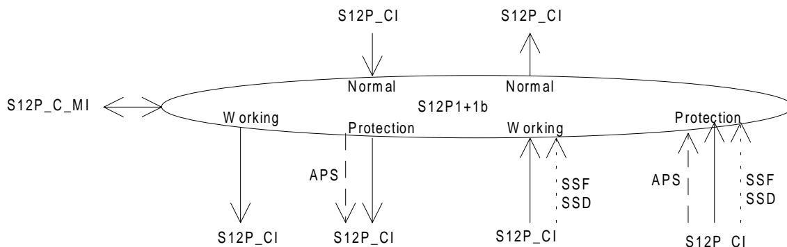
Figure 166: S12P1+1b_C symbol
