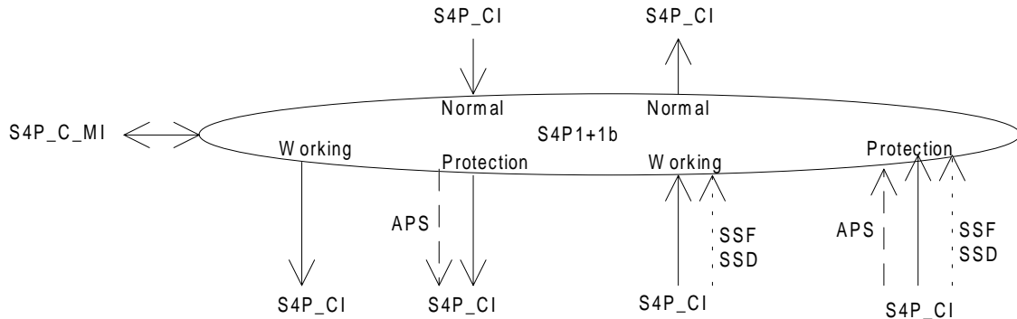
Figure 55: S4P1+1b_C symbol
