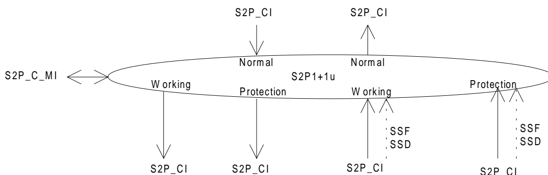
Figure 121: S2P1+1u_C symbol
