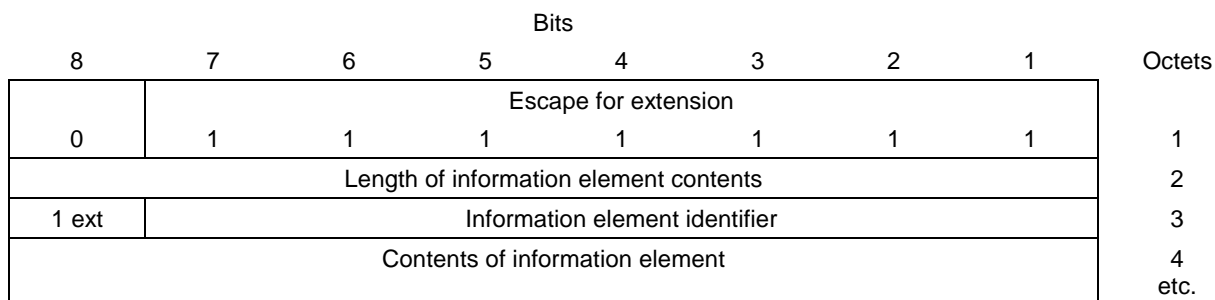
Figure 4-8: Information element format using escape for extension
