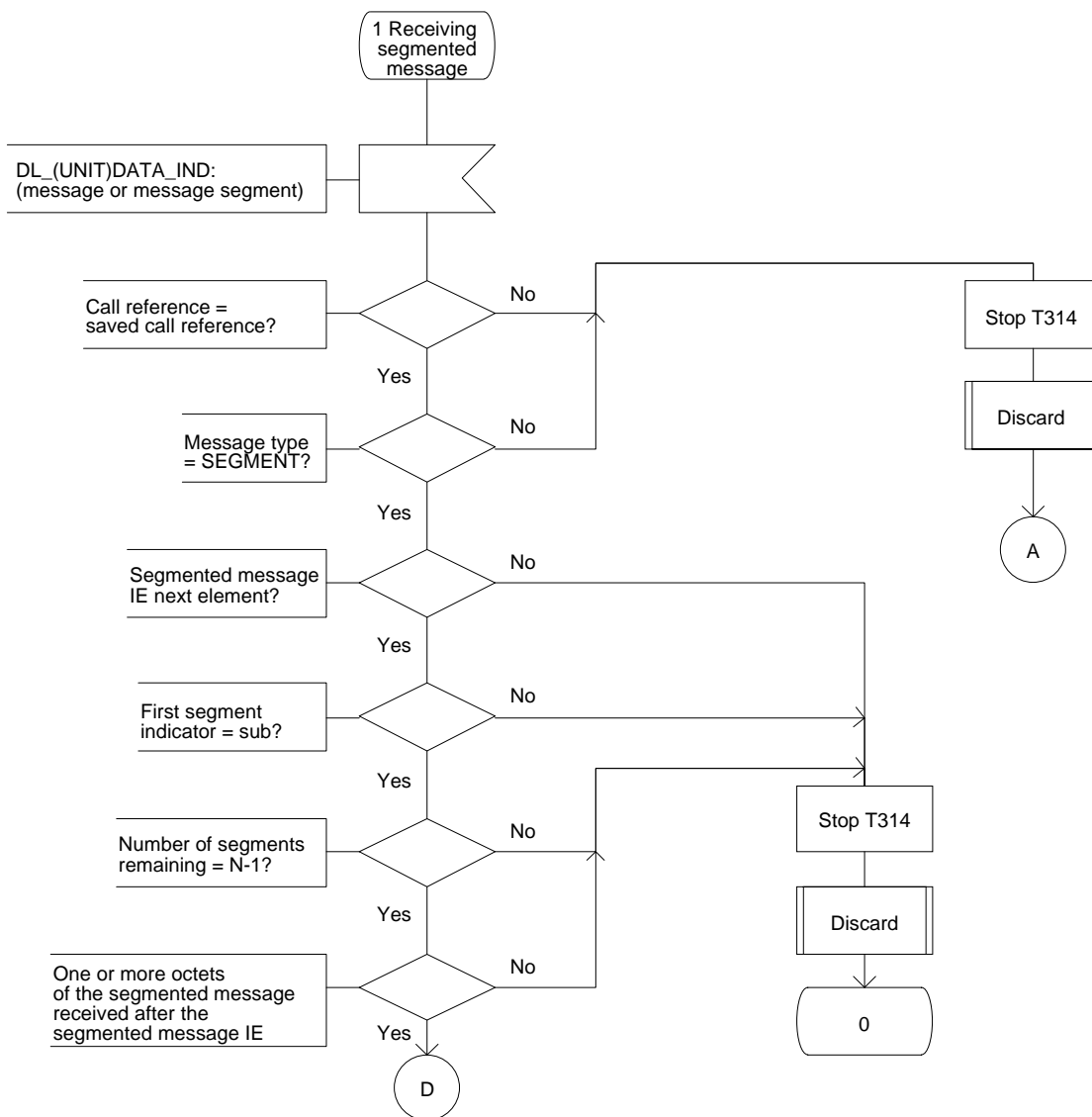
Figure H.5 (sheet 3 of 5): Message reassembler SDL
