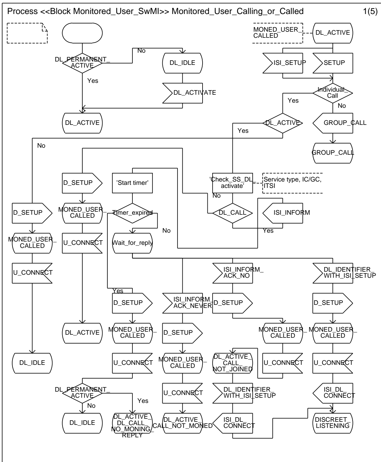
Figure A.3 (sheet 1 of 5): Monitored user visited SwMI SDL
