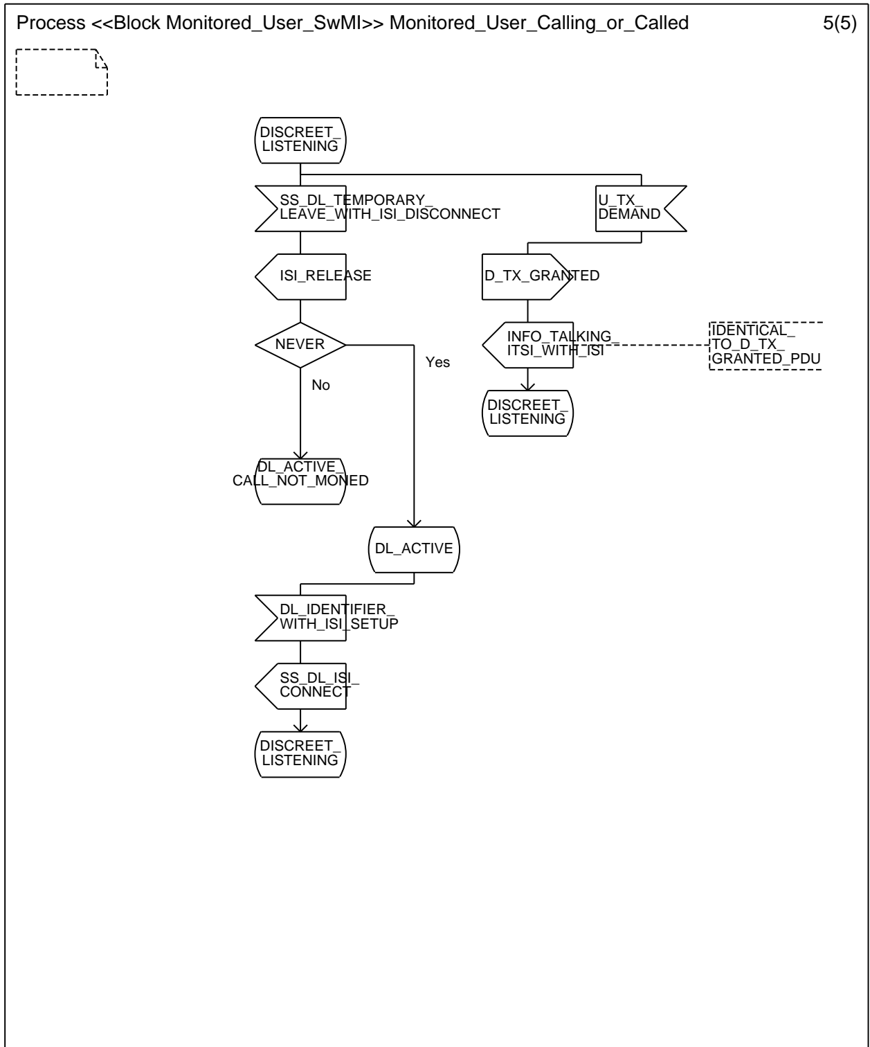
Figure A.3 (sheet 5 of 5): Monitored user registered SwMI SDL
