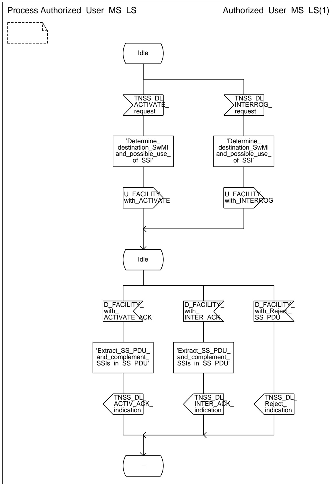
Figure A.4: SDL representation of SS-DL at the authorized user MS
