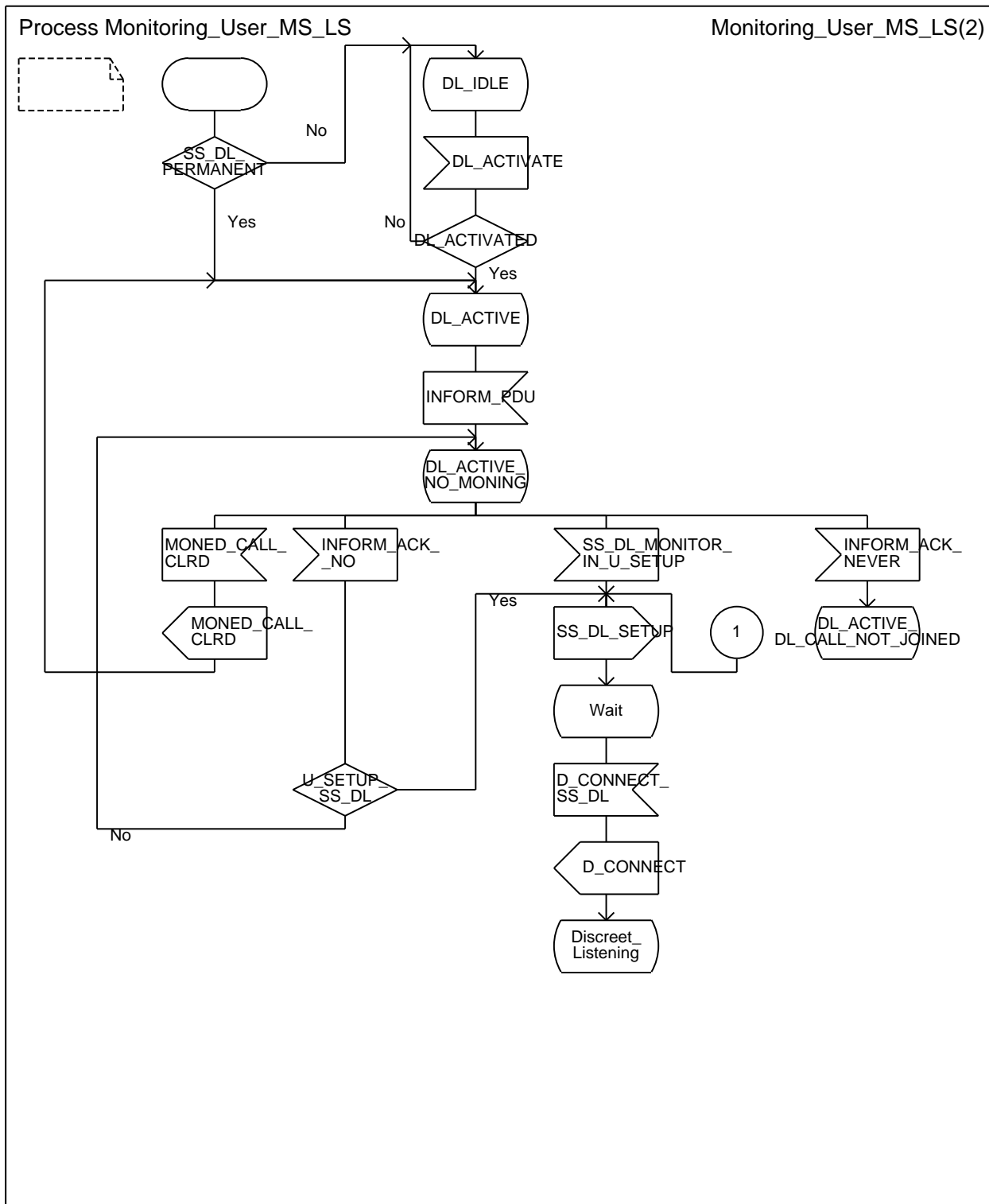
Figure A.1 (sheet 1 of 2): Monitoring user MS SDL
