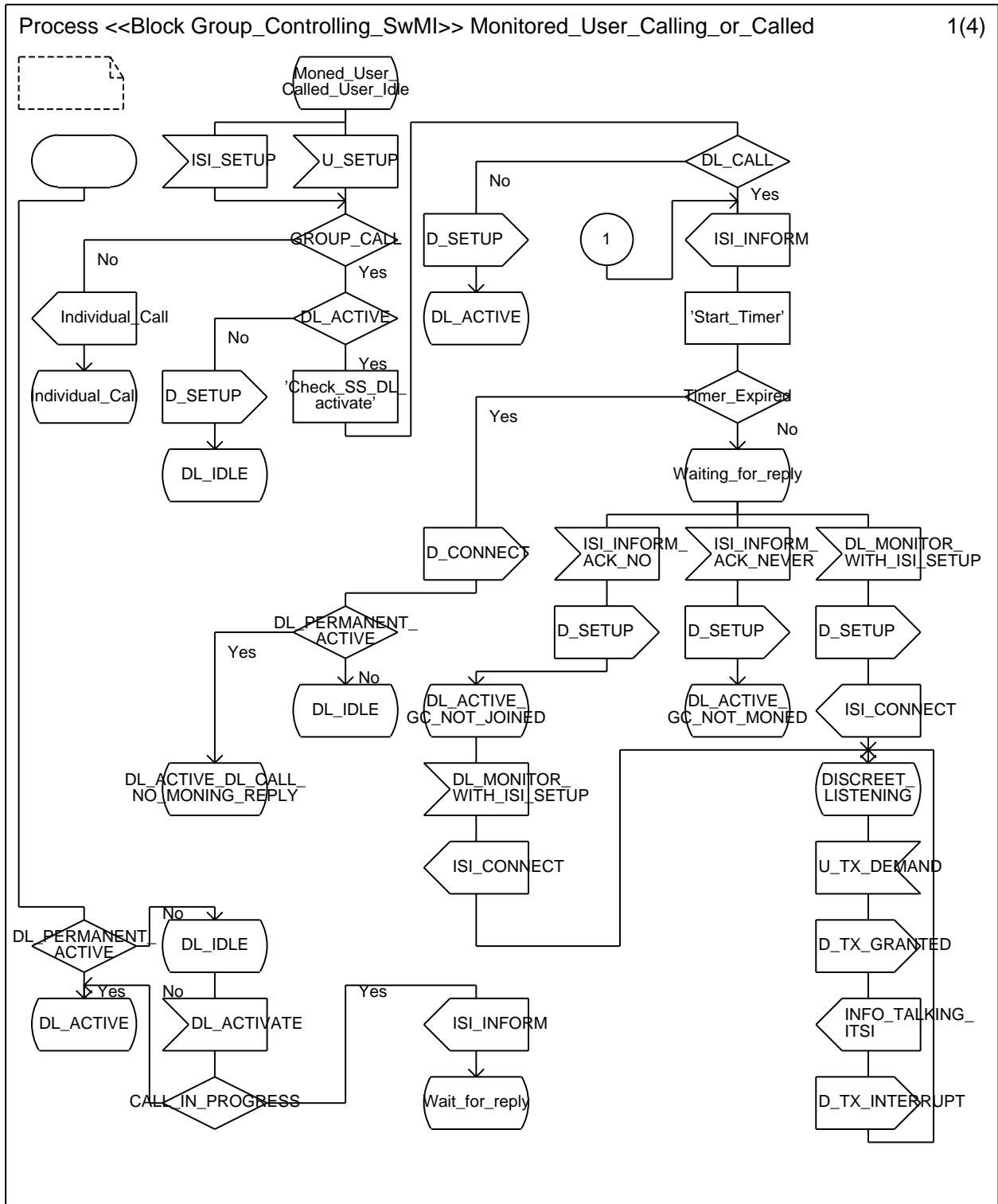
Figure A.2 (sheet 1 of 4): Group controlling SwMI SDL Monitored user is the calling user
