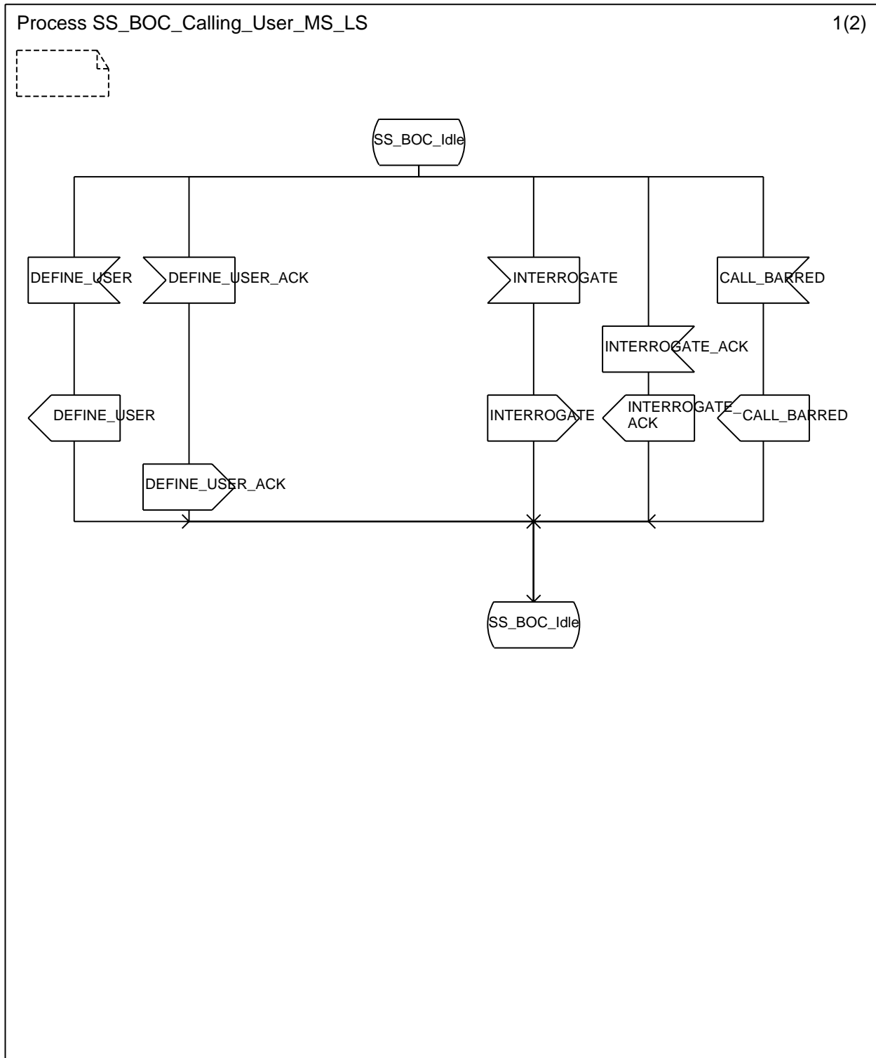
Figure A.2: SDL representations of SS-BOC at calling user home SwMI (1/2)
