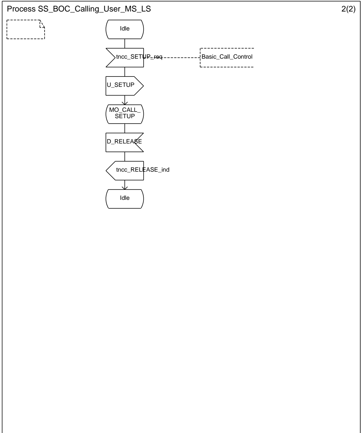
Figure A.1: SDL representations of SS-BOC at calling user MS/LS (2/2)
