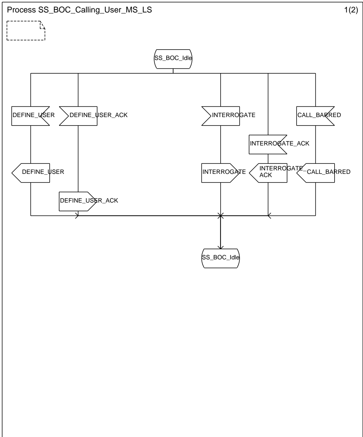
Figure A.1: SDL representations of SS-BOC at calling user MS/LS (1/2)
