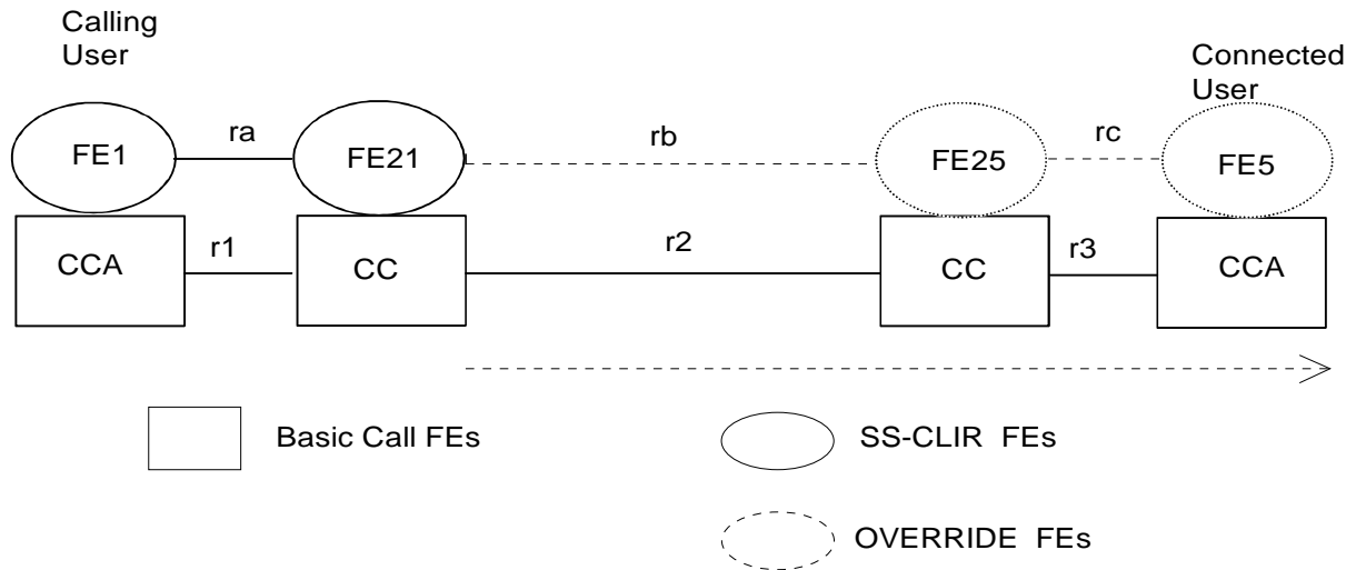
Figure 15: Example relationship between models for SS-CLIR and basic individual call
