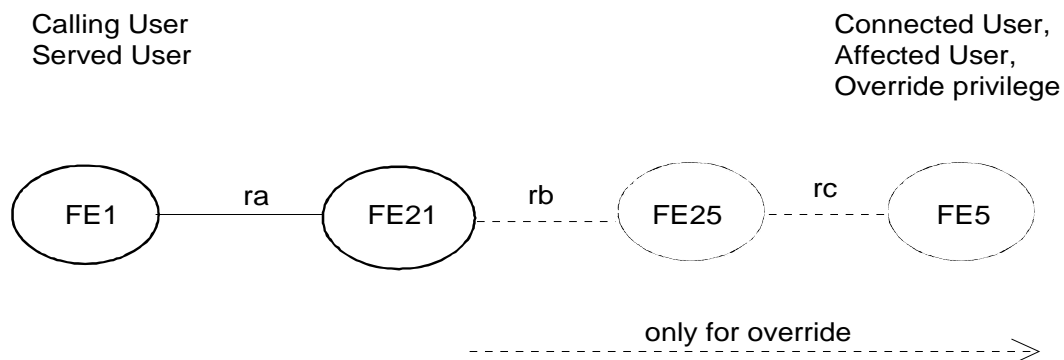
Figure 13: Functional model for SS-CLIR in case of Individual call
