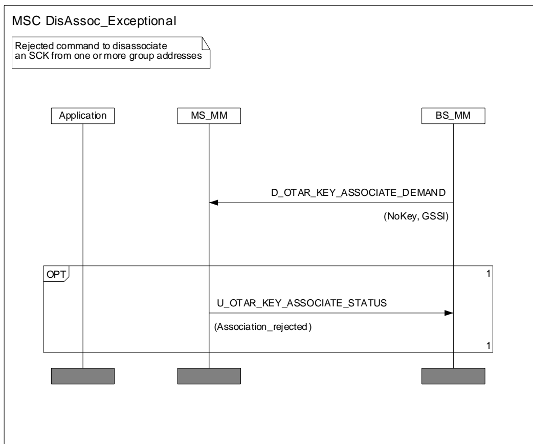
Figure 36a: Rejection of SCK disassociation
