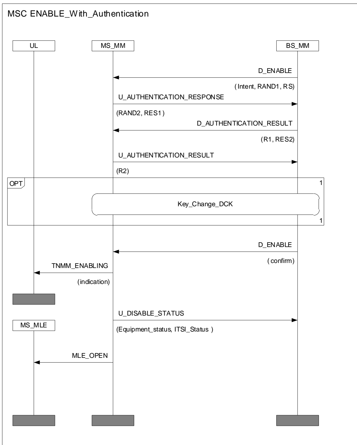
Figure 42: Enabling an MS with authentication
