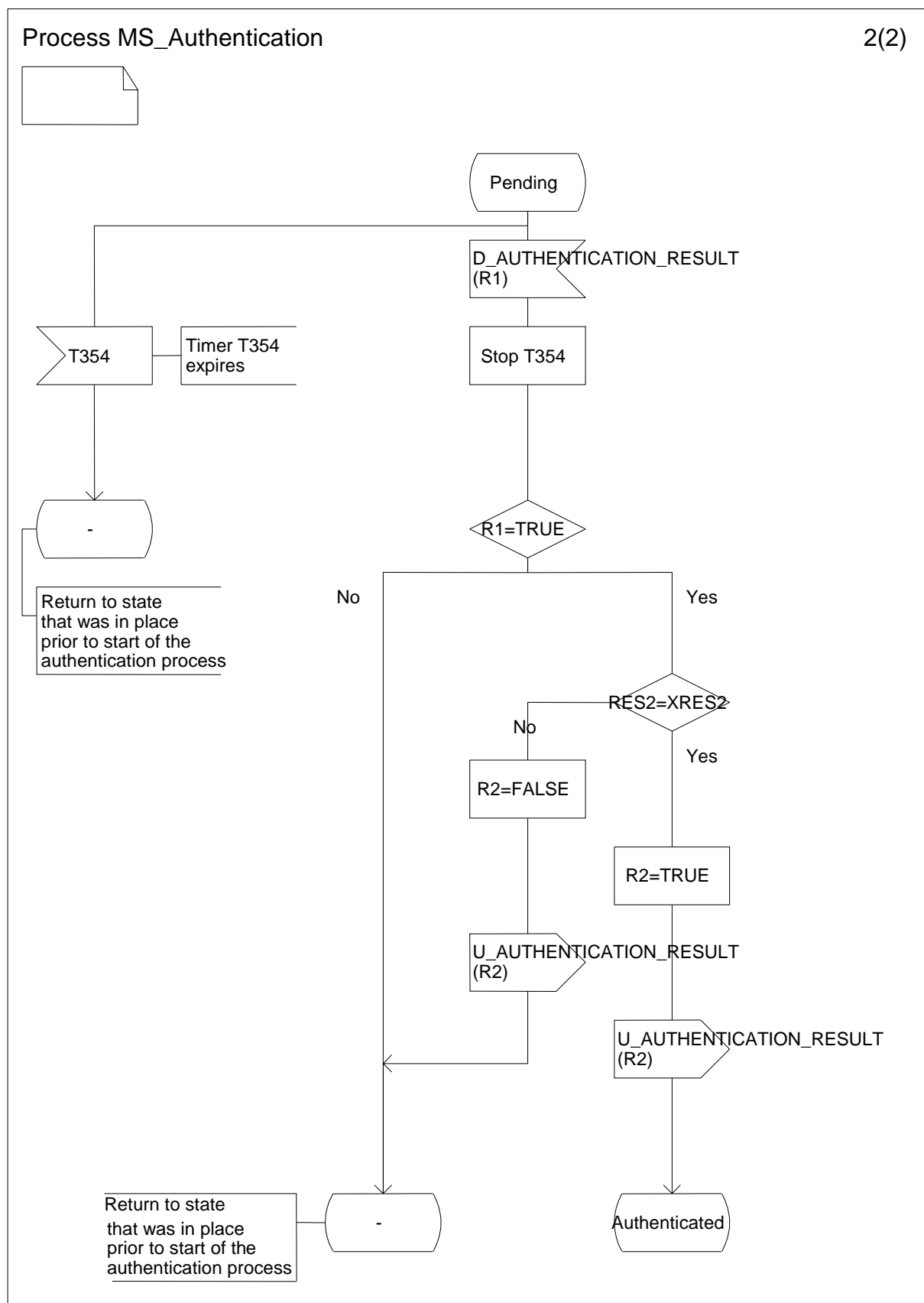
Figure 17: SDL process diagram for mutual authentication (page 2 of 2)
