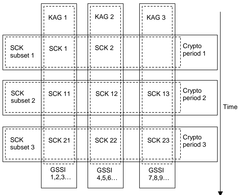
Figure 10a: Example of key association for SCK subset grouping number = 2
