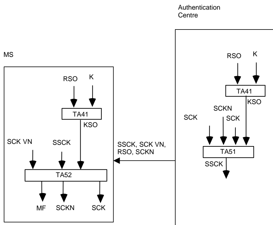
Figure 10: Distribution of SCK to an individual MS by an authentication centre
