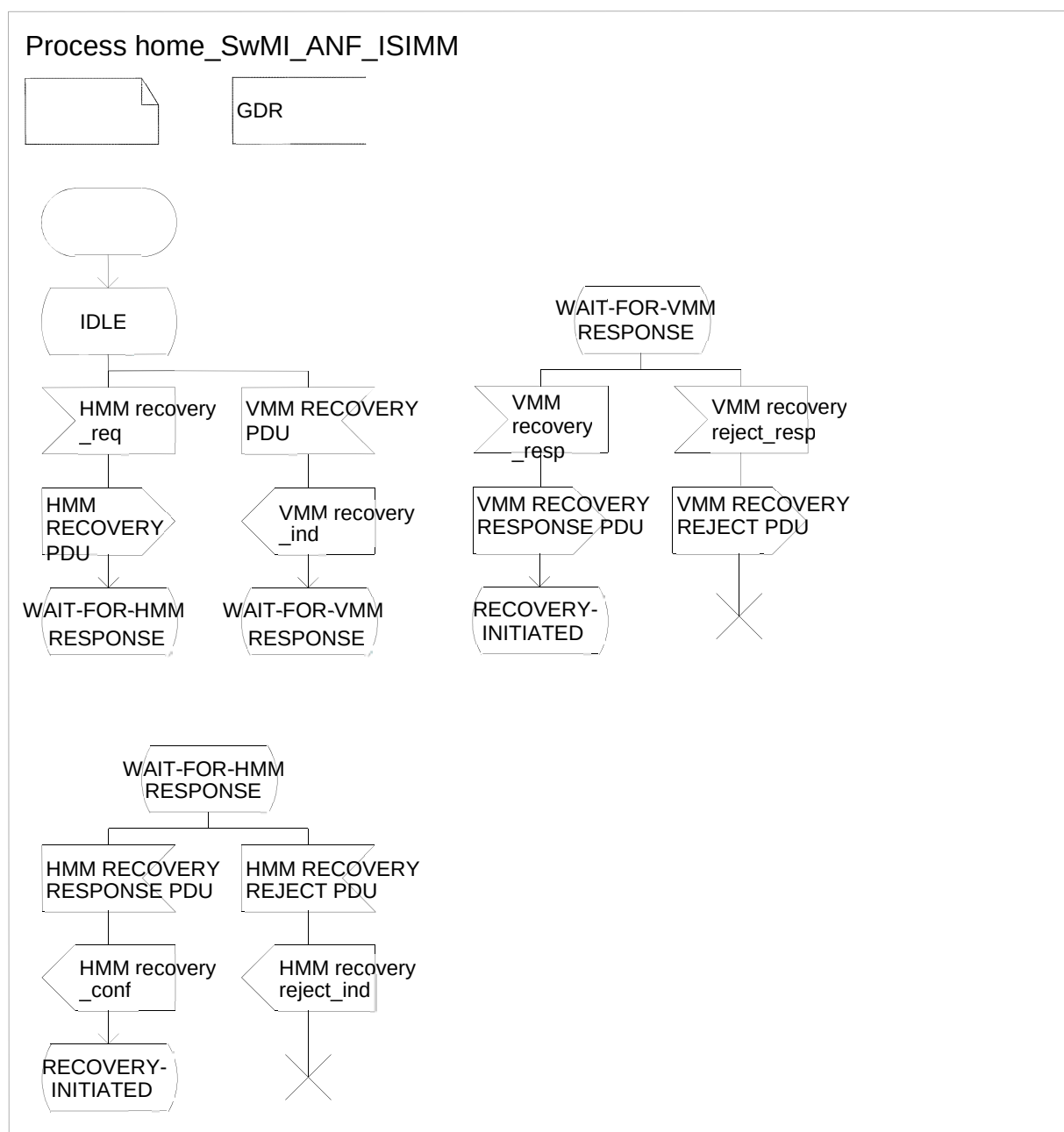
Figure 38.31: Group home SwMI ANF-ISIMM
