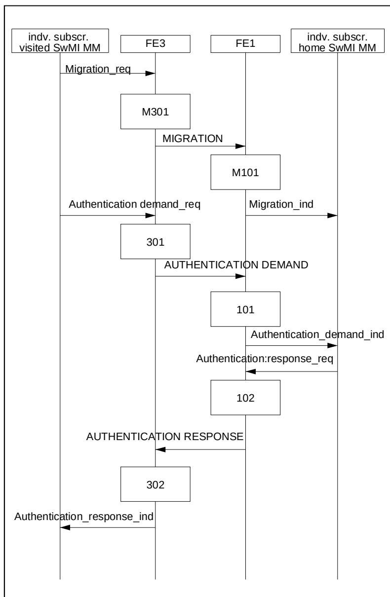
Figure 28.3: Authentication invoked in conjunction with migration (sheet 1 of 2)
