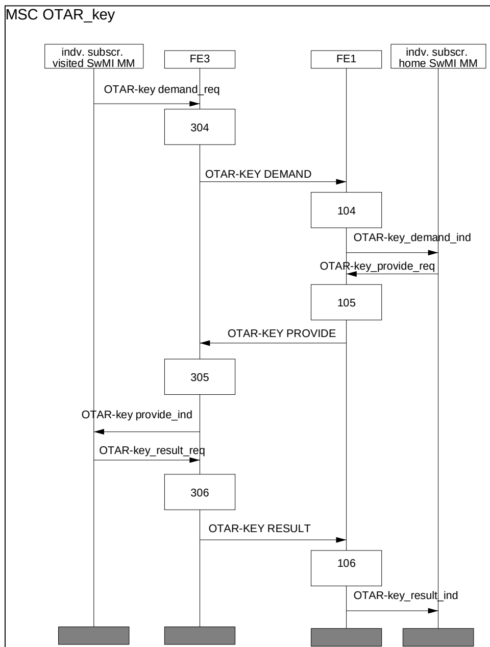
Figure 29.2: The individual subscriber visited SwMI MM initiated OTAR SCK delivery service
