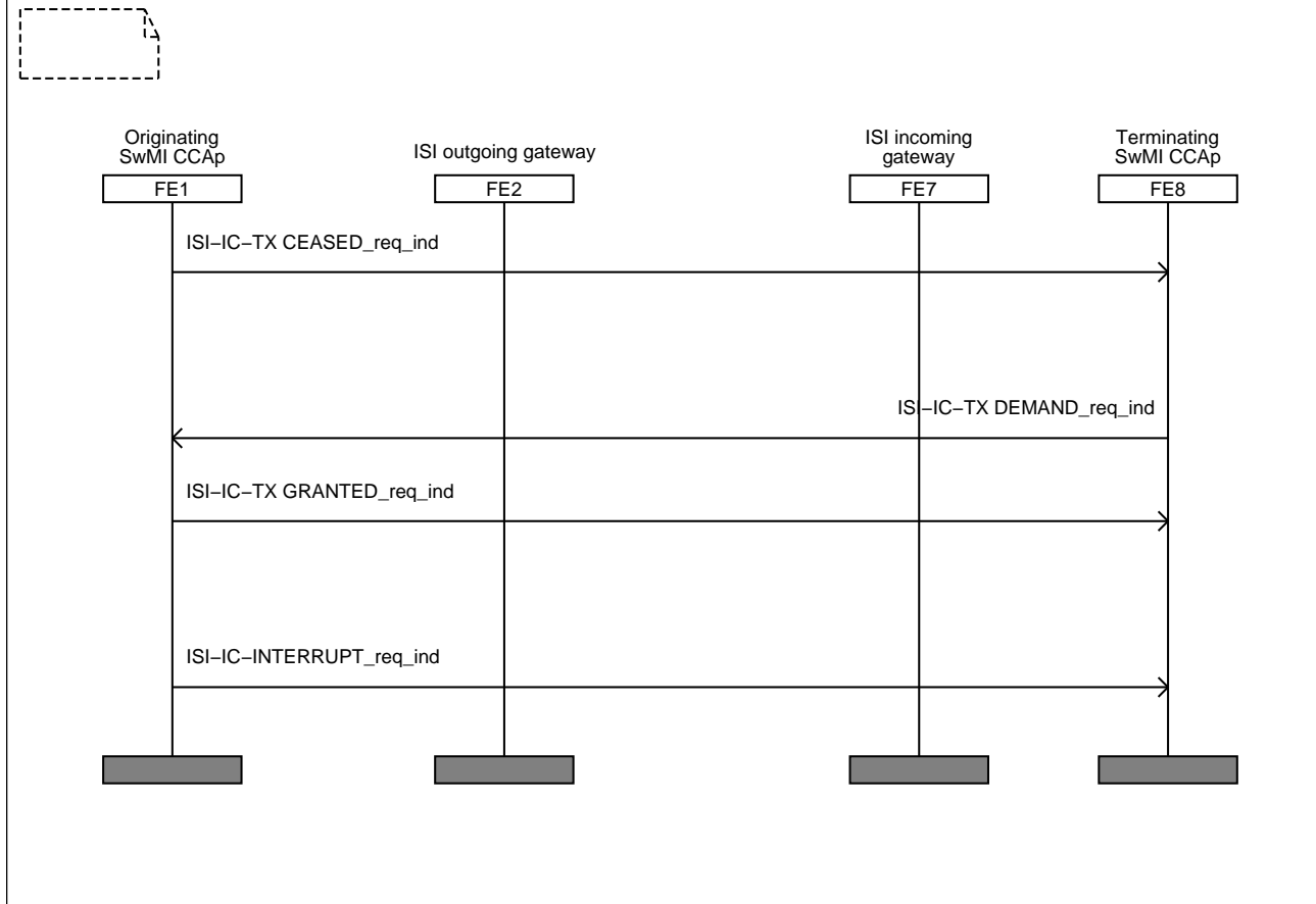
Figure 16: Information flow sequence - half-duplex operation with the called user requesting to transmit
