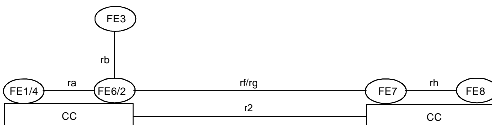
Figure 6: Example relationship between models for ANF-ISIIC and basic call in the case of called user hSwMI being SwMI A
