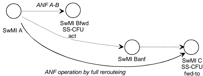
Figure C.3: Interaction with SS-CFU re-routing Forwarded-to user with home SwMI different from SwMI B, having migrated ANF operation by full re-routing
