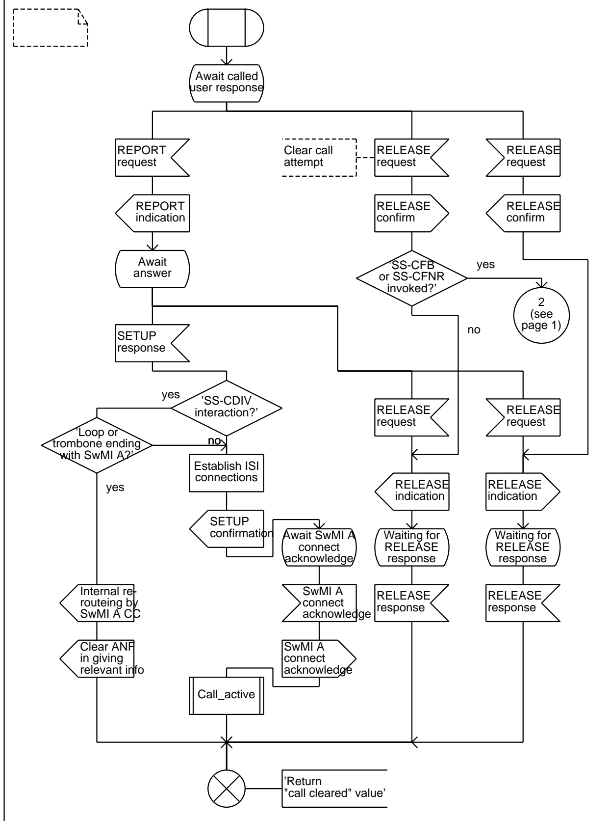
Figure 2 (sheet 3 of 5): ANF-ISIIC, overall SDL Call establishment procedure
