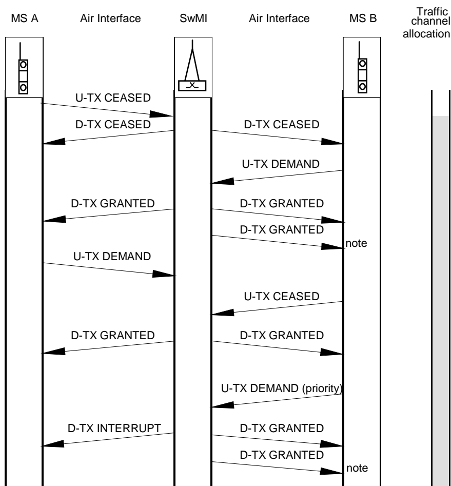
Figure E.2: Request to transmit for a group call in a message trunked system
