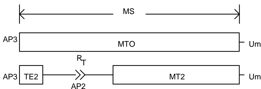
Figure A.4: MS access to a TETRA LMN
