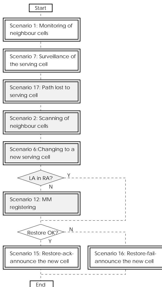
Figure H.23: Unannounced cell re-selection
