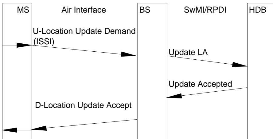
Figure G.3: Registration at accepted roaming, with no authentication nor identity exchange
