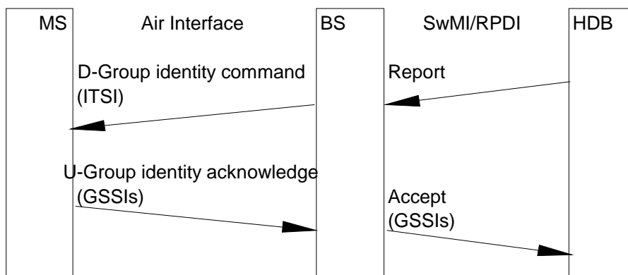
Figure G.22: Reporting current group identities (GSSI) to the network
