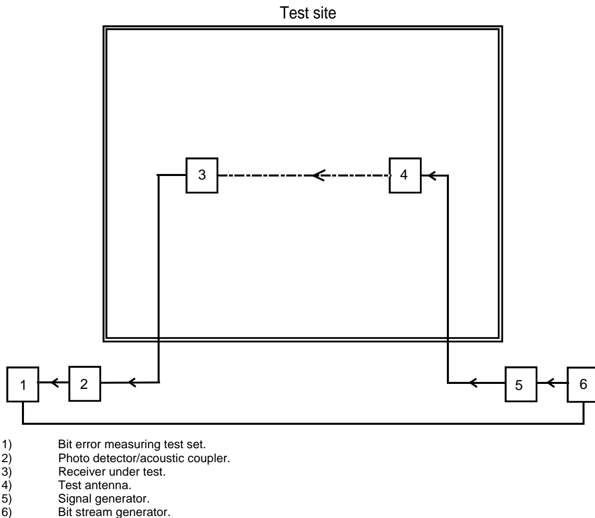
Figure 14: Measurement arrangement
