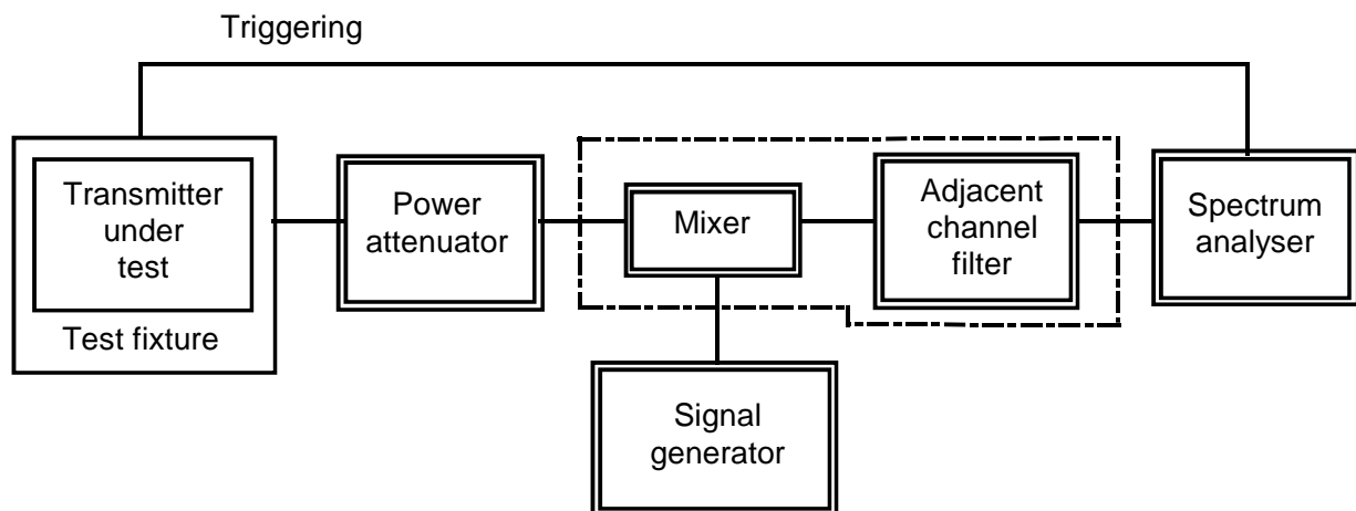
Figure 13: Adjacent channel transient power measuring device measurement arrangement
