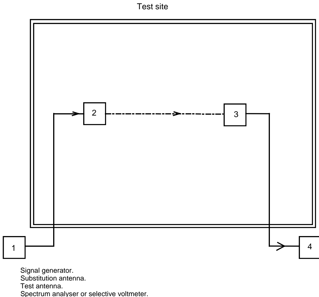
Figure 4: Measurement arrangement
