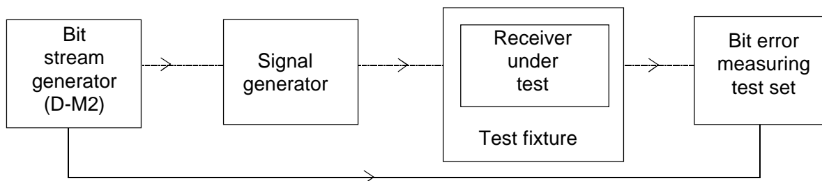
Figure 18: Measurement arrangement
