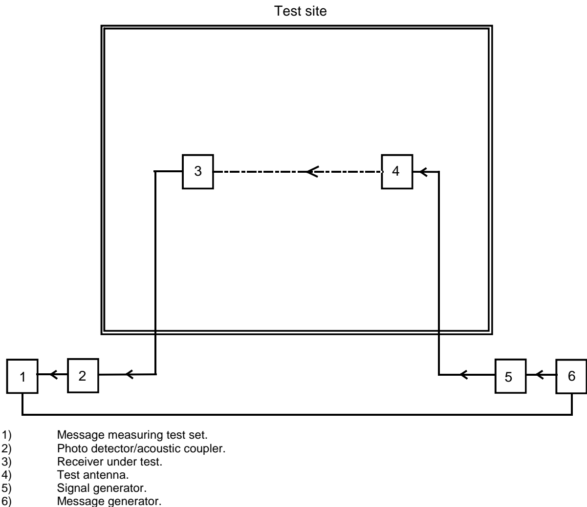
Figure 16: Measurement arrangement
