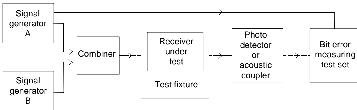
Figure 22: Measurement arrangement
