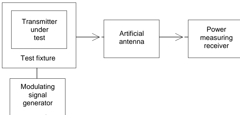
Figure 6: Measurement arrangement
