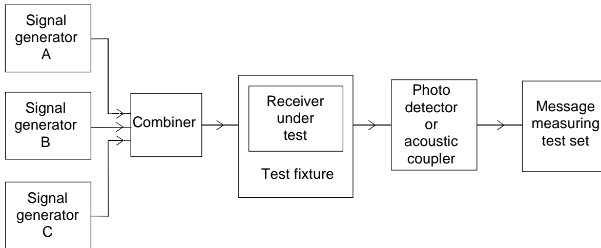
Figure 26: Measurement arrangement
