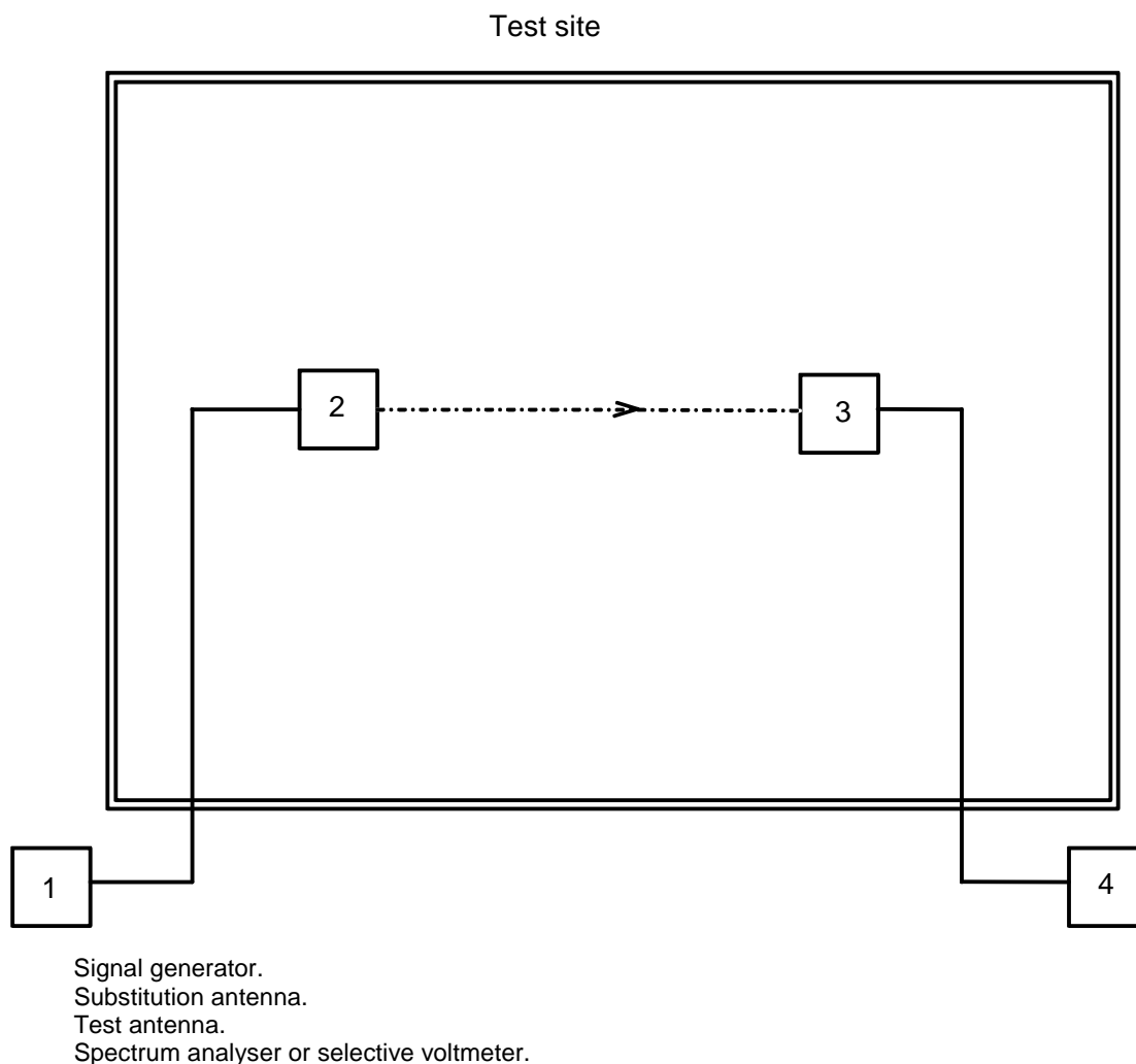
Figure 30: Measurement arrangement
