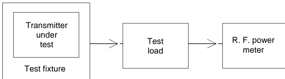
Figure 5: Measurement arrangement
