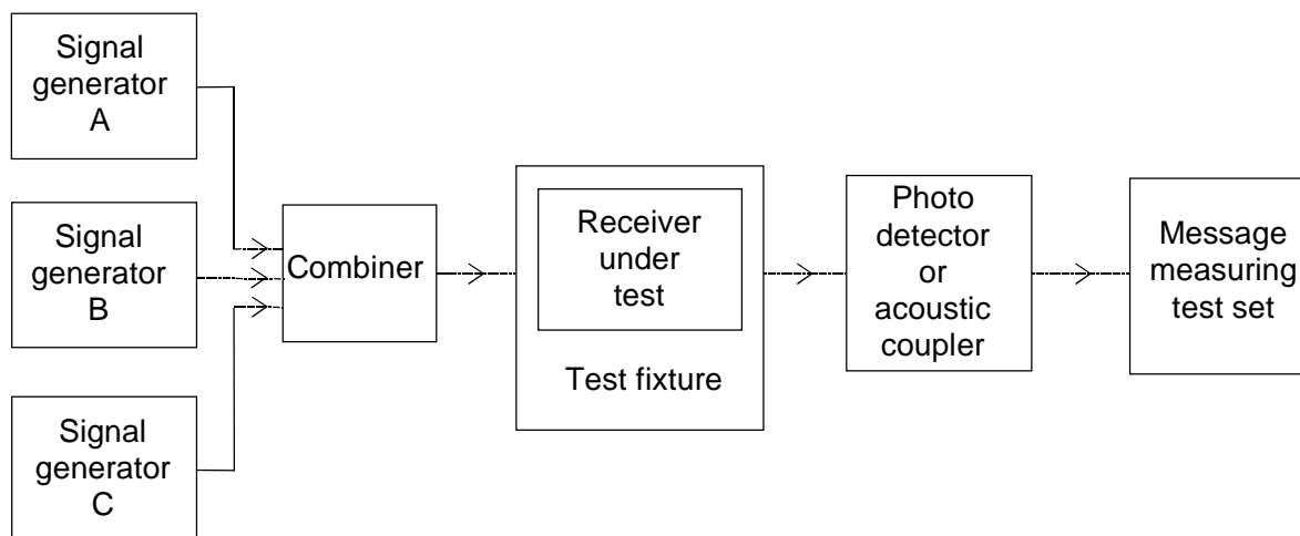
Figure 25: Measurement arrangement
