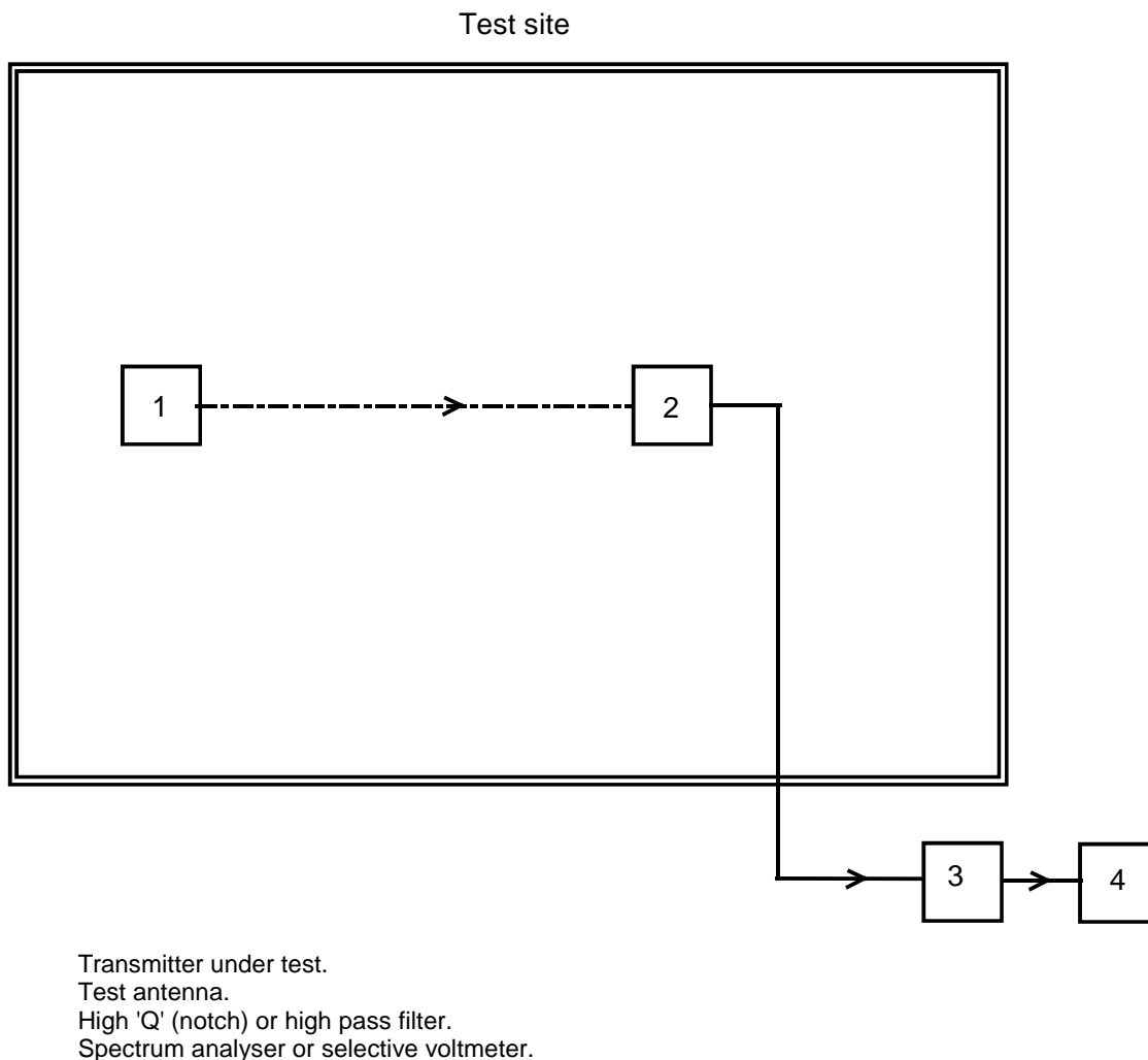
Figure 7: Measurement arrangement
