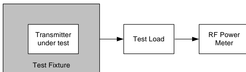
Figure 6: Measurement arrangement
