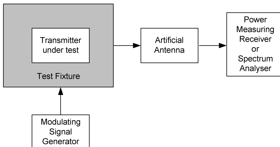
Figure 7: Measurement arrangement
