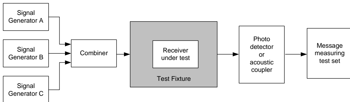
Figure 26: Measurement arrangement
