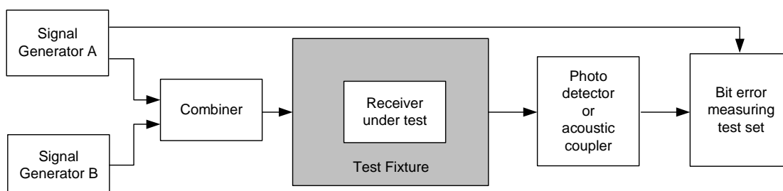
Figure 21: Measurement arrangement
