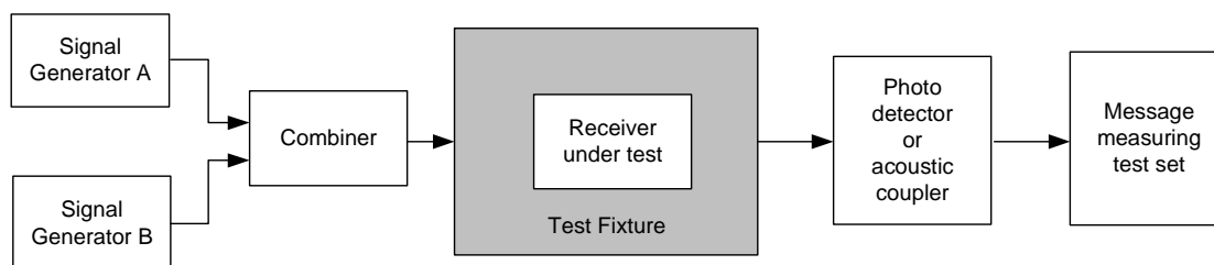
Figure 24: Measurement arrangement
