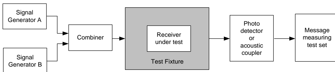
Figure 22: Measurement arrangement
