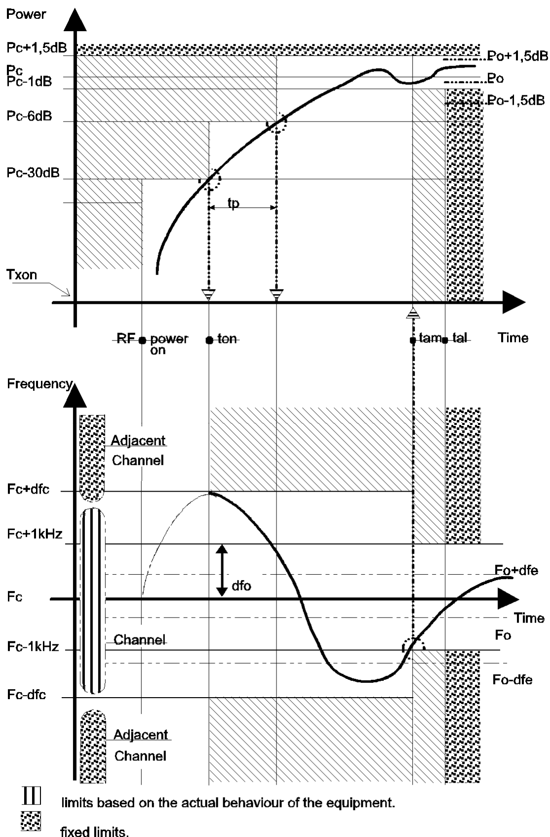
Figure 11: Transmitter attack time according to clause 7.5.1 b) and transient behaviour during switch-on (case where the attack time is given by the behaviour of the frequency)
