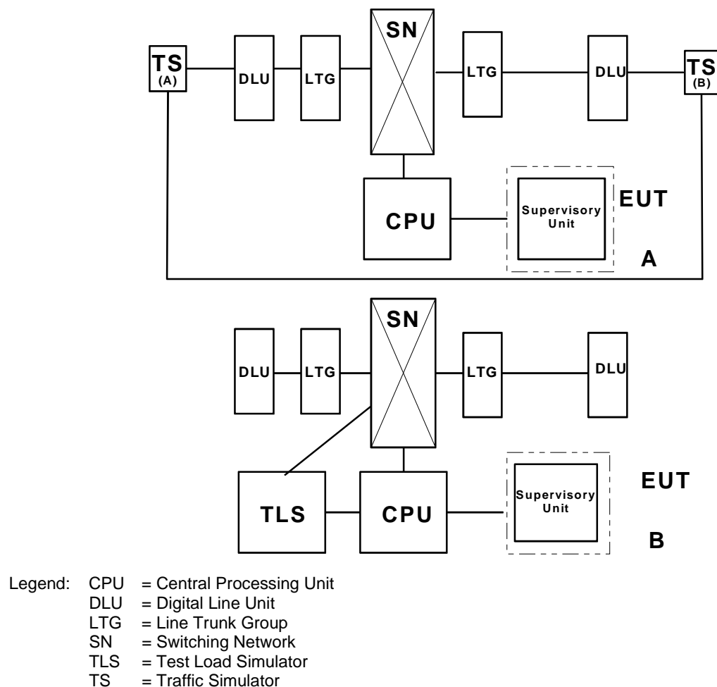
Figure 6: Two examples for the configuration of the EUT and exercising equipment
