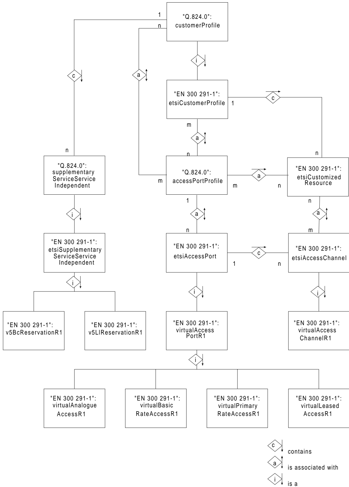
Figure 5: Relation to EN 300 291-1 - customer administration
