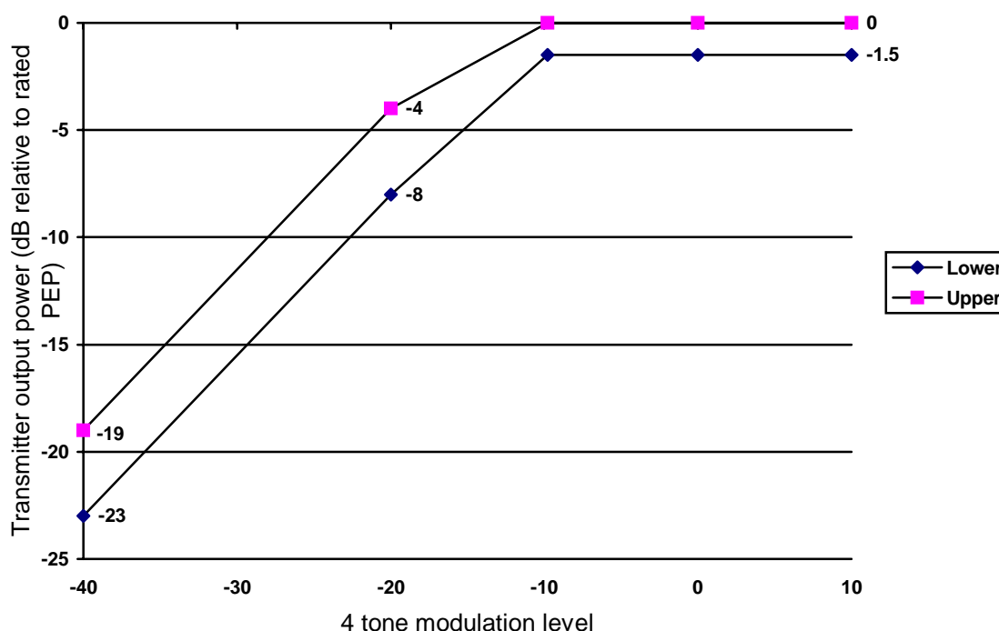
Figure 4: Limits of telephony level control
