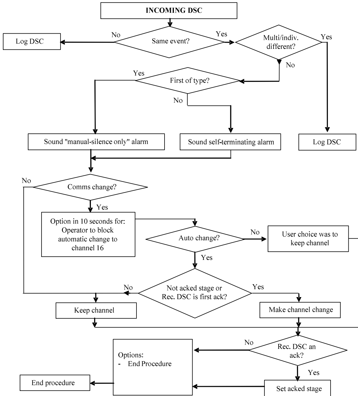
Figure 2: Receiving distress procedure
