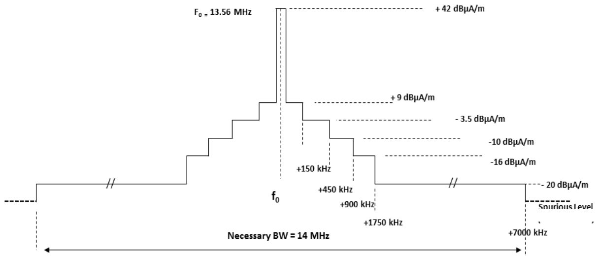
Figure G.3: Spectrum mask limit for wideband RFIDs in the 13,56 MHz range
