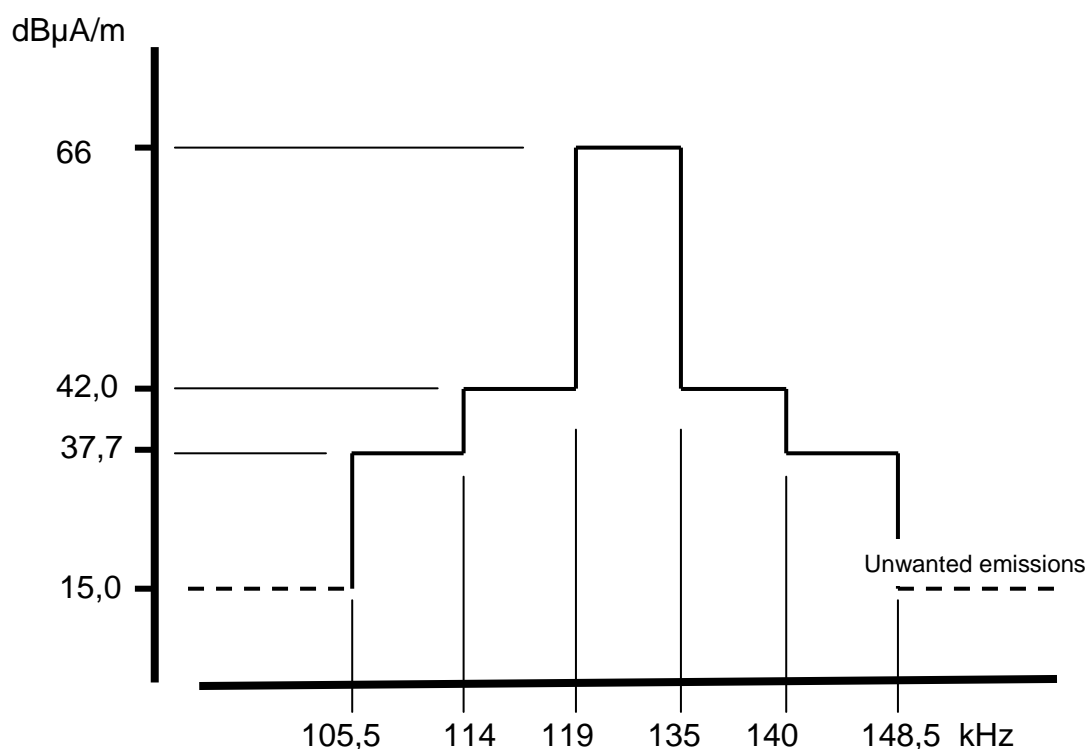
Figure G.1: Emission boundary for LF RFID systems
