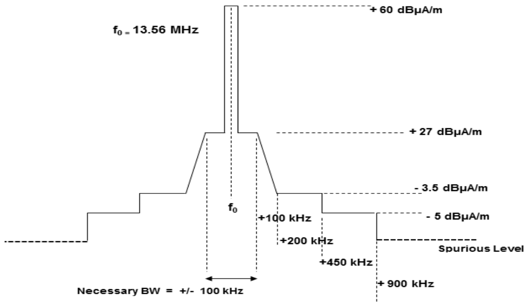
Figure G 4: Spectrum mask limit for narrowband RFIDs in the 13,56 MHz range
