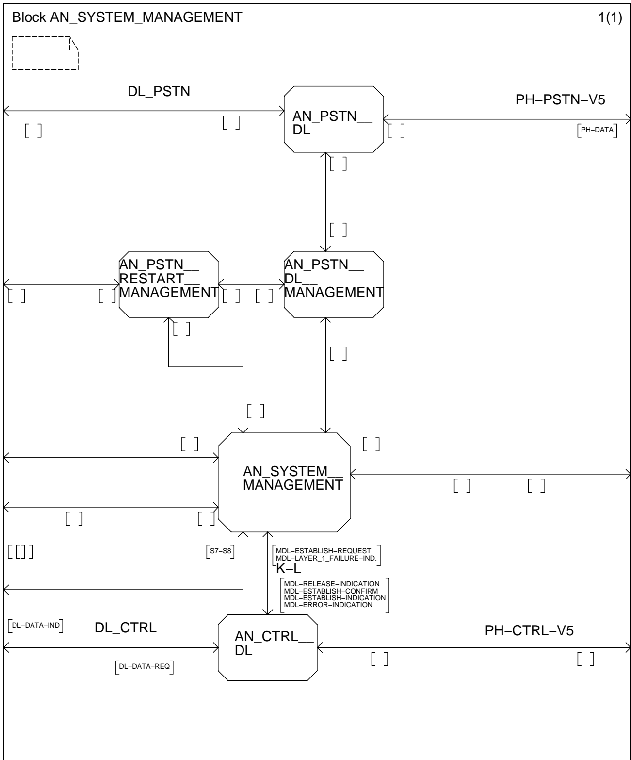
Figure L.6: System management block description AN-side
