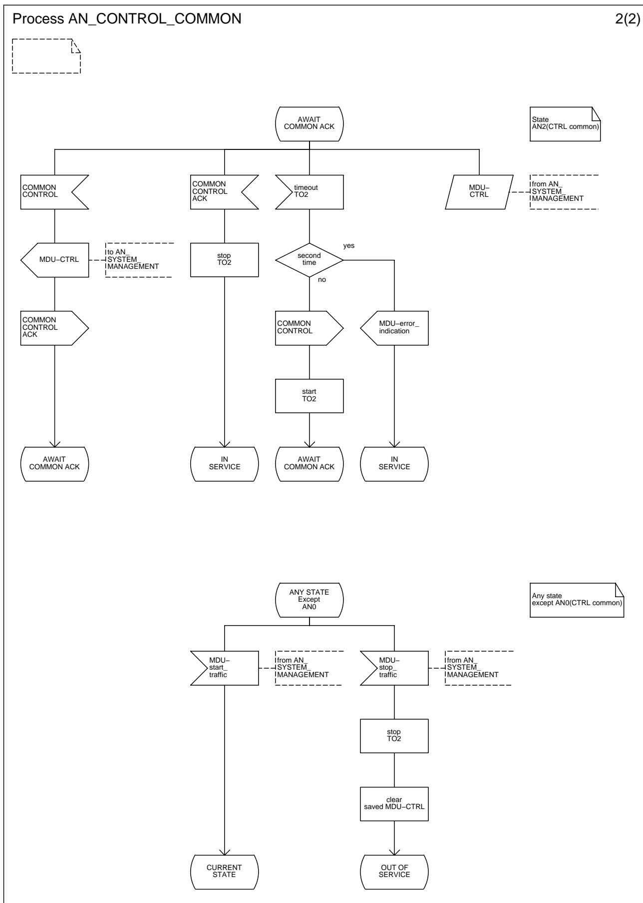
Figure L.12.2: Common control protocol AN-side; state AWAIT COMMON ACK (AN2(CTRL common)) and any state except AN0(CTRL common)
