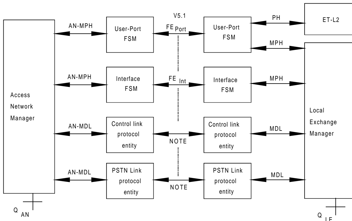
Figure 4: L1 and L2 FSM functional model
