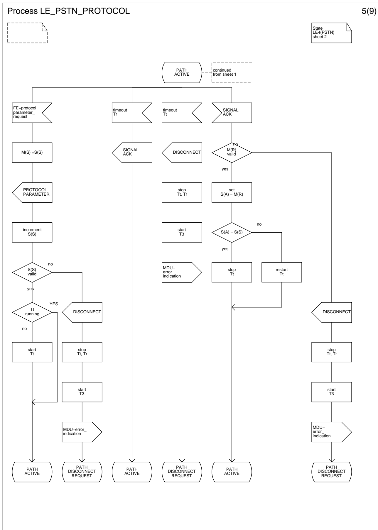
Figure L.25.5: PSTN protocol LE-side; state PATH ACTIVE (LE4(PSTN)) (sheet 2)
