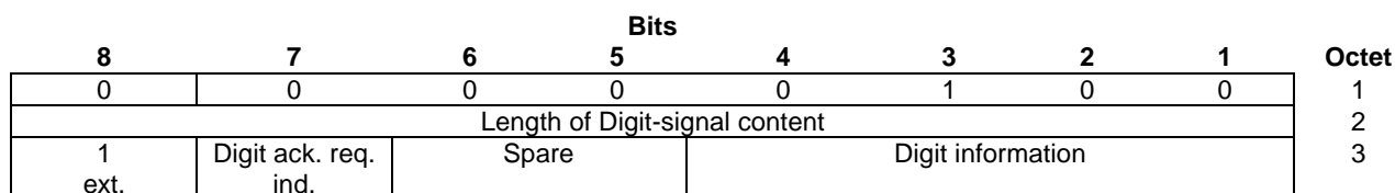
Figure 24: Digit-signal information element
