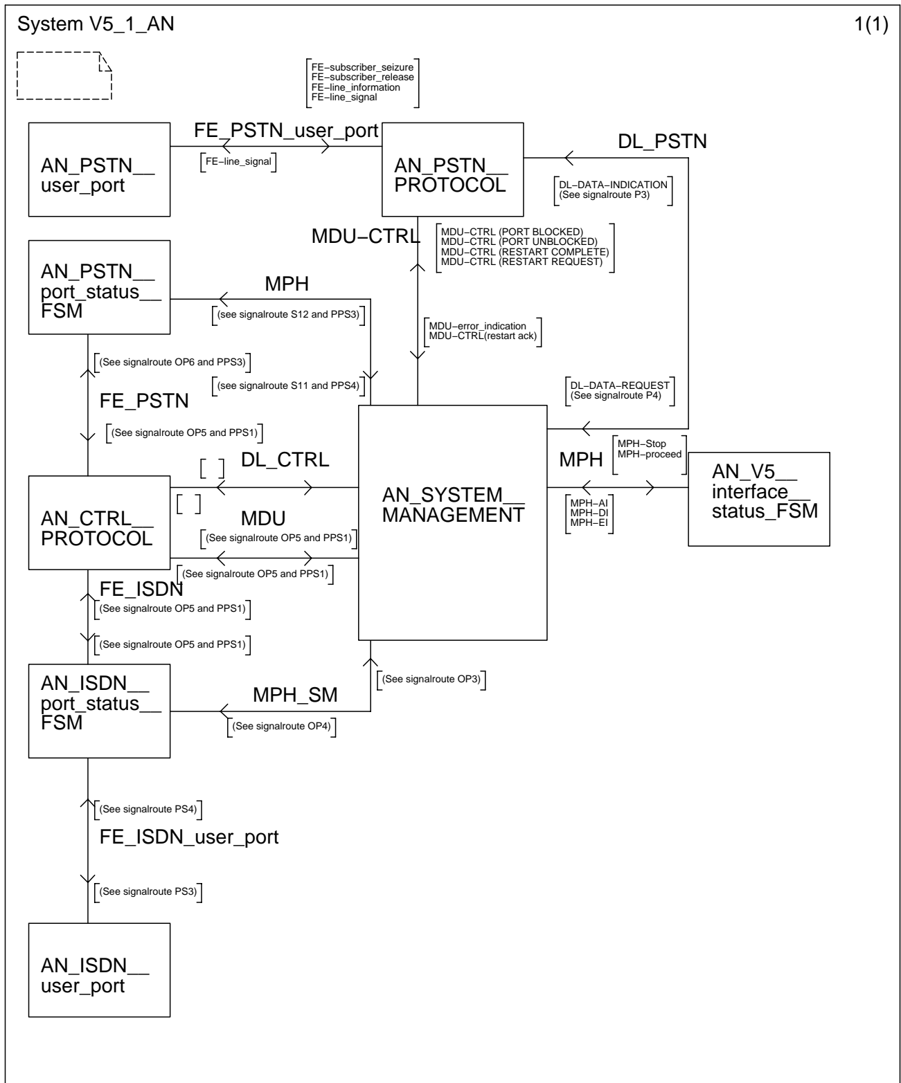
Figure L.1: V5.1 system overview AN-side
