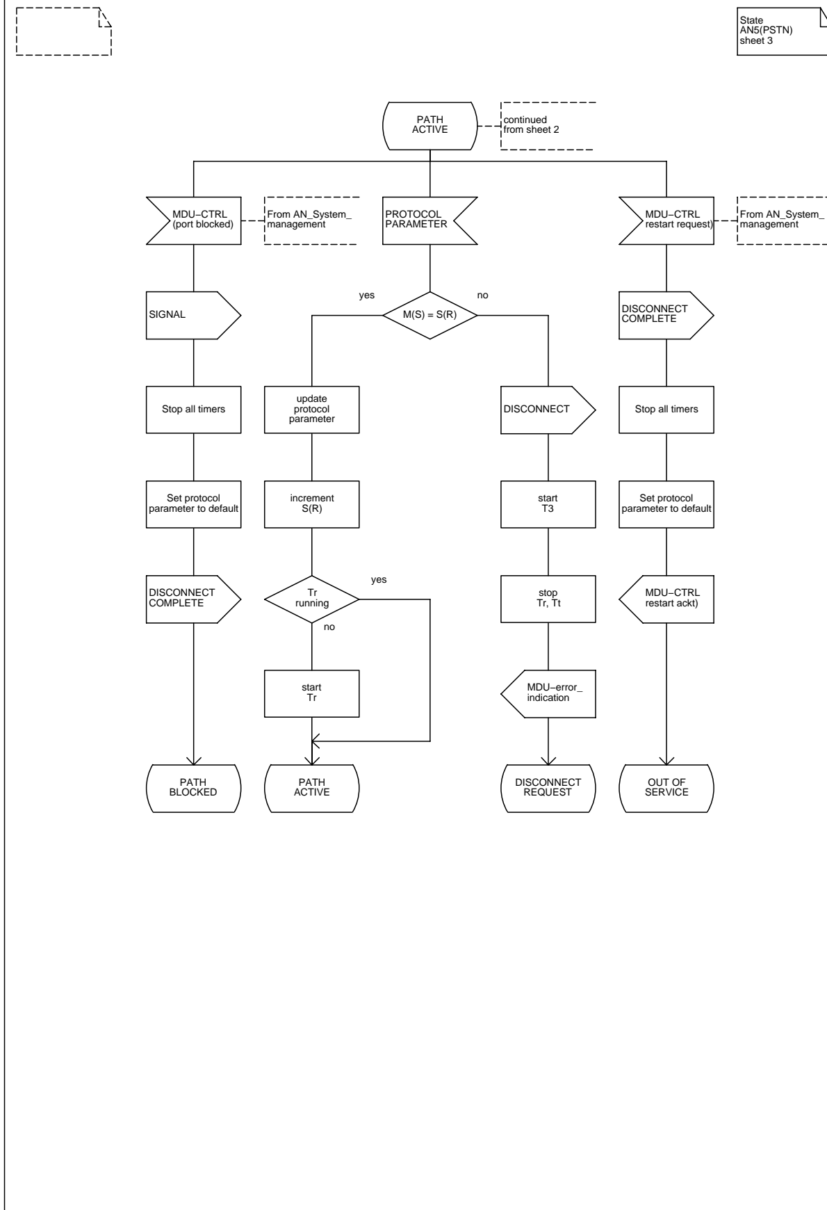
Figure L.9.8: PSTN protocol AN-side; state PATH ACTIVE (AN5(PSTN)) (sheet 3 of 3)
