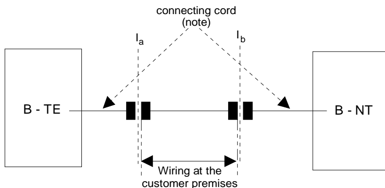
Figure 5: Wiring configuration
