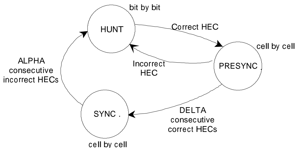
Figure 12: Cell delineation state diagram
