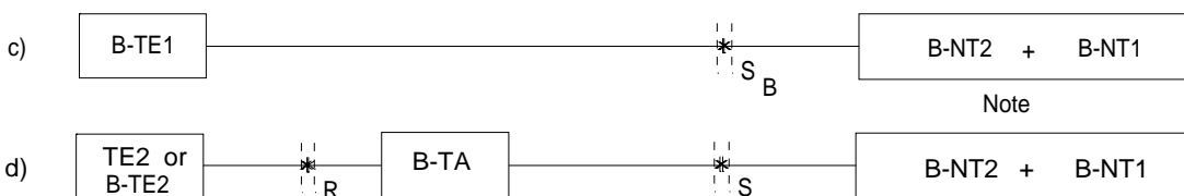
Configurations where B-ISDN physical interfaces occur at reference point S_B only
