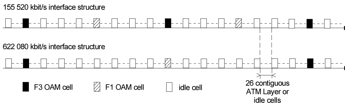
Figure 9: Interface structure
