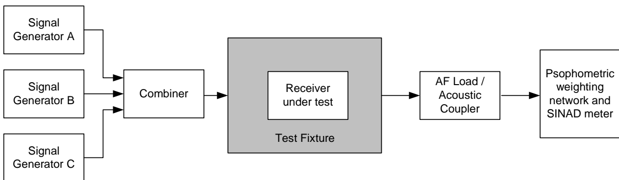
Figure 18: Measurement arrangement
