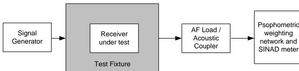
Figure 12: Measurement arrangement
