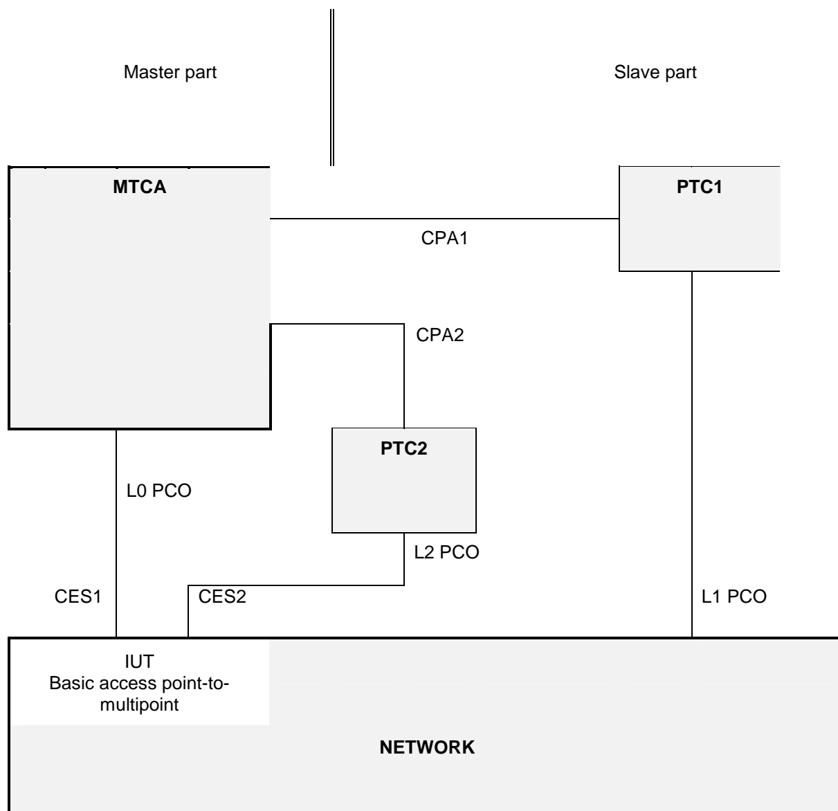
Figure 3: Multi-party test method - modified for point-to-multipoint configurations
