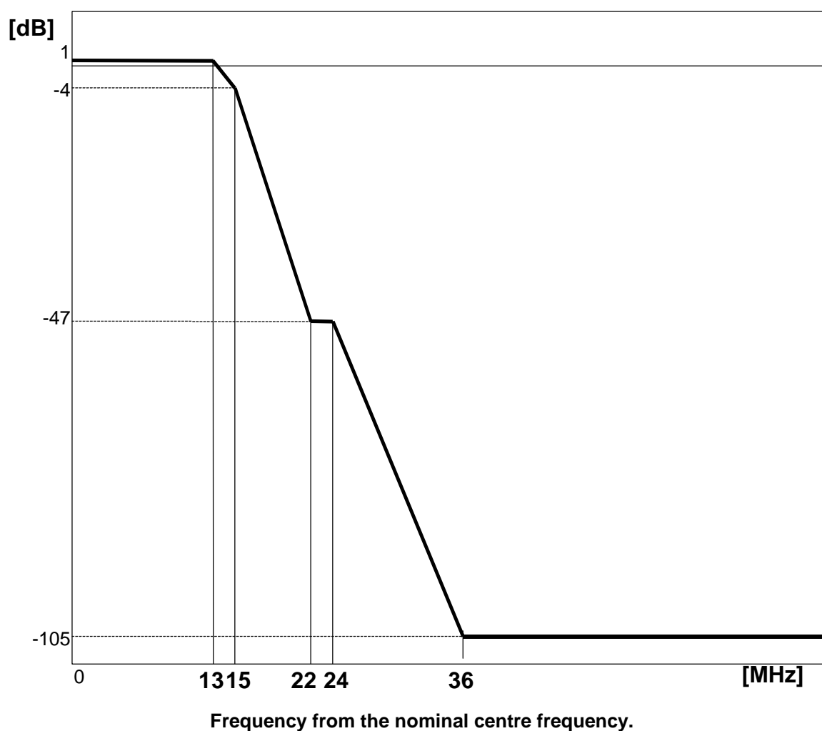
Figure 8: Overall minimum receiver selectivity of the inner side of innermost receiver for L6 GHz band (class 5 Grade A) with compatibility requirements, see clause 4.2
