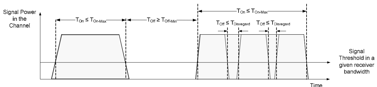
Figure 4: Transmission definitions
