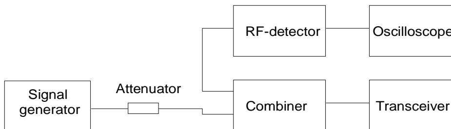
Figure 4: Measurement arrangement
