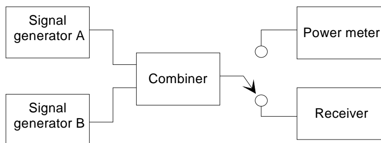
Figure 8: Measurement arrangement
