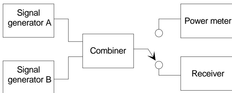
Figure 5: Measurement arrangement
