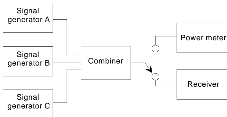
Figure 7: Measurement arrangement
