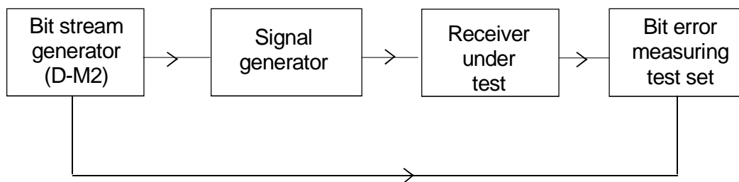
Figure 2: Measurement arrangement
