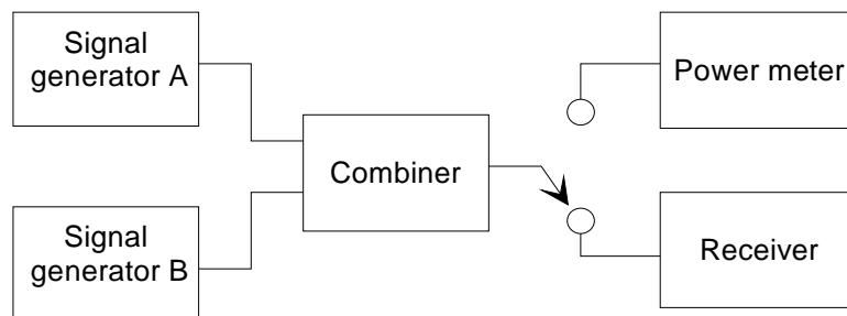
Figure 6: Measurement arrangement
