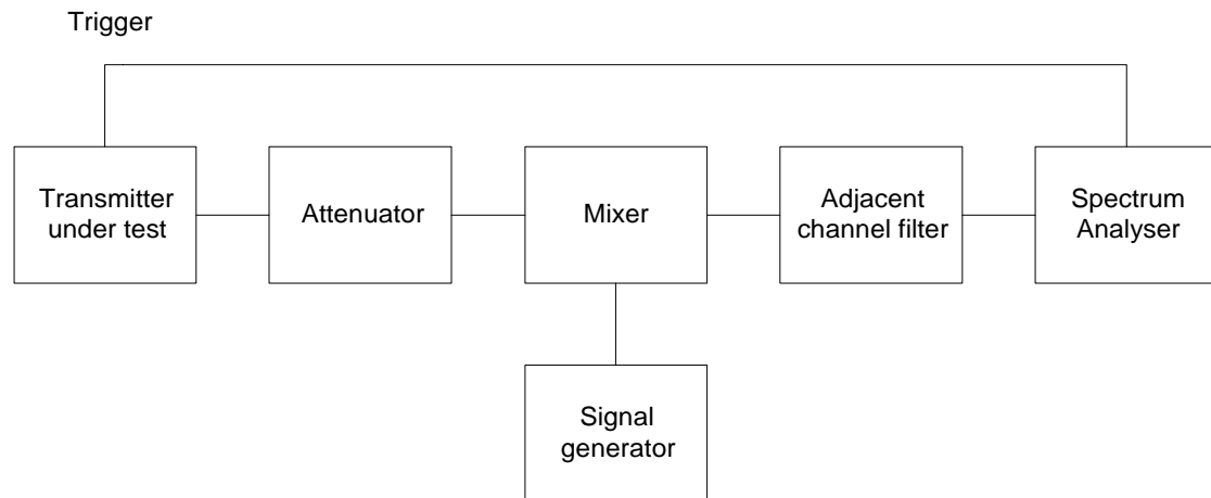
Figure 1: An example of a transient power measuring device measurement arrangement
