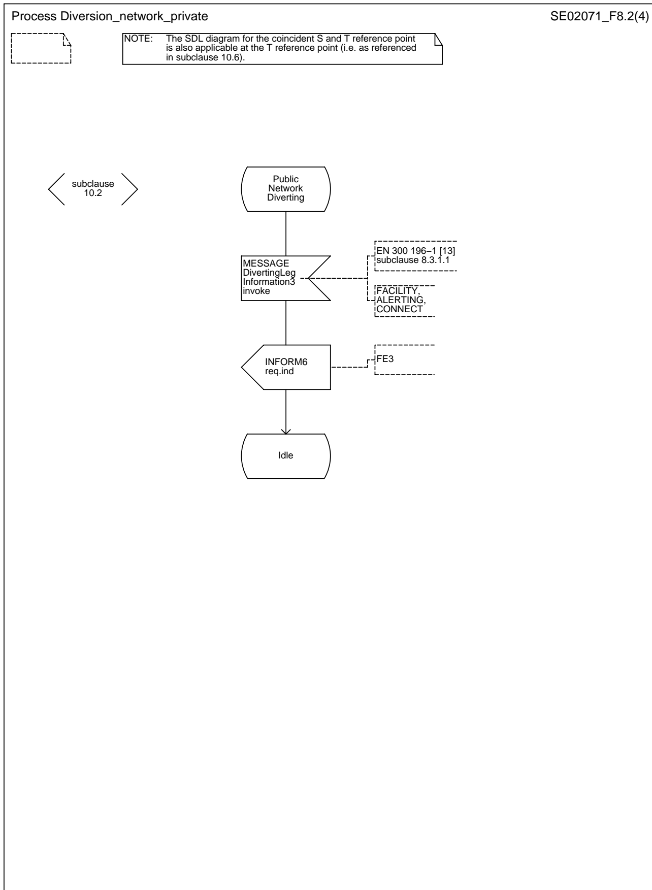
Figure 8 (sheet 2 of 4): Network at the T reference point
