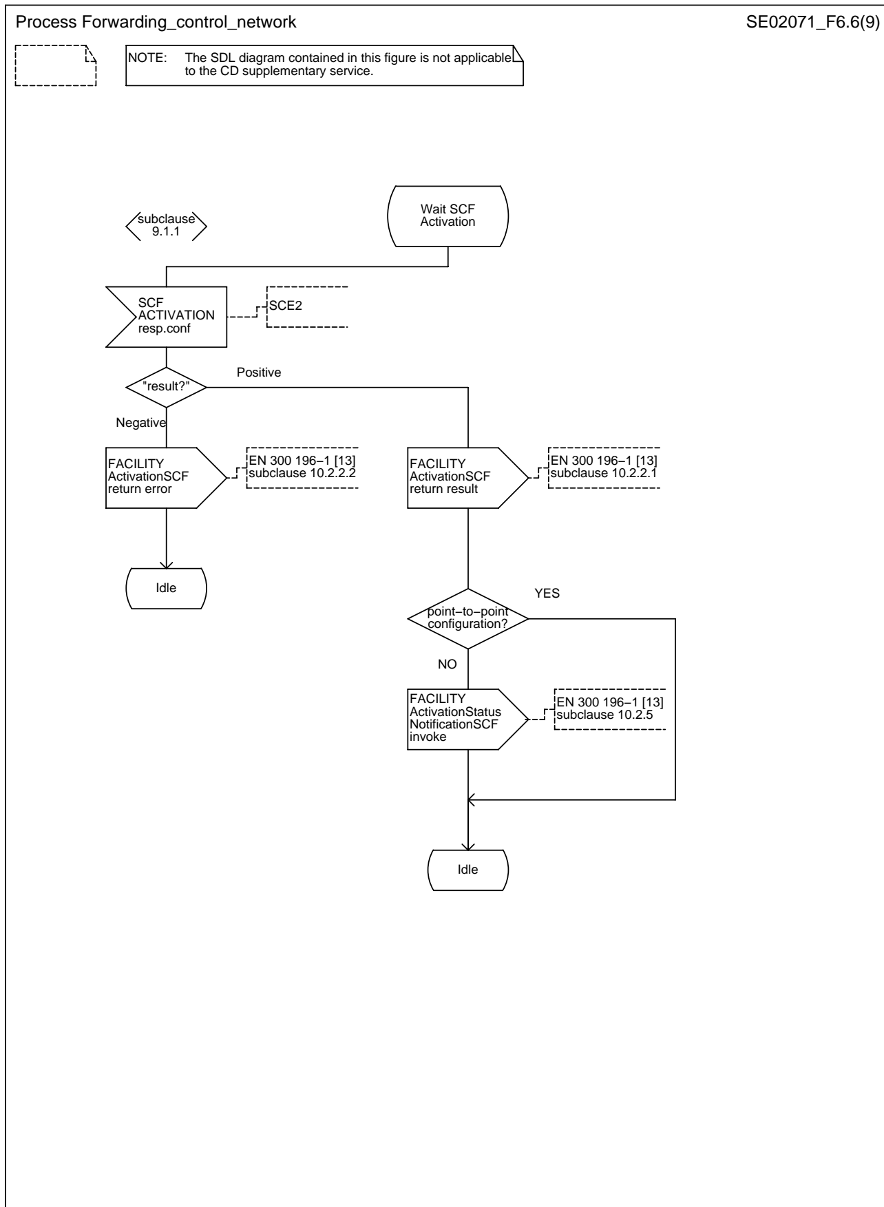
Figure 6 (sheet 6 of 9): Network at the coincident S and T reference point
