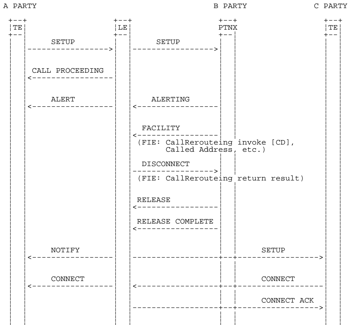
Figure A.4: Partial rerouting requested by the PTNX, triggered in case of CD alerting, early release, in the PTNX
