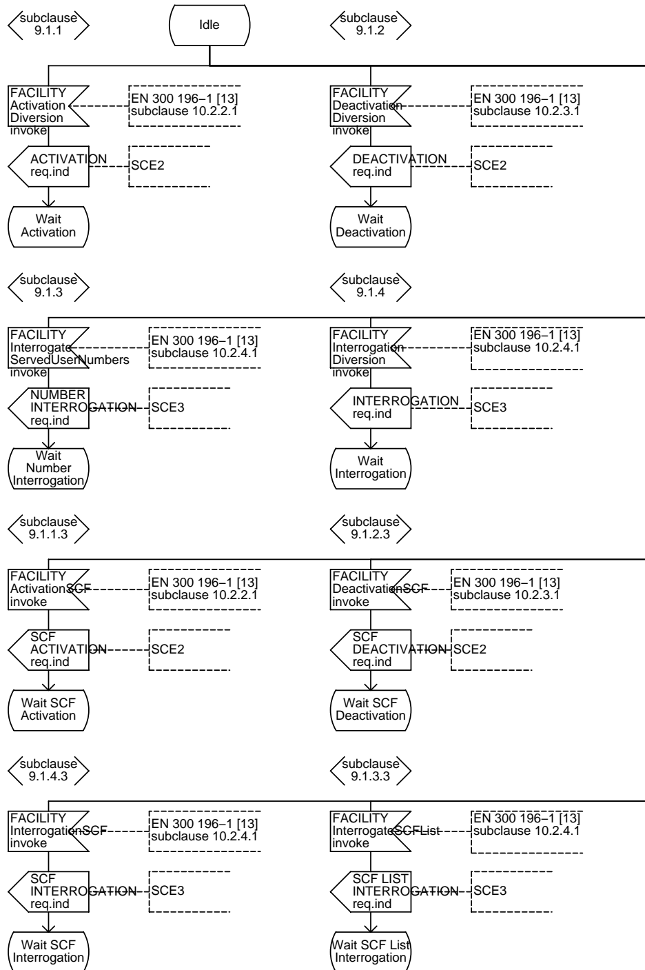
Figure 6 (sheet 1 of 9): Network at the coincident S and T reference point
