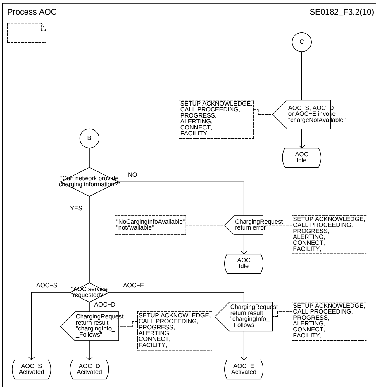
Figure 3 (sheet 2 of 2): Network side - AOC Idle
