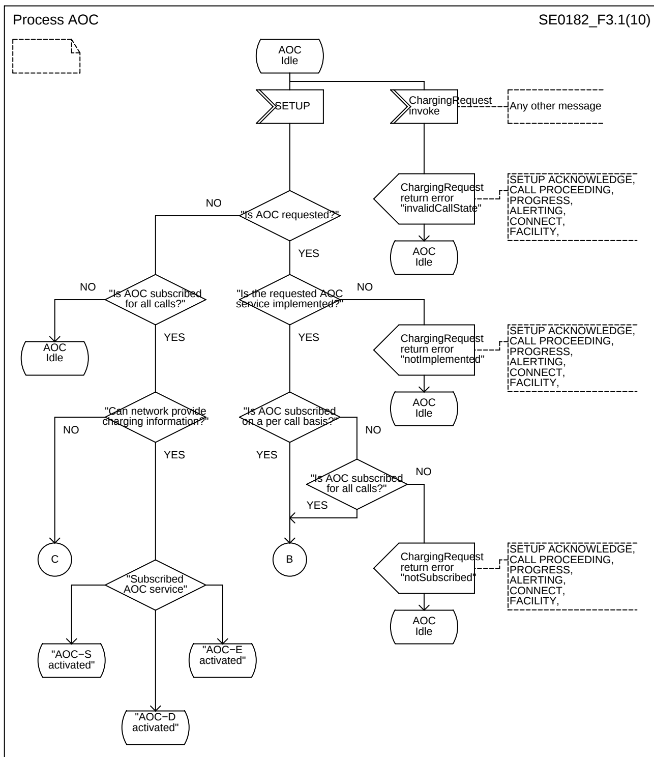
Figure 3 (sheet 1 of 2): Network side - AOC Idle
