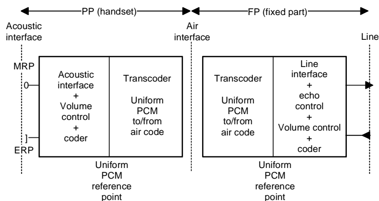
Figure 4.1: Basic reference configuration
