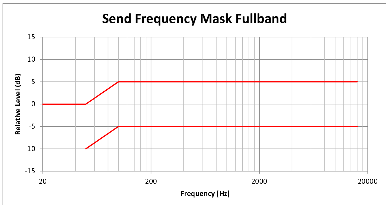
Figure 7.18f: Send frequency response mask for Fullband
