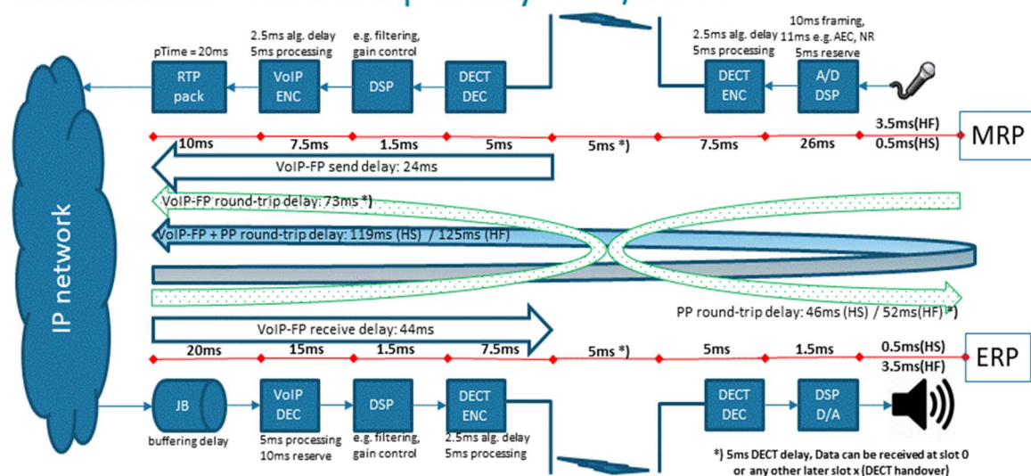
Figure F.1: Delay breakdown - PP and VoIP FP
