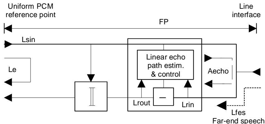
Figure A.5: Echo canceller implementation
