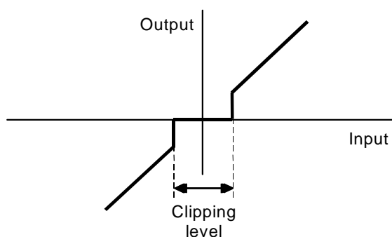
Figure A.2: Transfer function of non-linear processor
