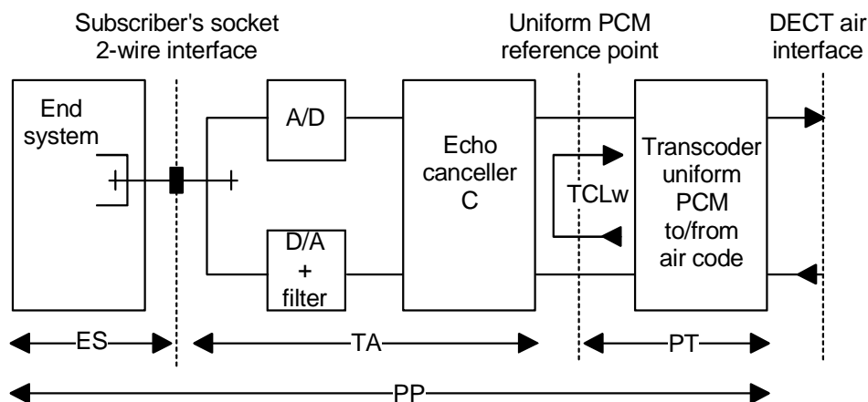
Figure B.1: PP in tethered local loop application
