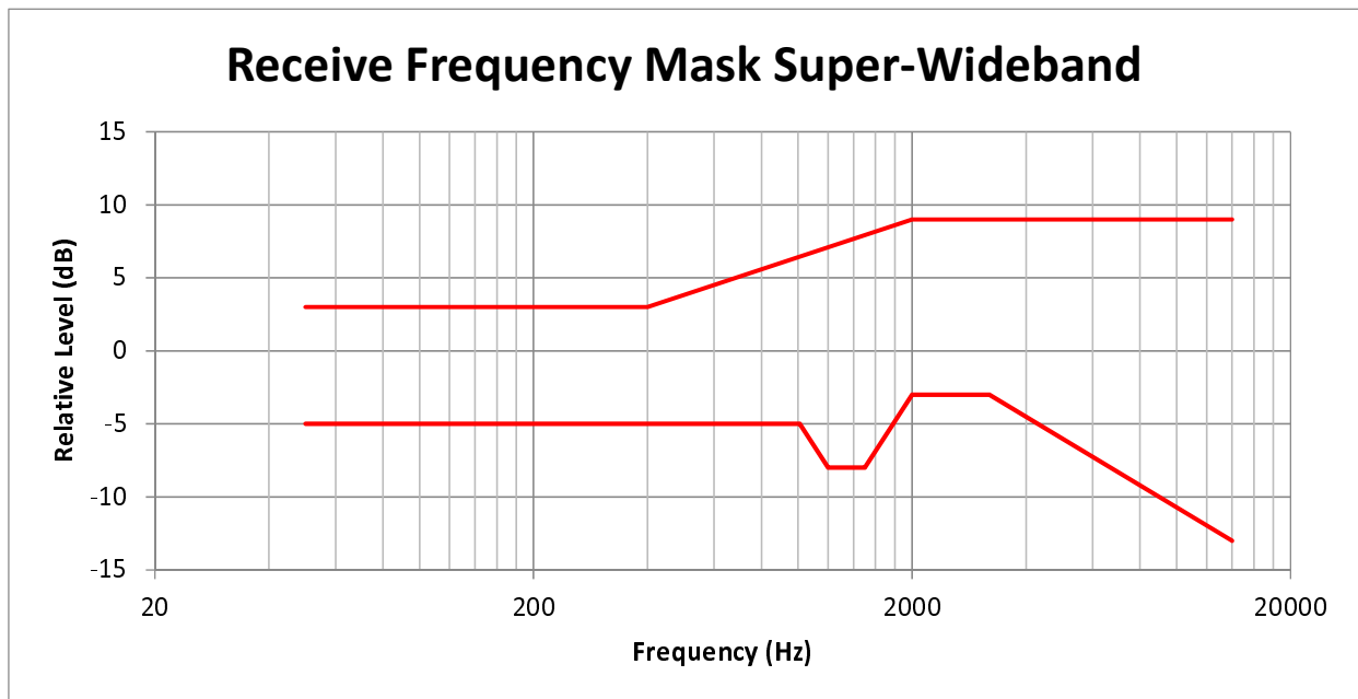
Figure 7.18b: Receive frequency response mask for super-wideband
