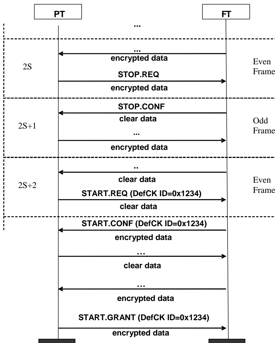
Figure 6.11a: Encryption change to a DefCK
