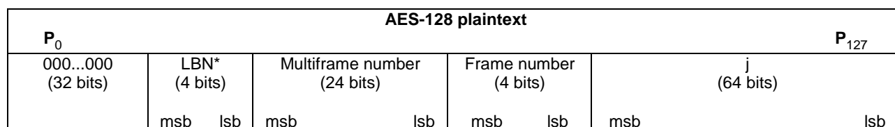
Figure M.1: Mapping of DECT values into AES-128 plaintext
