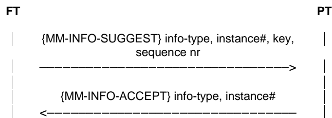
Figure 6.1a: FT parameter assignment procedure
