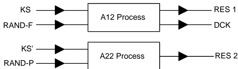
Figure 4.9: Derivation of RES1, DCK and RES2 for type 1 authentication
