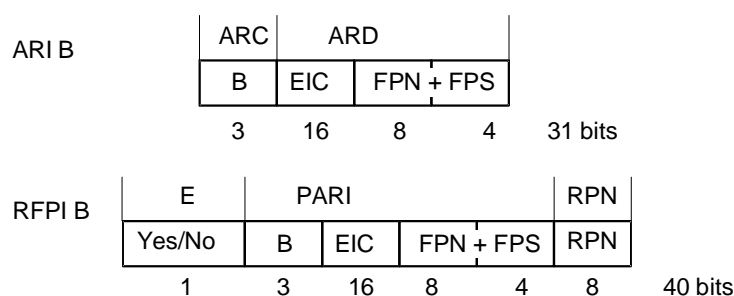
Figure 5.8: Access right class B, ARI, RFPI
