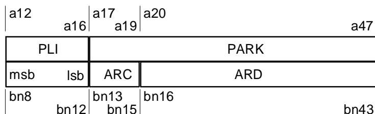
Figure 5.16: TARI PP request message
