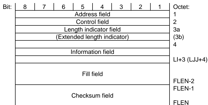
Figure 6.1.1: Frame format type FA
