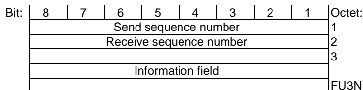
Figure 12.4.1.1: Frame format type FU3a
