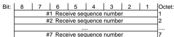
Figure 12.5.1.2: Frame format type FU4b
