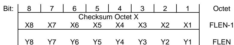
Figure 7.9.1: Checksum field format
