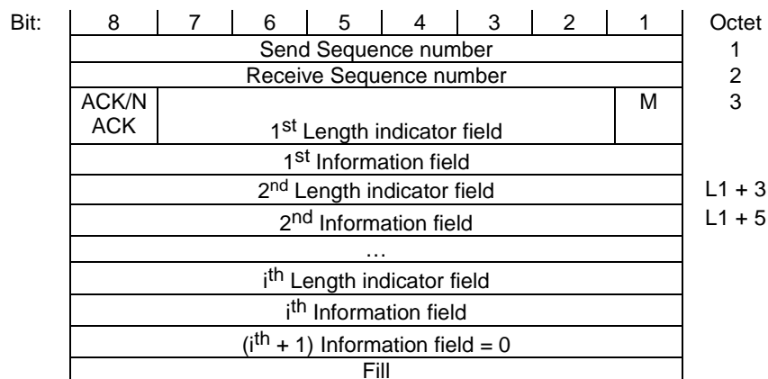
Figure 12.11.1.2: Frame format type FU10b
