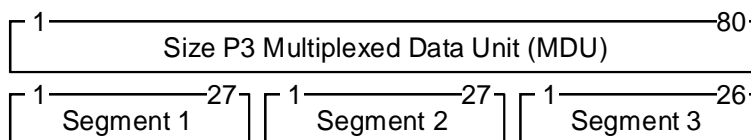
Figure 11.6.2.4.1: Segmentation of Size P3 MDU
