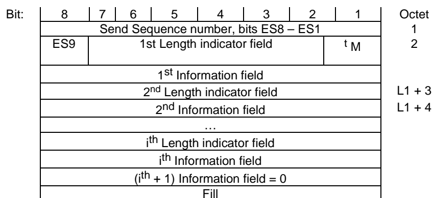
Figure 12.11.1.1: Frame format type FU10a
