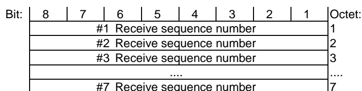
Figure 12.7.1.2: Frame format type FU6b
