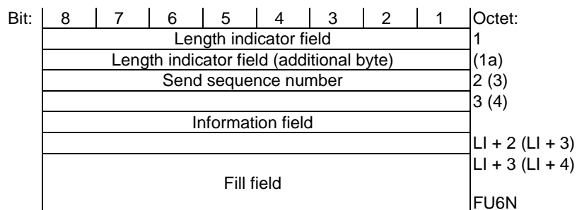
Figure 12.7.1.1: Frame format type FU6a
