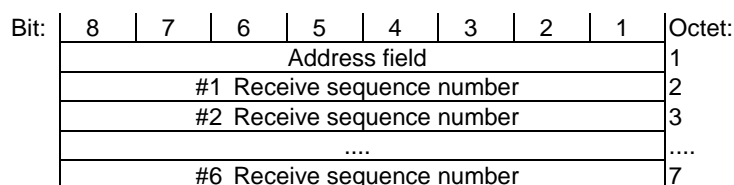
Figure 12.6.1.2: Frame format type FU5b
