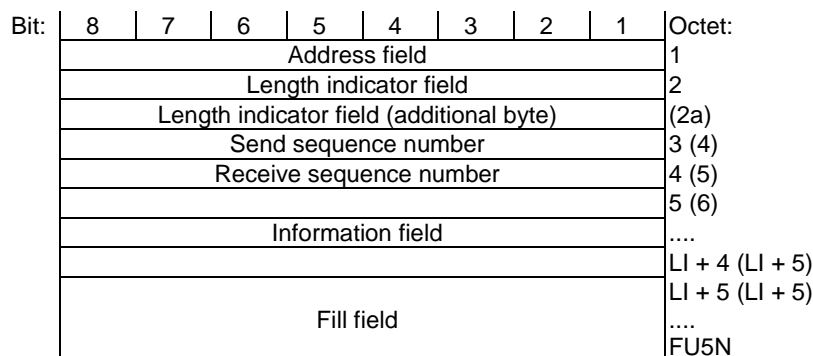
Figure 12.6.1.1: Frame format type FU5a
