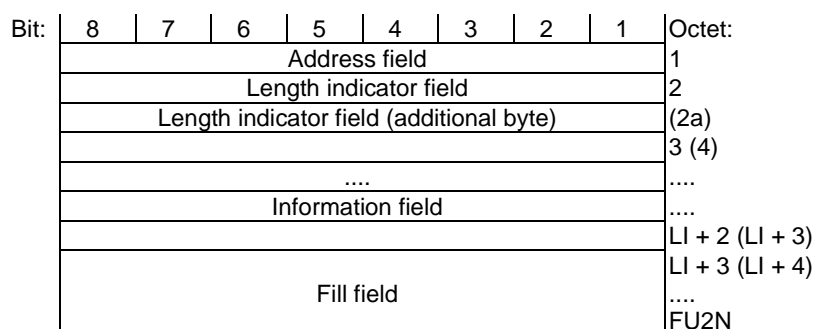
Figure 12.3.1.1: Frame Format Type FU2
