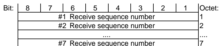
Figure 12.4.1.2: Frame format type FU3b
