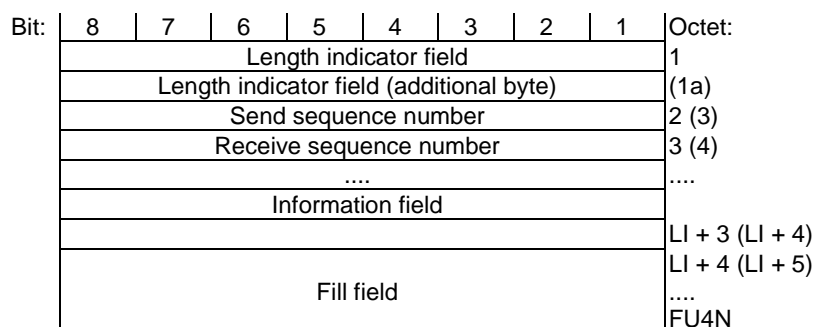
Figure 12.5.1.1: Frame format type FU4a
