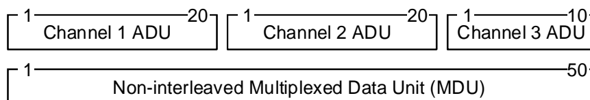
Figure 11.6.2.3.1: Example of non-interleaved packing (MCS Ref: P2/16)
