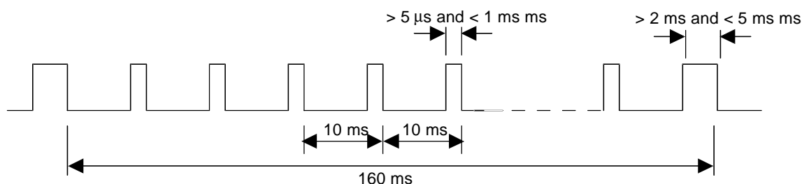
Figure B.3: Synchronization signal timing
