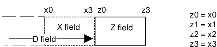
Figure 18: The Z-field
