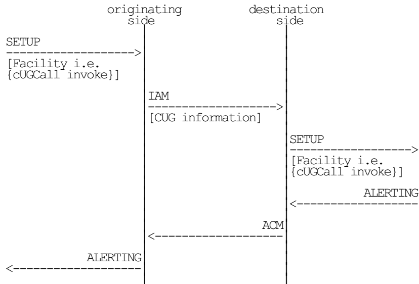
Figure A.1: Call passes both originating and destination network side checks and is successful in the destination user's side
