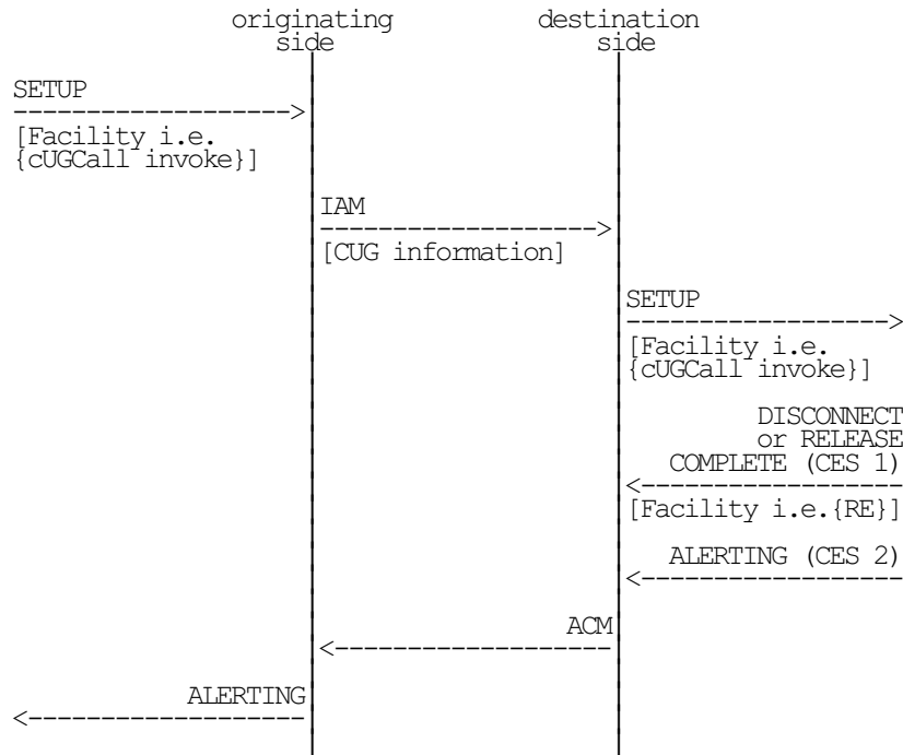
Figure A.3: Call passes both originating and destination network side checks, with point-to-multipoint configuration at destination user's side
