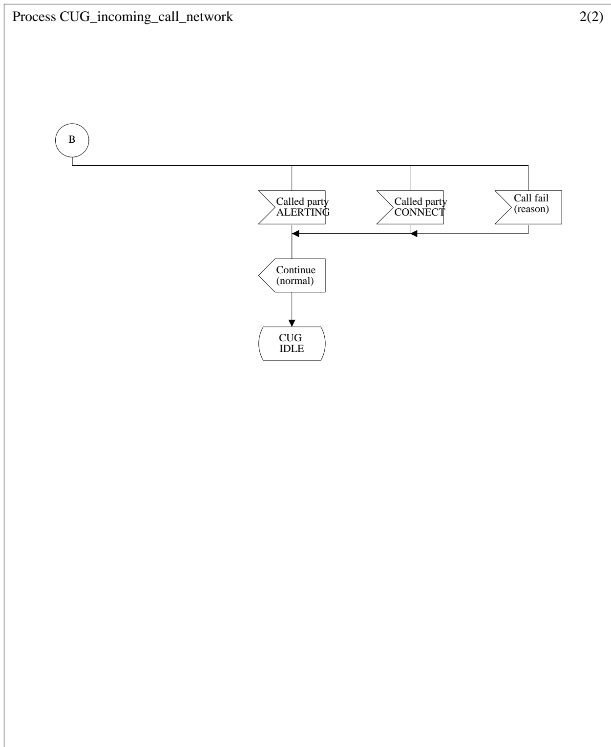
Figure 2 (sheet 2 of 2): CUG process - incoming call (network side)
