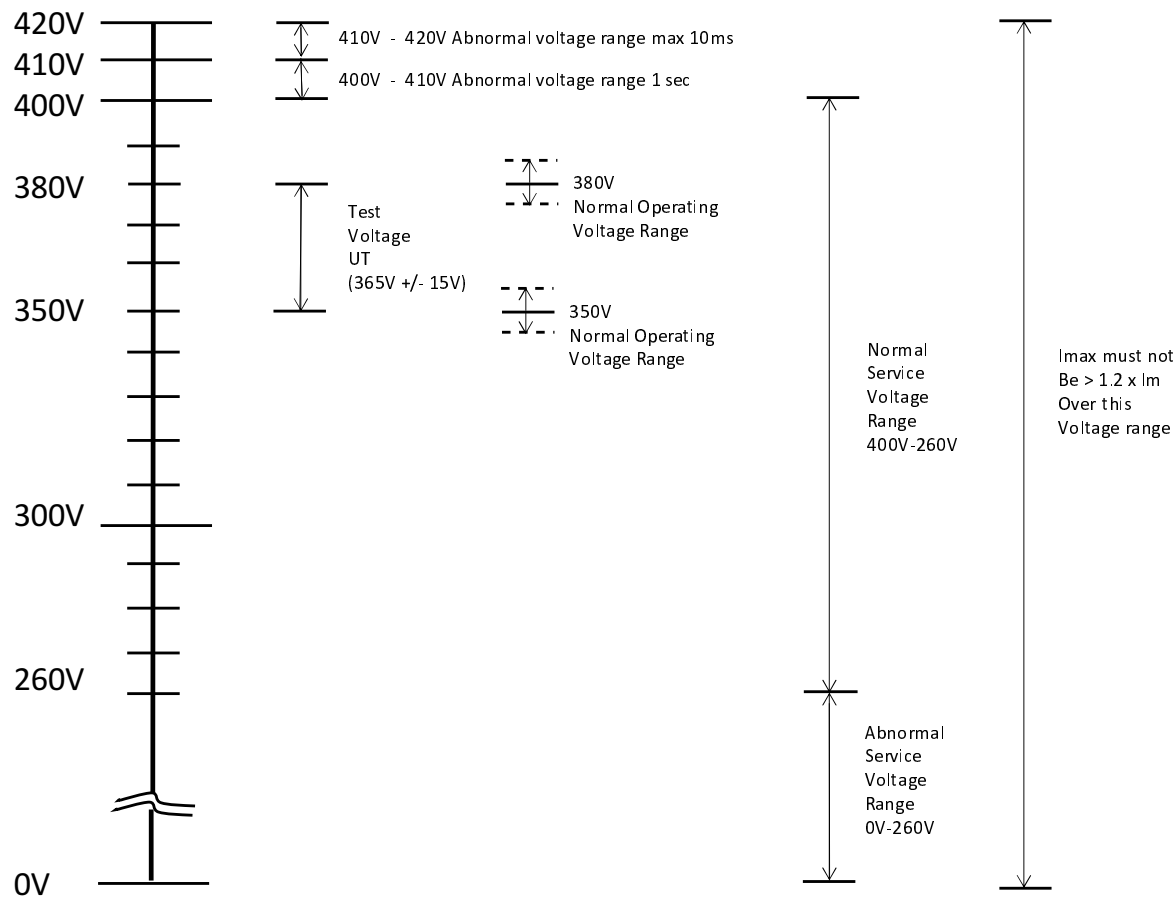
Figure G.1: Diagram of DC voltage ranges and values at the interface "A3"
