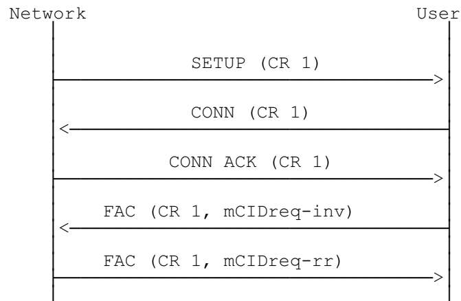
Figure A.1: Successful MCID supplementary service invocation during the Active state (N10, U10)
