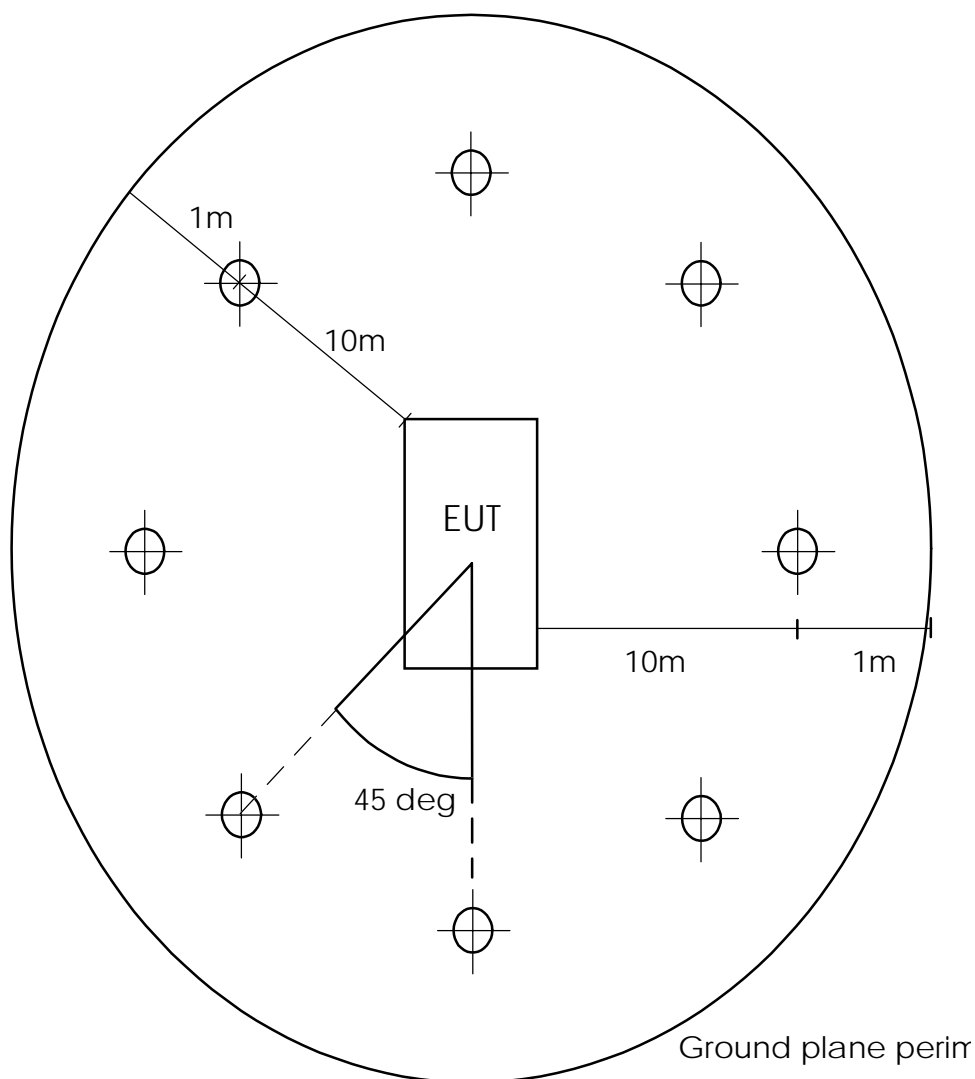
Figure 5: Example of an 8 radial position measurement site
