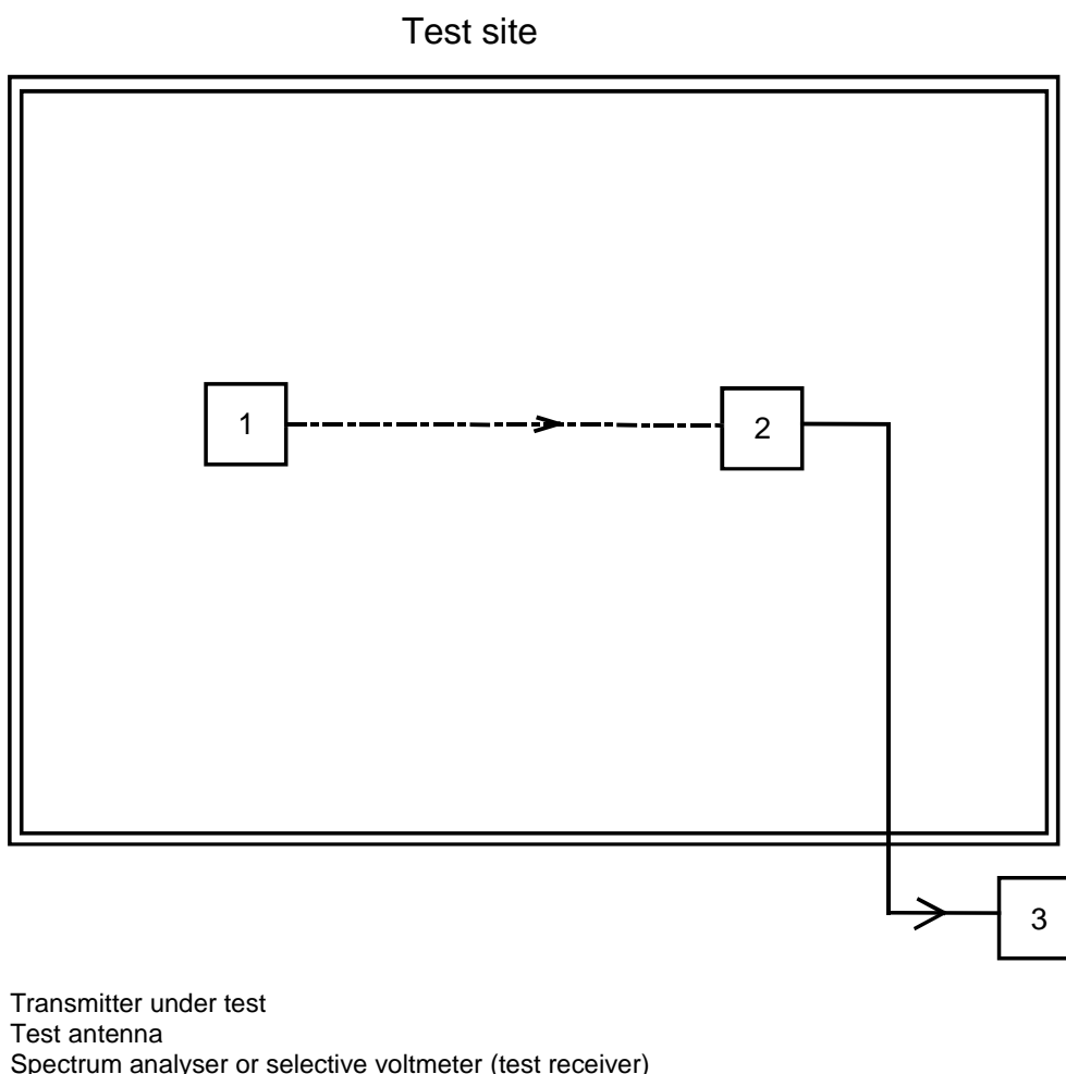
Figure 9: Measurement arrangement
