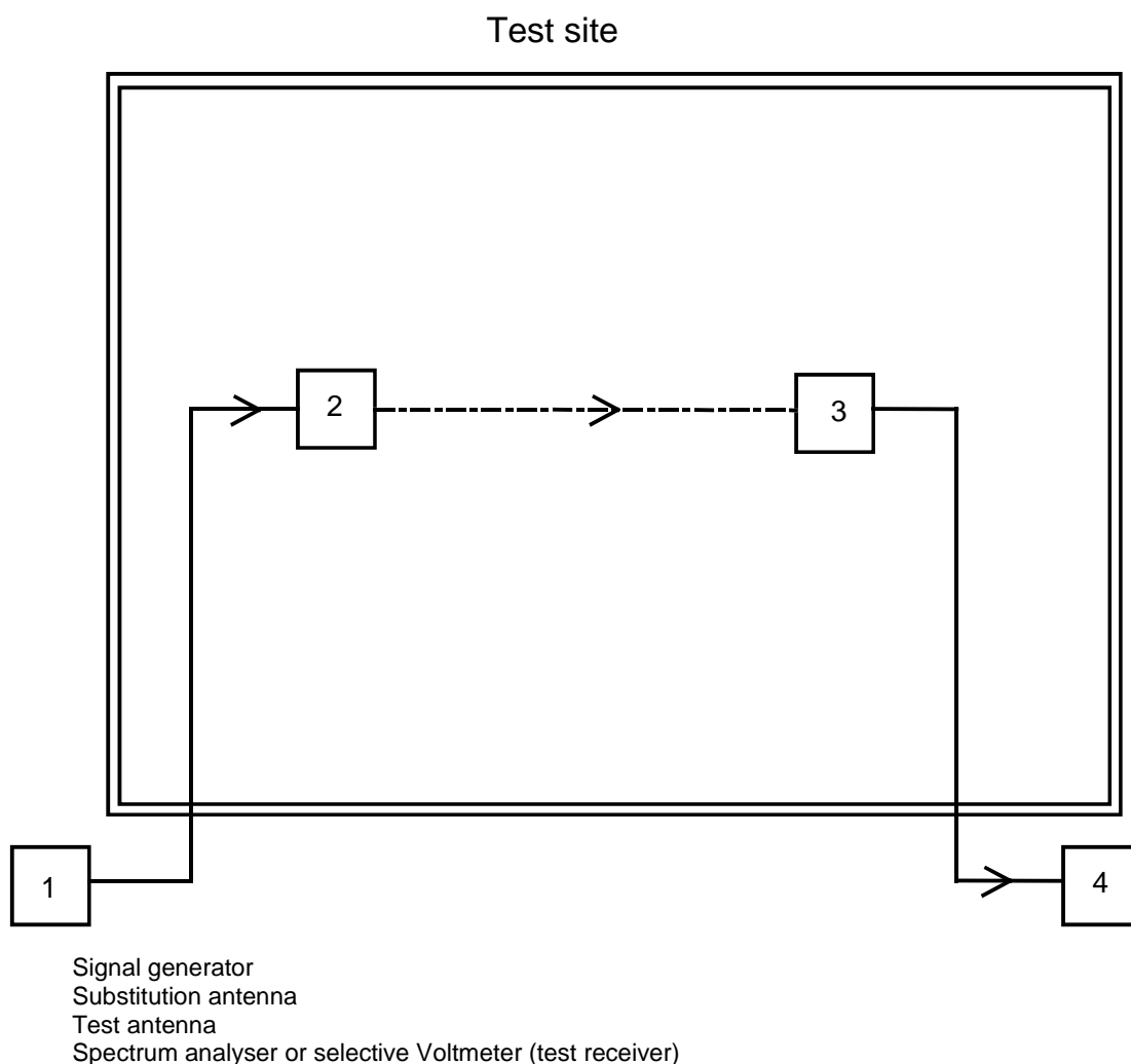
Figure 10: Measurement arrangement
