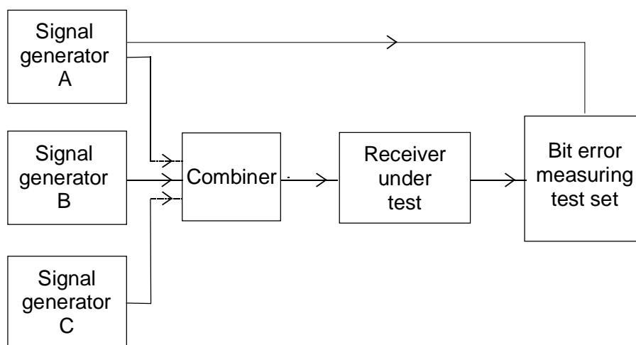
Figure 26: Measurement arrangement
