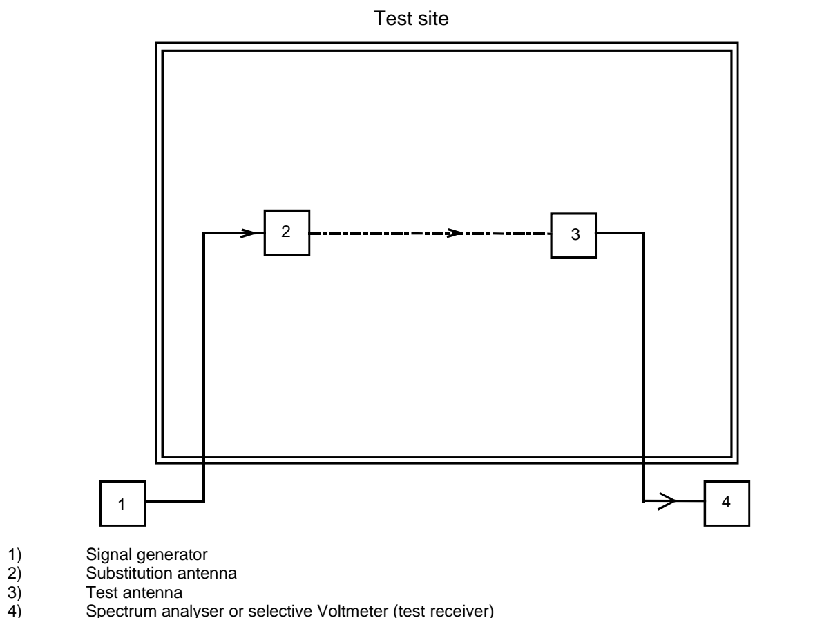
Figure 6: Measurement arrangement
