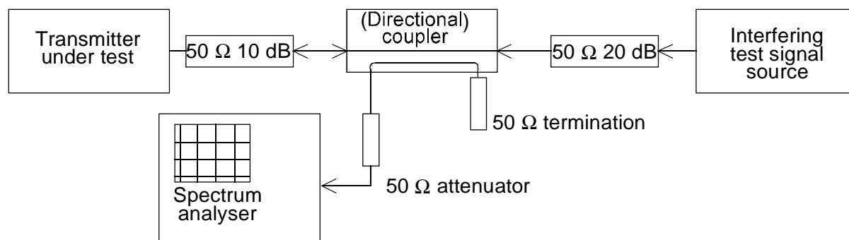
Figure 11: Measurement arrangement
