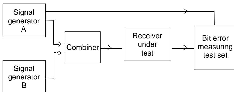
Figure 21: Measurement arrangement
