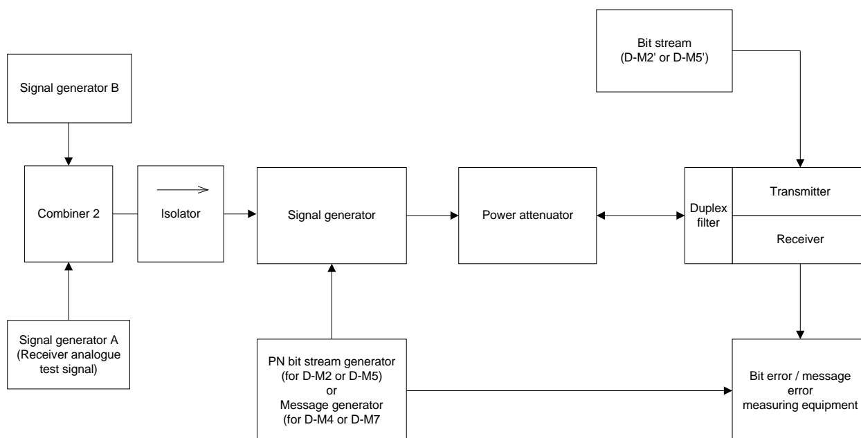
Figure 35: Measurement arrangement for equipment with a Duplex filter
