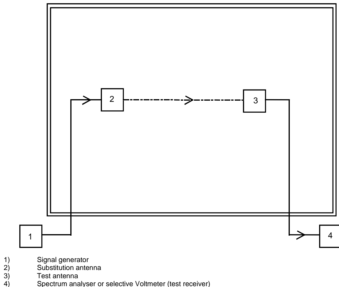
Figure 10: Measurement arrangement
