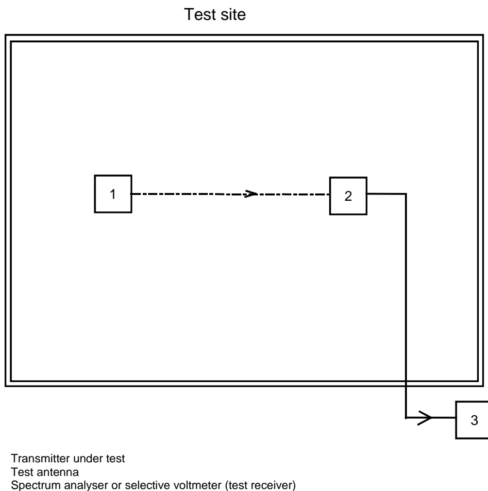
Figure 9: Measurement arrangement
