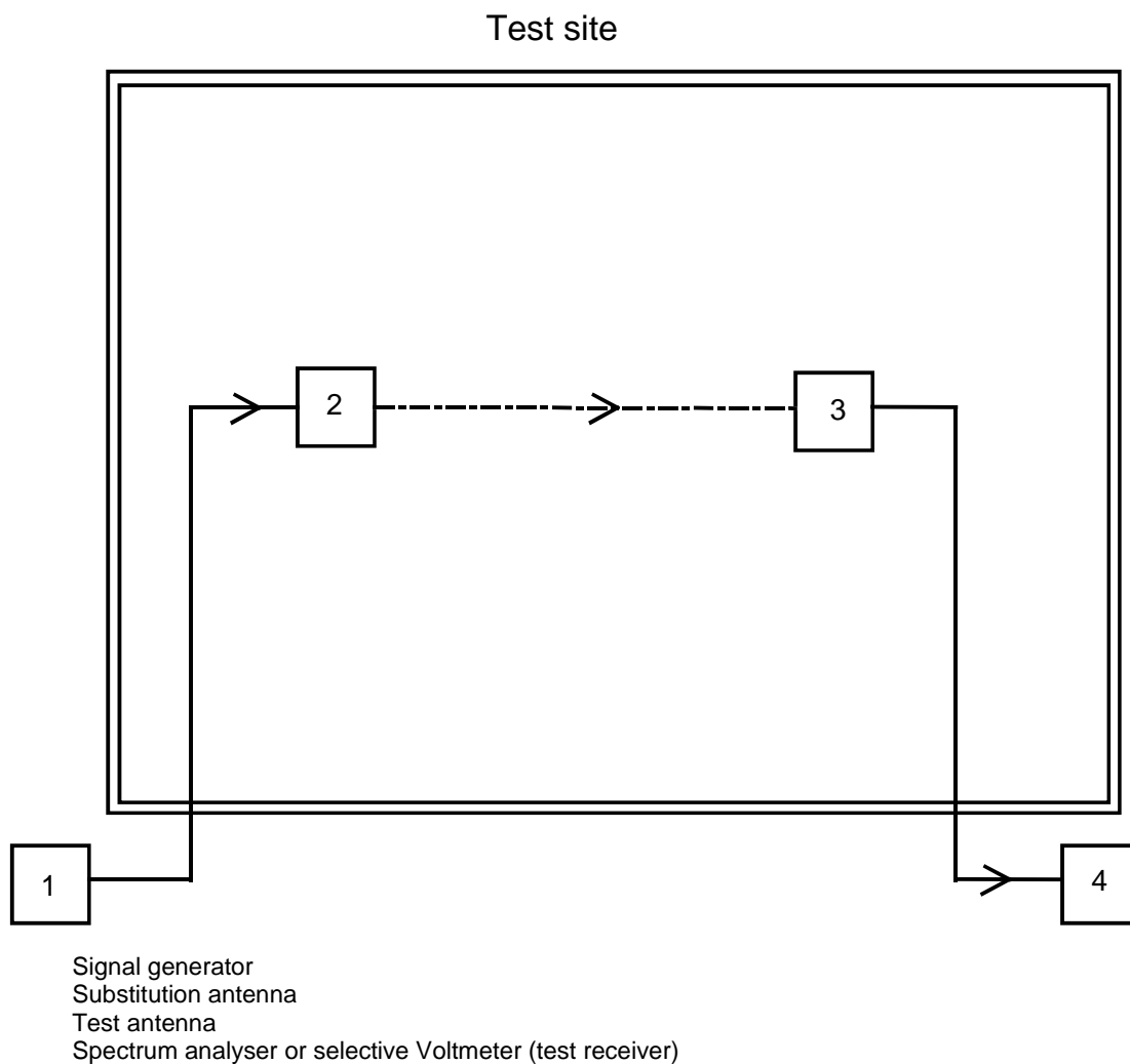
Figure 32: Measurement arrangement
