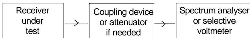
Figure 30: Measurement arrangement
