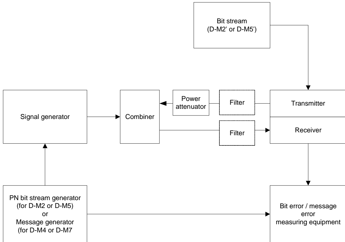
Figure 34: Measurement arrangement
