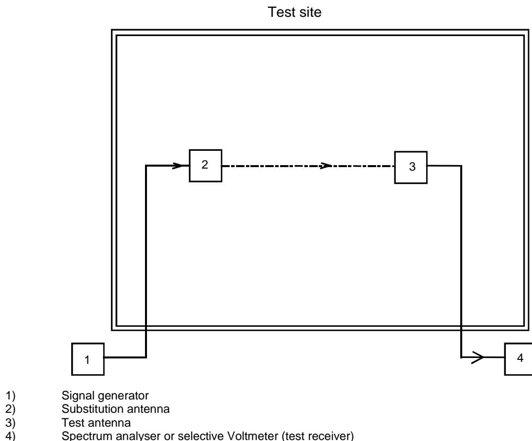
Figure 6: Measurement arrangement
