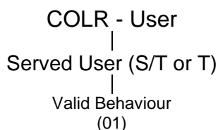
Figure 1: Test suite structure
